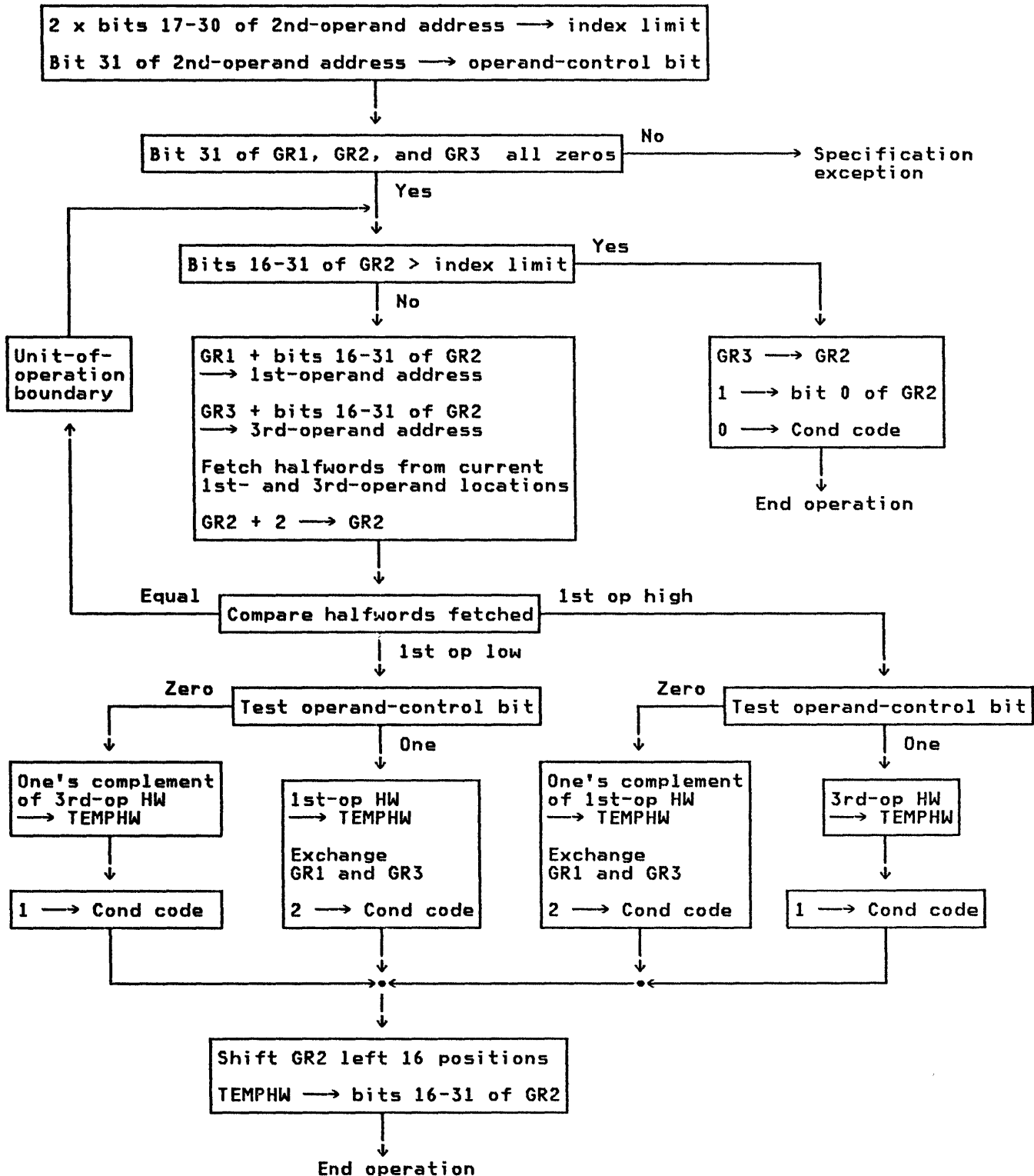
Execution of COMPARE AND FORM CODEWORD
