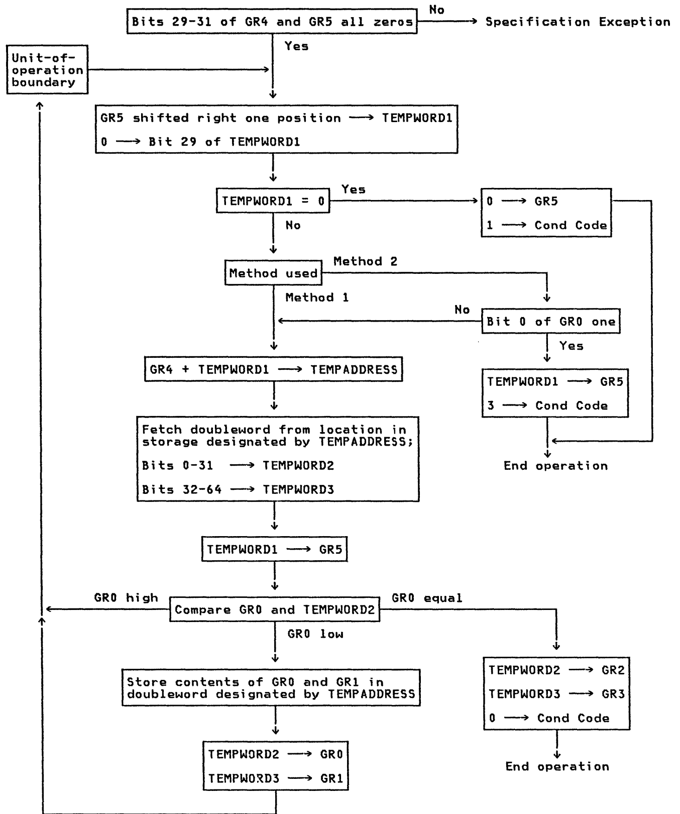
Execution of UPDATE TREE
