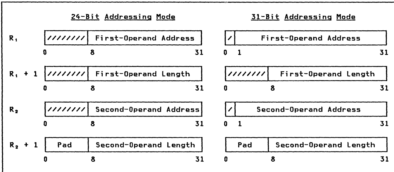
Register Contents for MOVE LONG
