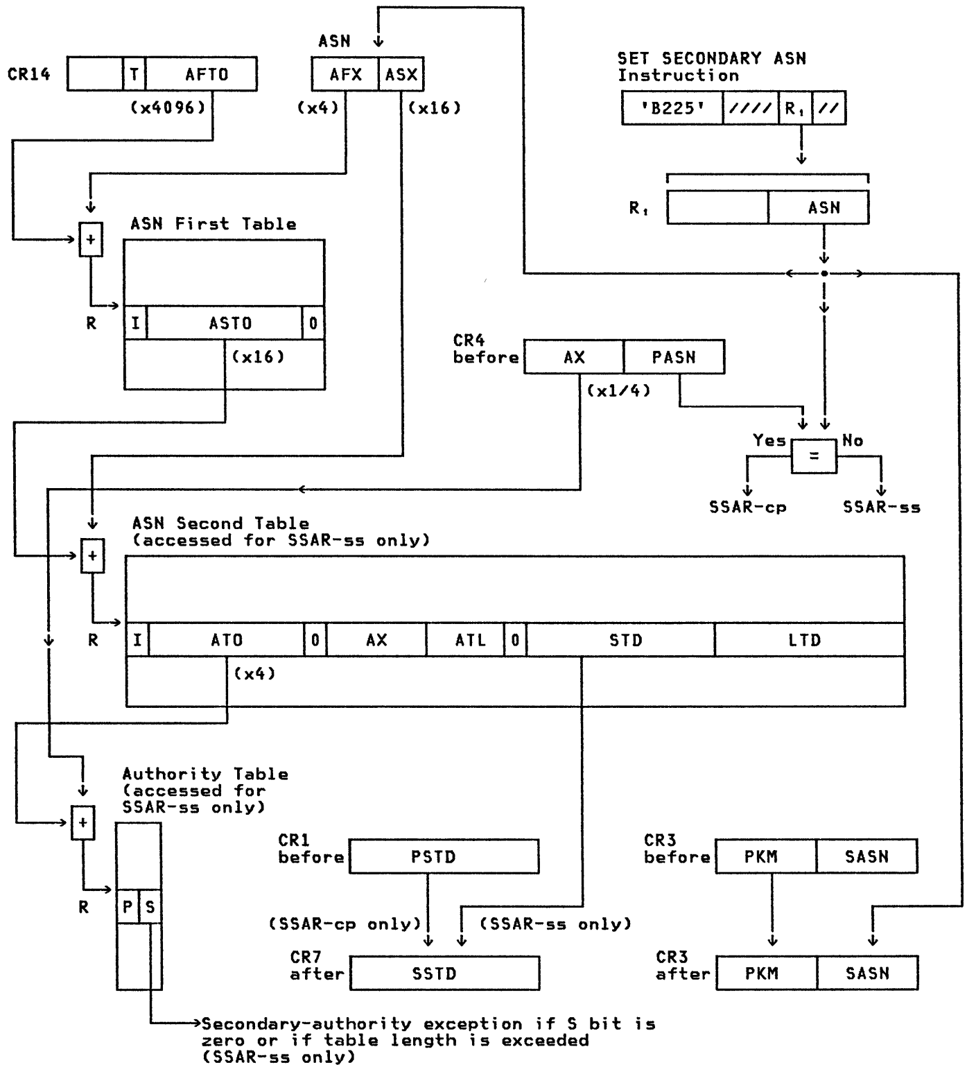
Execution of SET SECONDARY ASN
