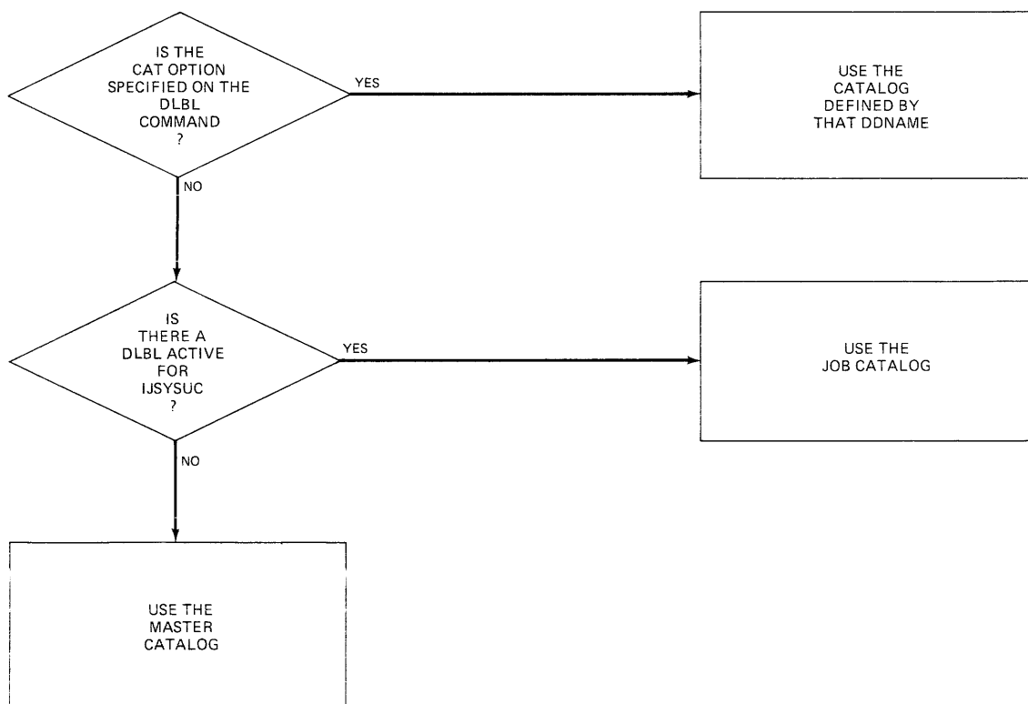
Figure 7. Determining Which VSAM Catalog to Use
