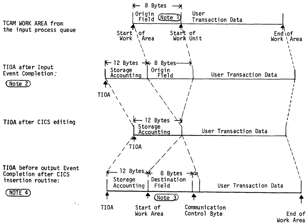
Figure 14. Stages of the TCAM work area and CICS terminal input/output area (TIOA)
