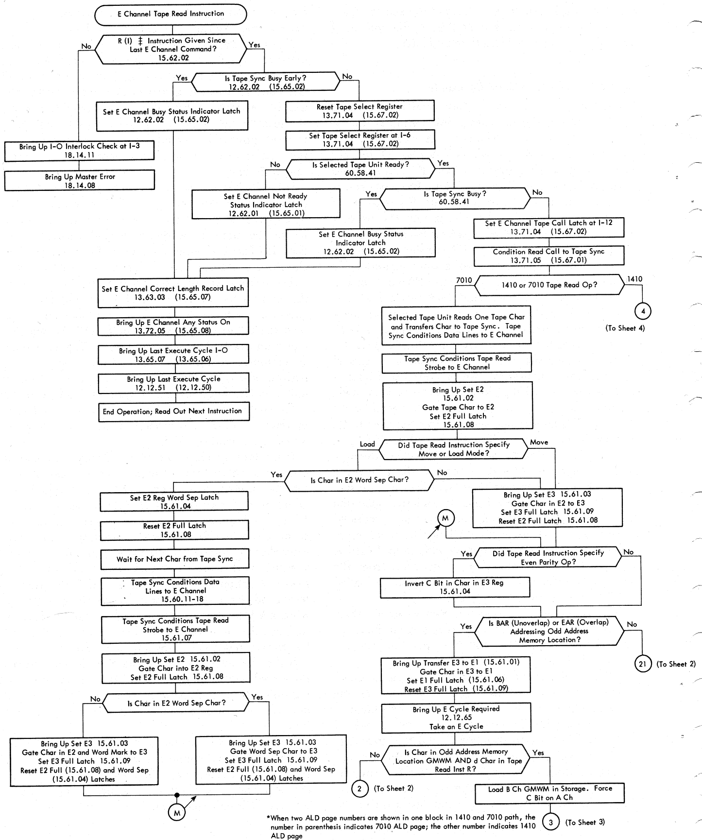
Figure 15. E-Channel Tape Read Operation (Sheet 1 of 5)
