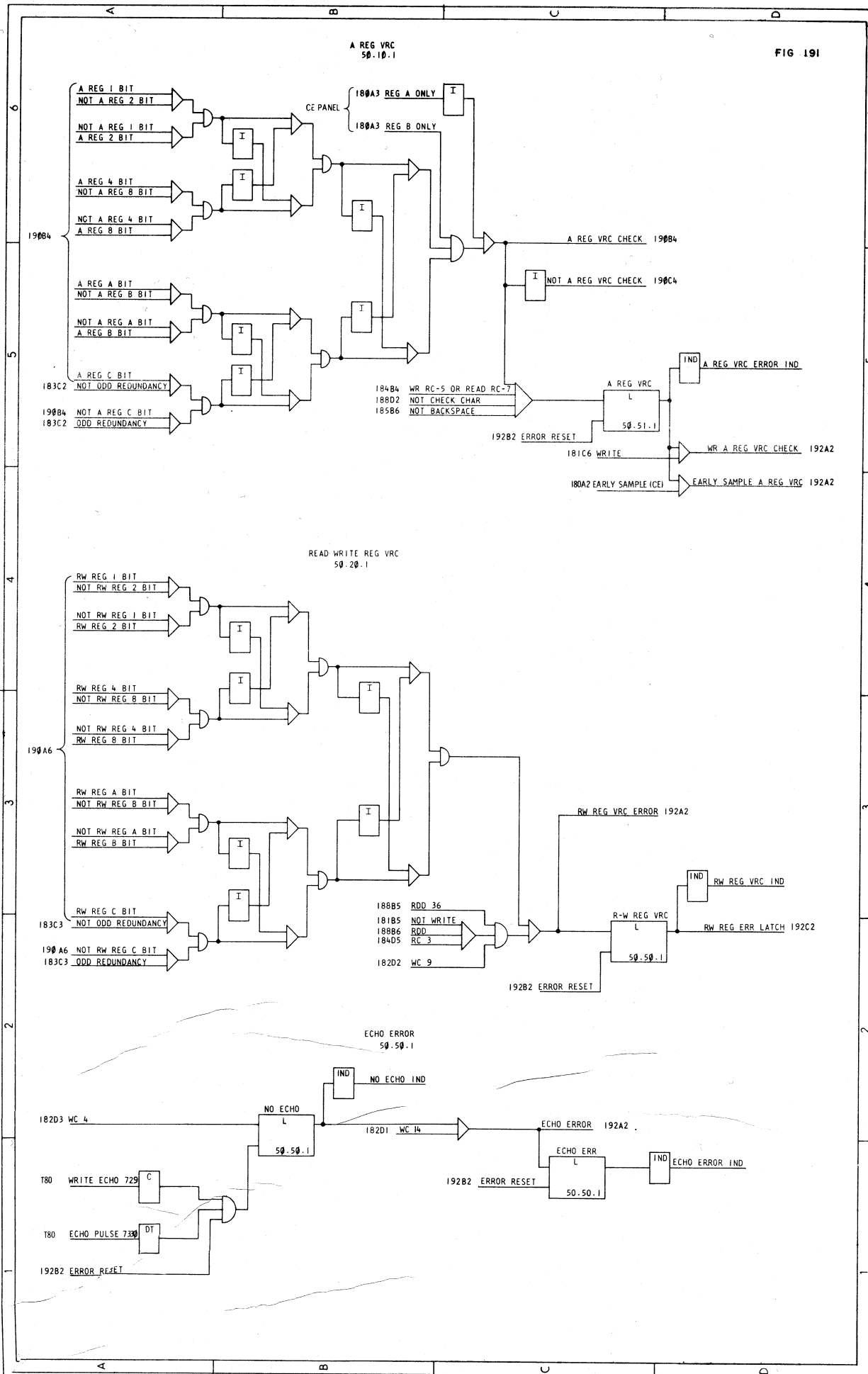
Figure 191. Error Circuits I
