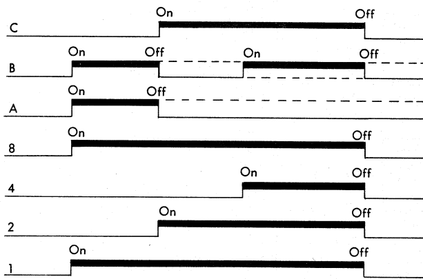
Figure 21. LRCR Check
