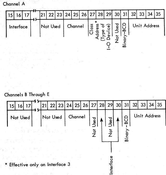
Figure 8. Breakdown of Address Part of Select Instruction
