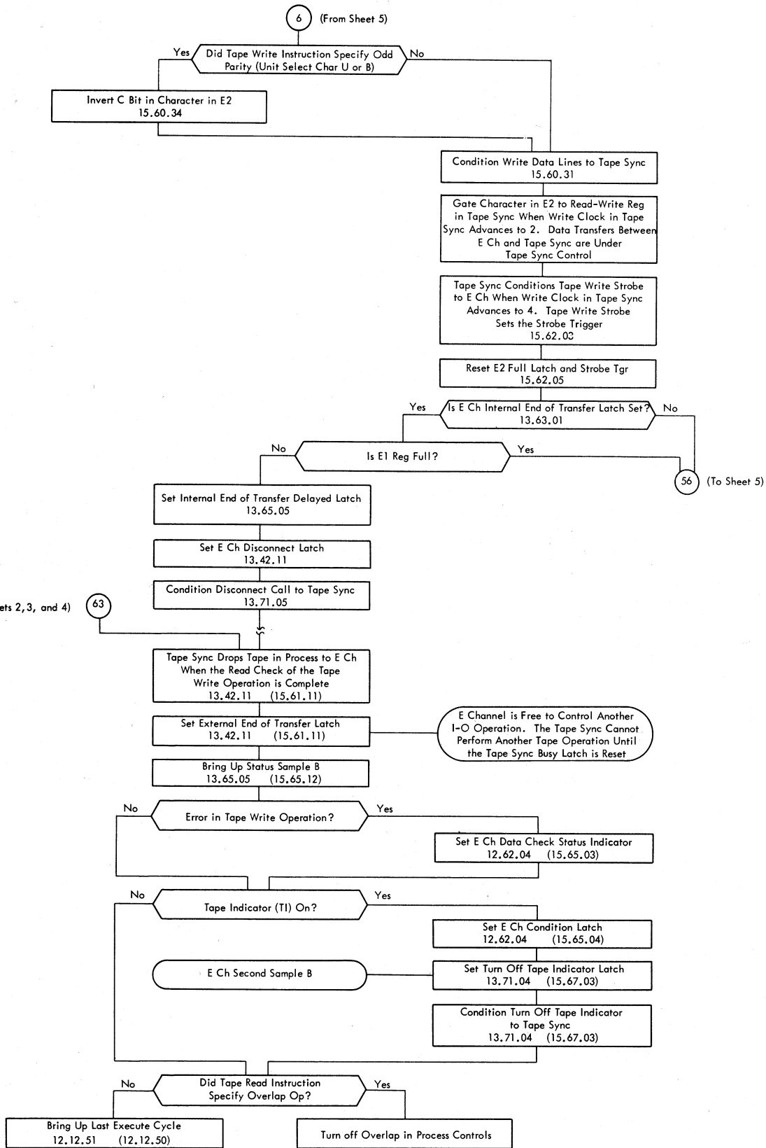
Figure 14. E-Channel Tape Write Operation (Sheet 6 of 6)
