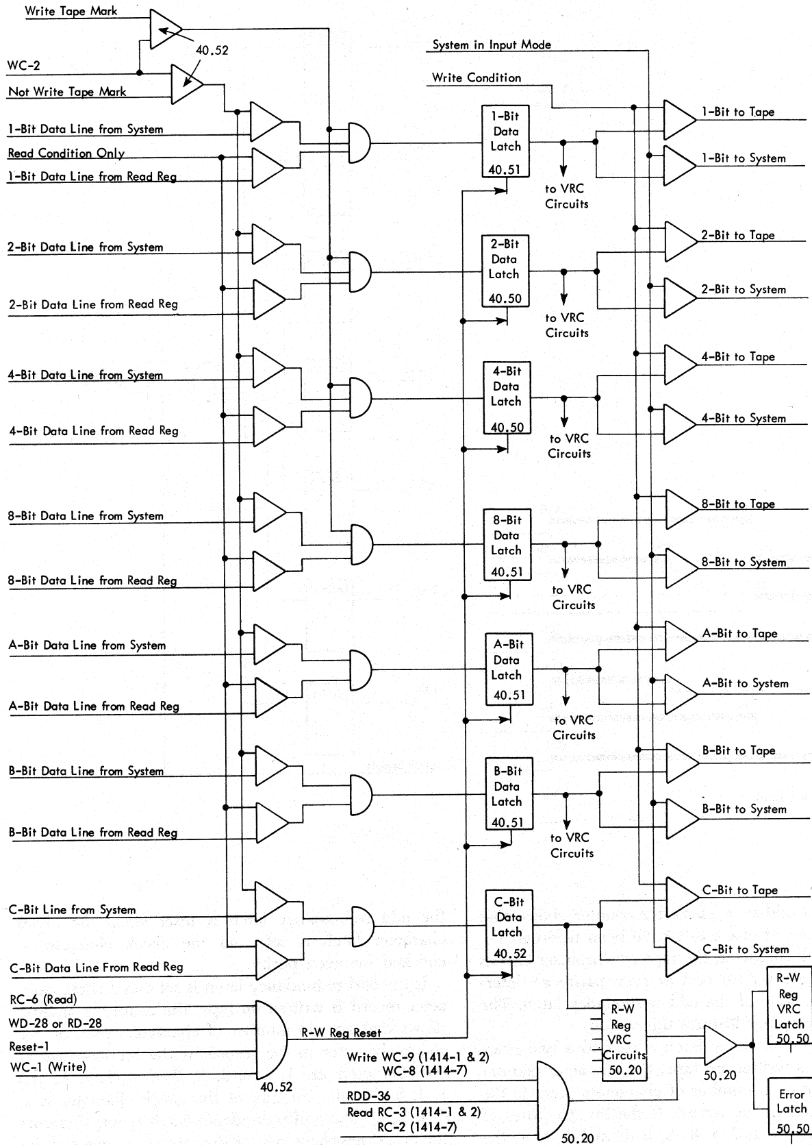
Figure 20. Read-Write Register
