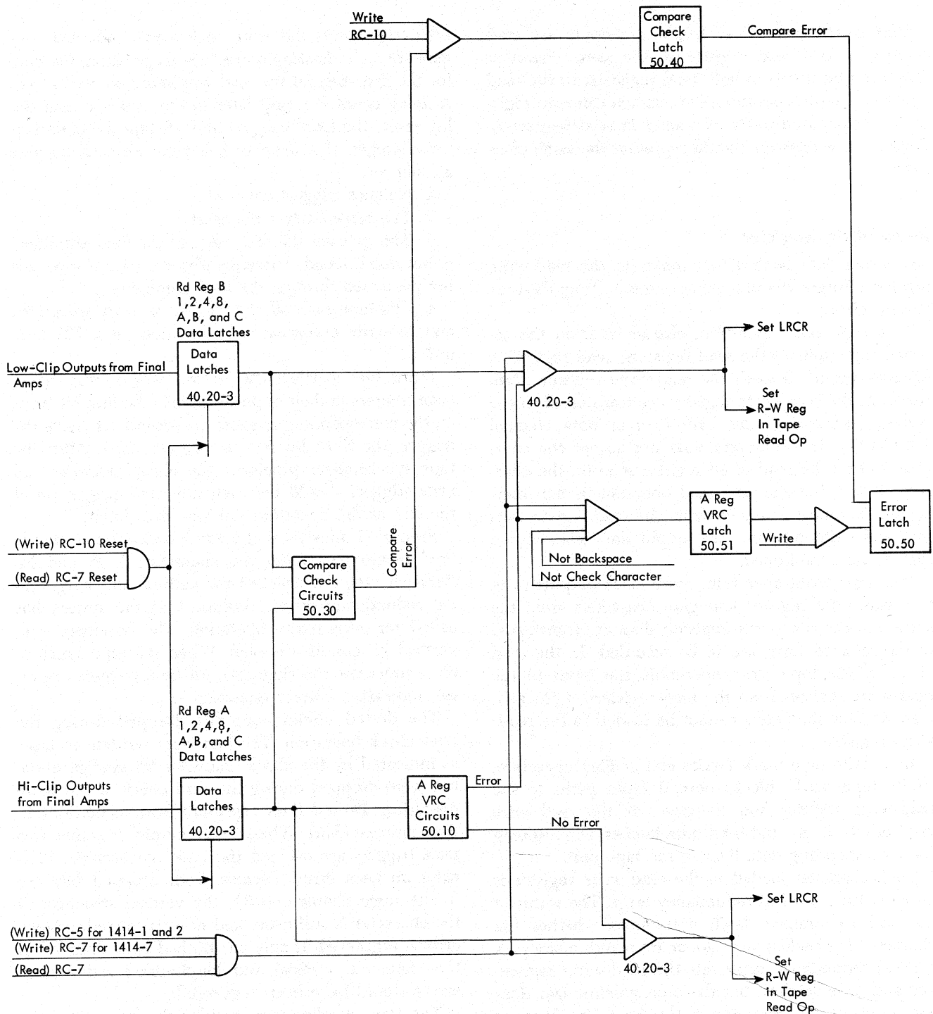
Figure 19. Read Registers
