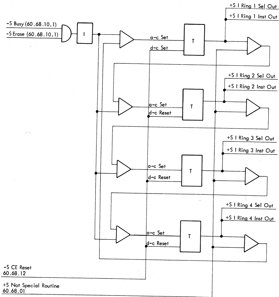
Figure 46. Instruction Ring
