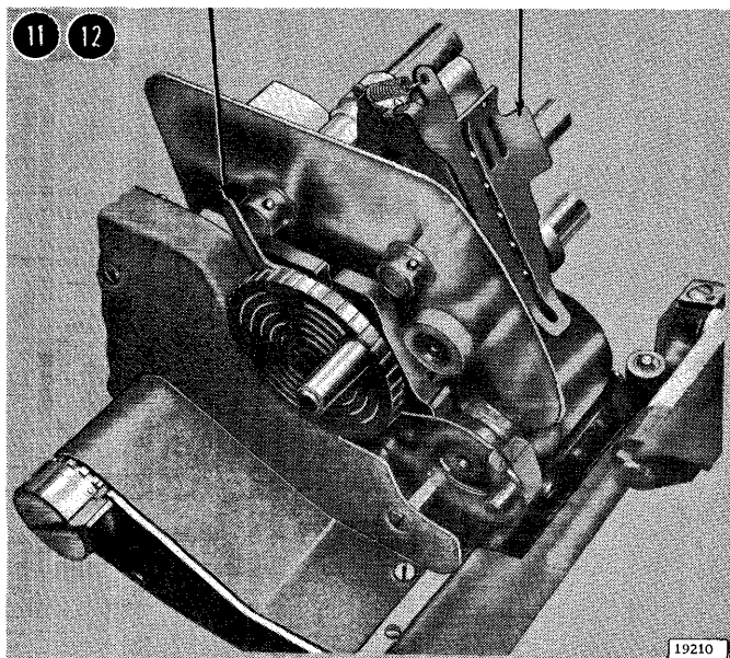
Platen Pressure Roll Release Lever Left Hinged Pressure Plate
