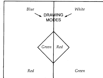
Mode 6-Complement 2
