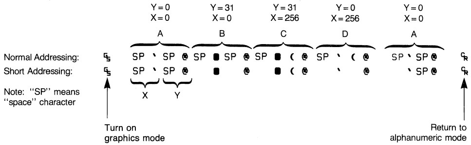
Figure 3-20. Computer to Terminal Addressing
