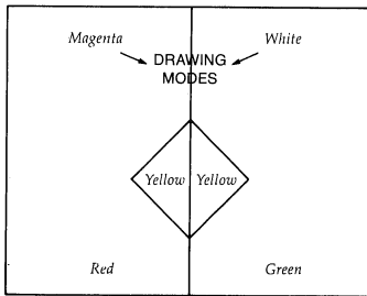
Mode 5-OR
