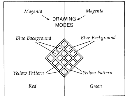
Mode 4-Jam 2
