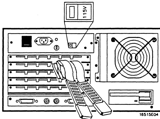
Figure 1-3. Selecting the proper line voltage
