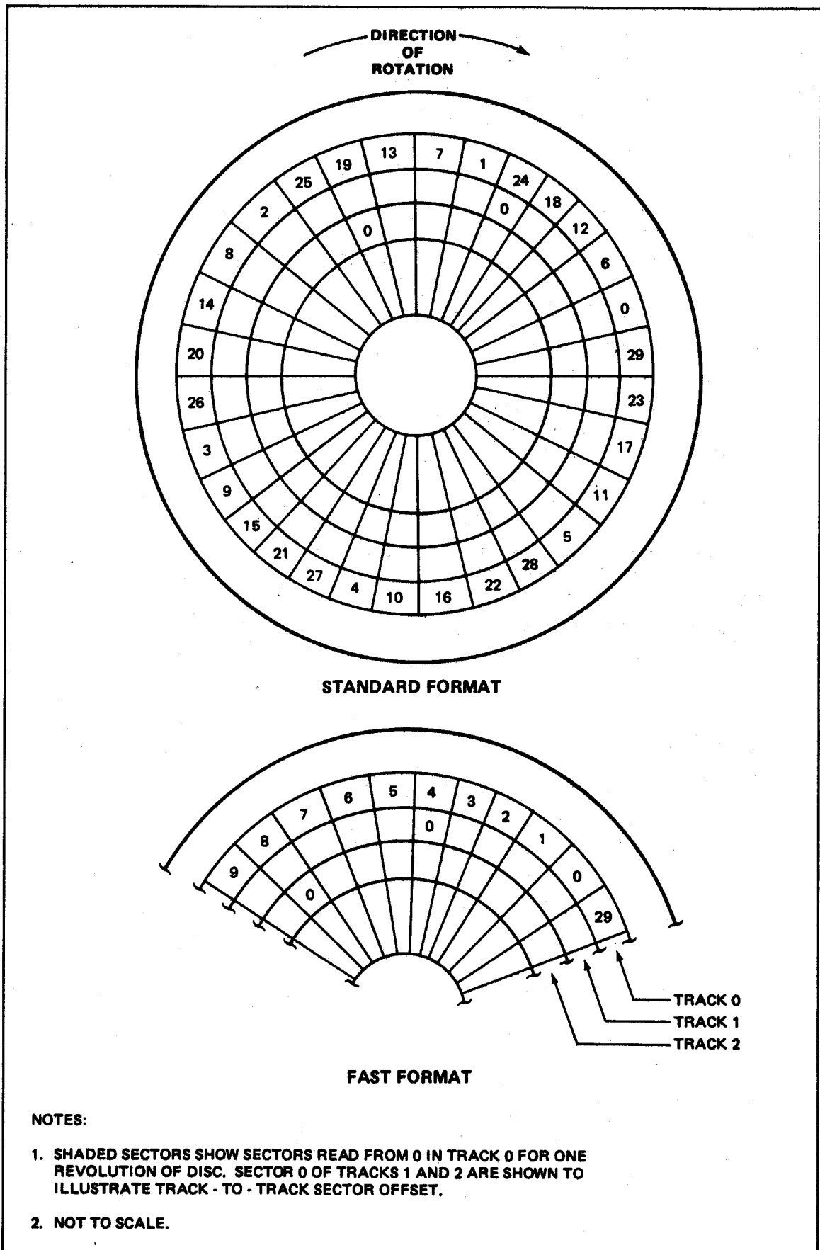
Figure B-1. Flexible Disc Formats
