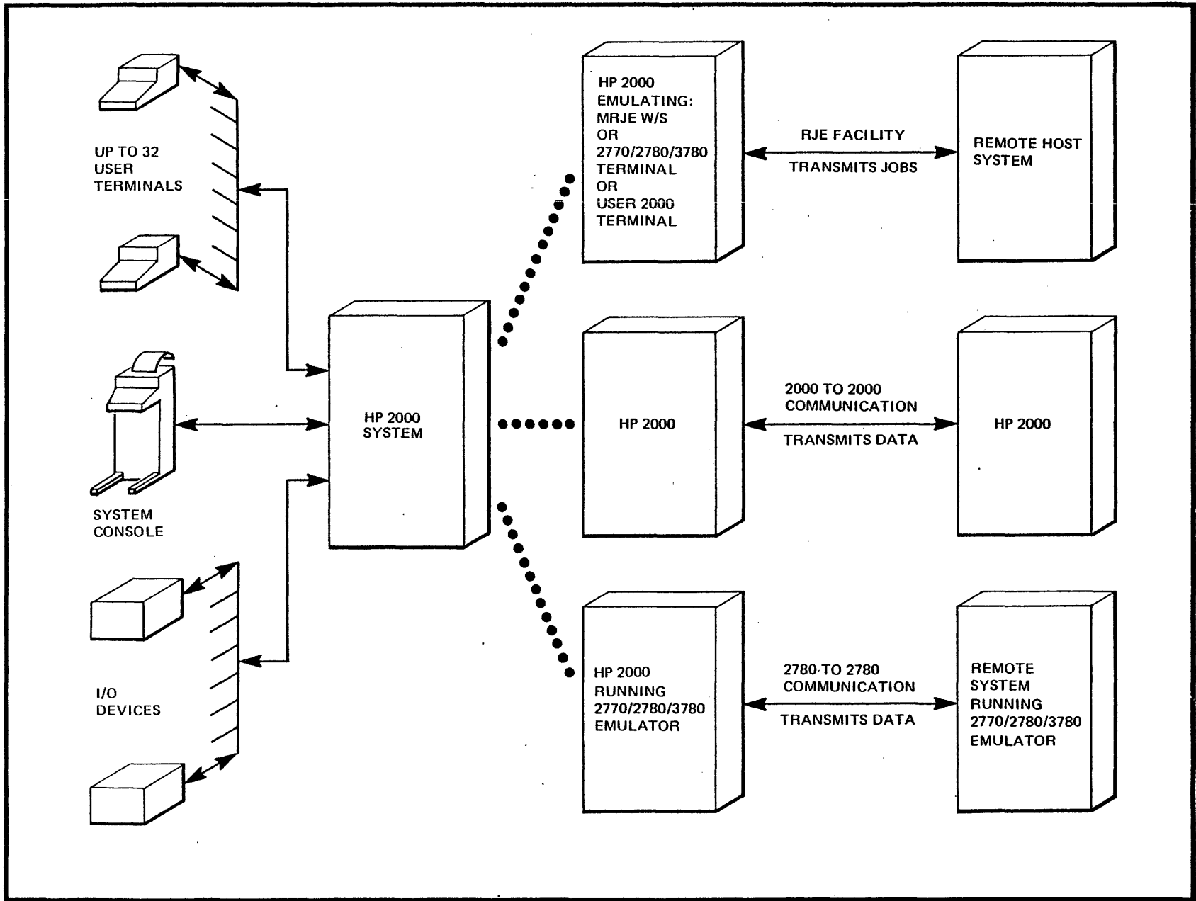
Figure 6-1. Elements of an HP 2000 Data Communications Facility
