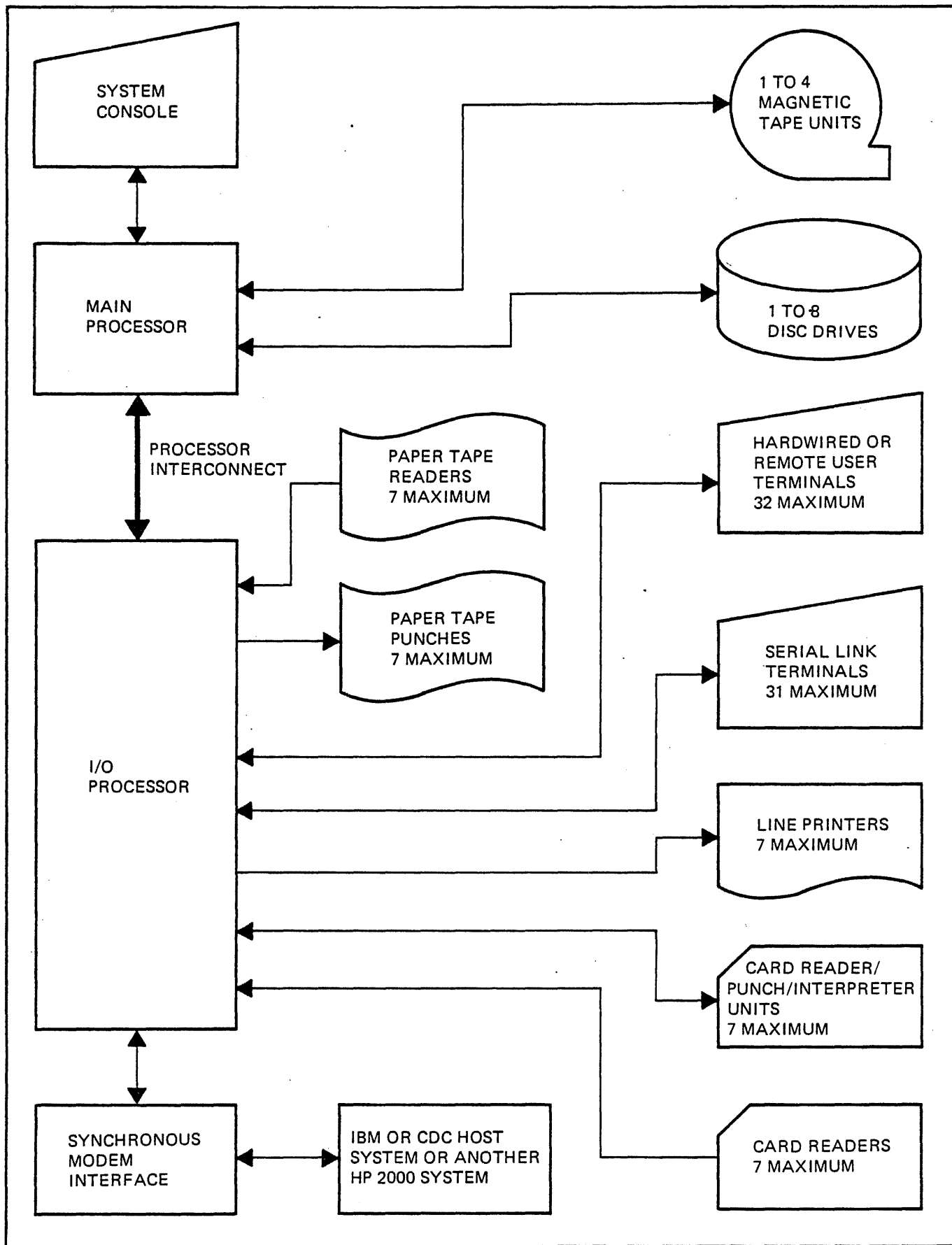
Figure 1-1. HP 2000 Computer System Organization
