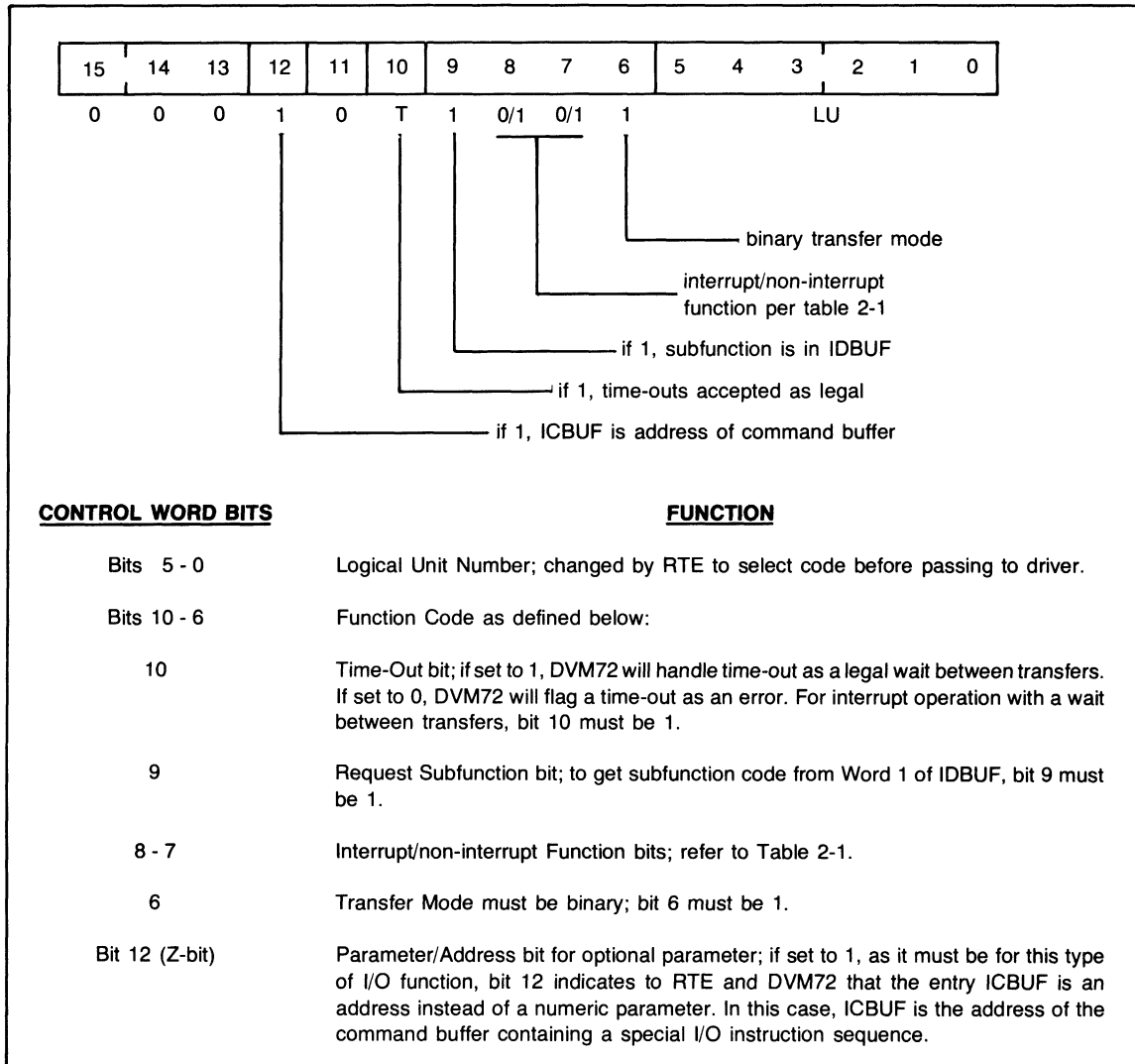
Figure 2-6. Control Word Format, Special Read/Write Requests
