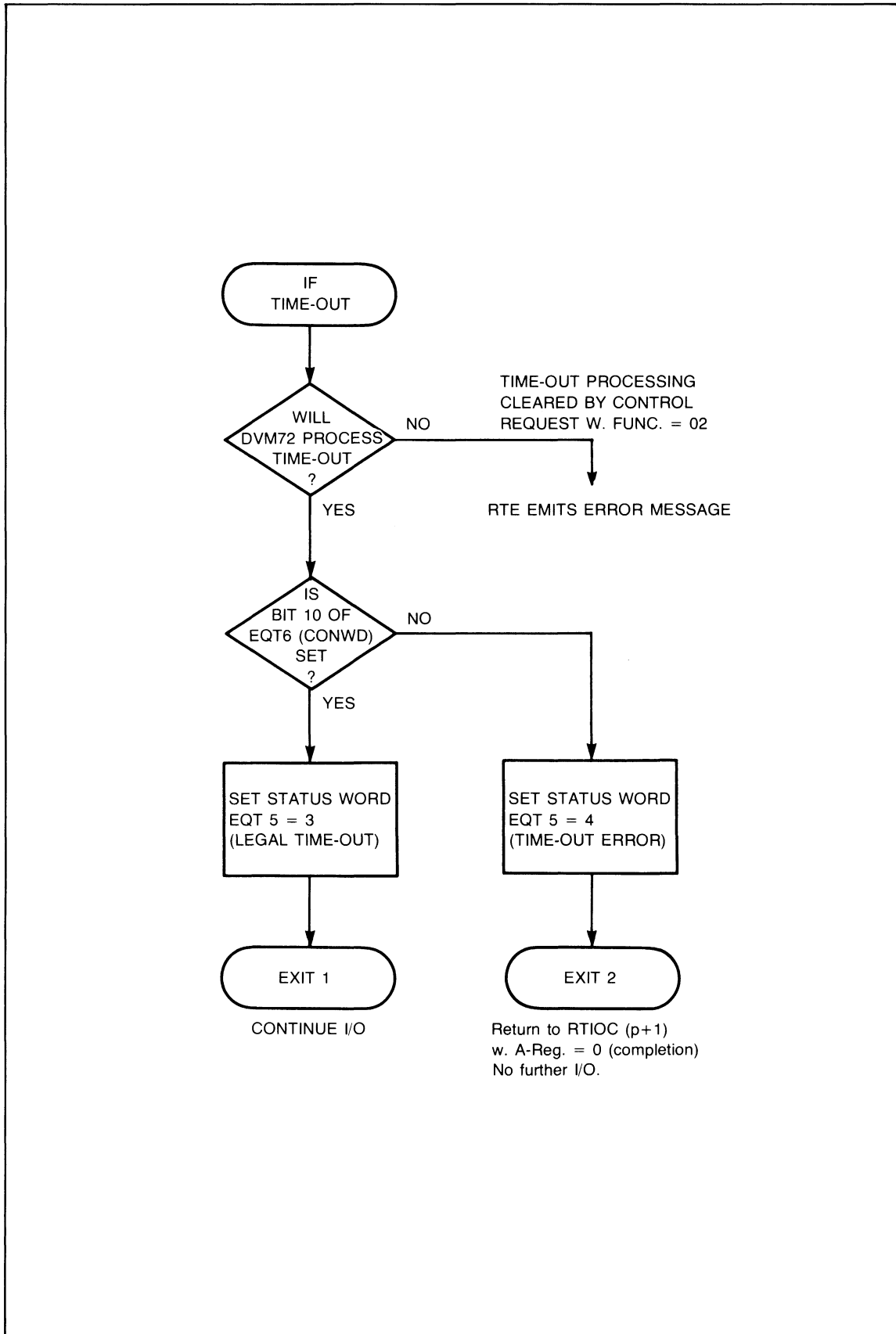
Figure 2-2. DVM72 Time-Out Processing
