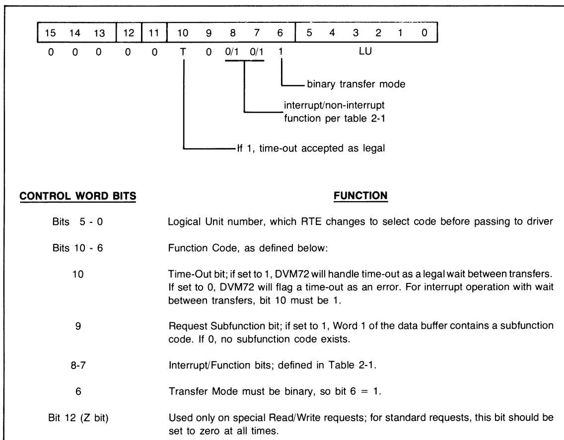
Figure 2-3. Control Word Format, Standard Read/Write Requests
