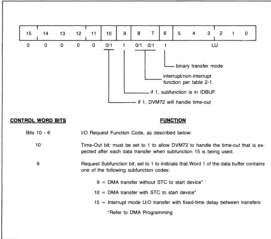
Figure 2-4. Control Word Format, Read/Write Requests with Subfunction
