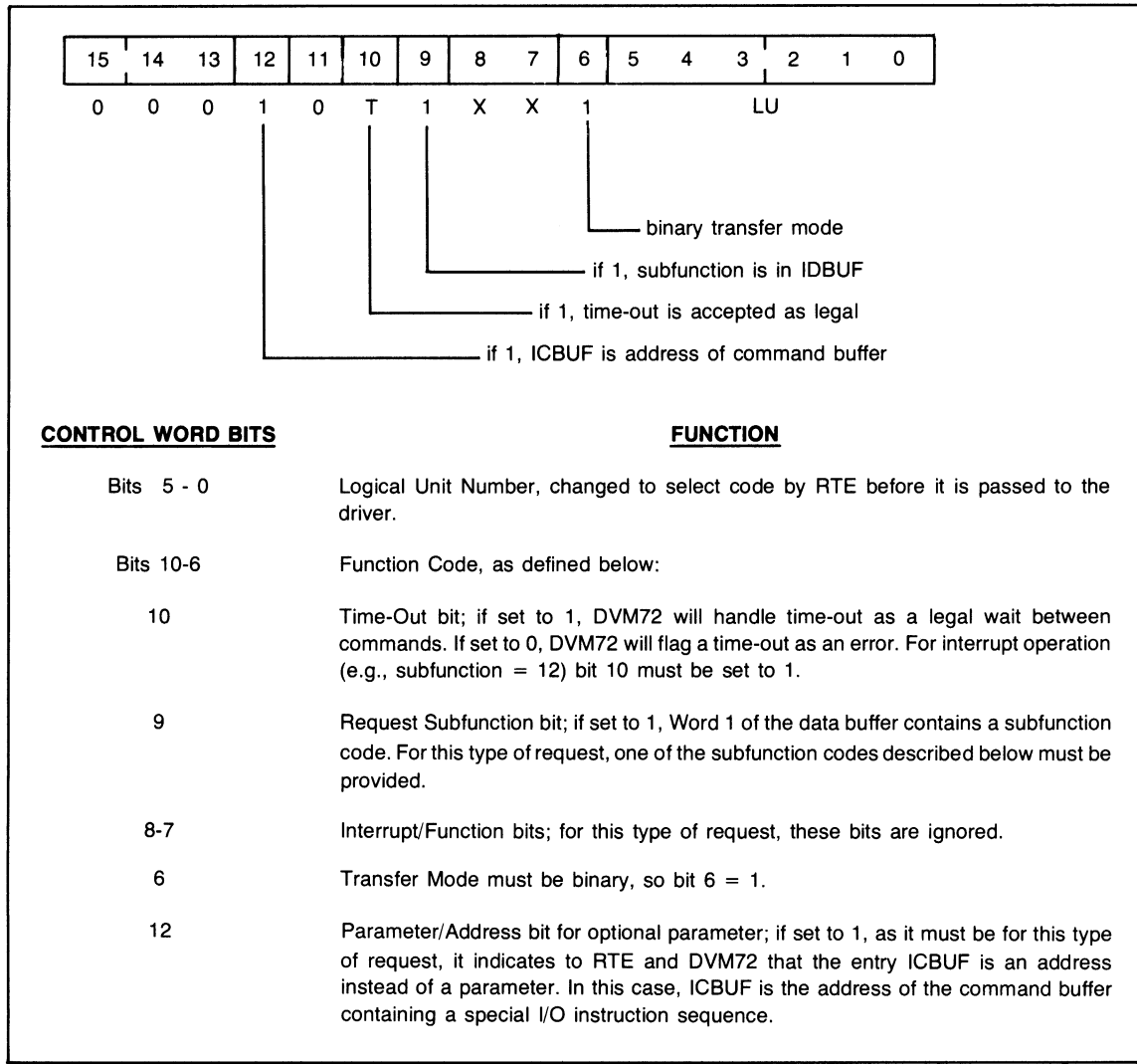
Figure 2-5. Control Word Format, Special Control Requests
