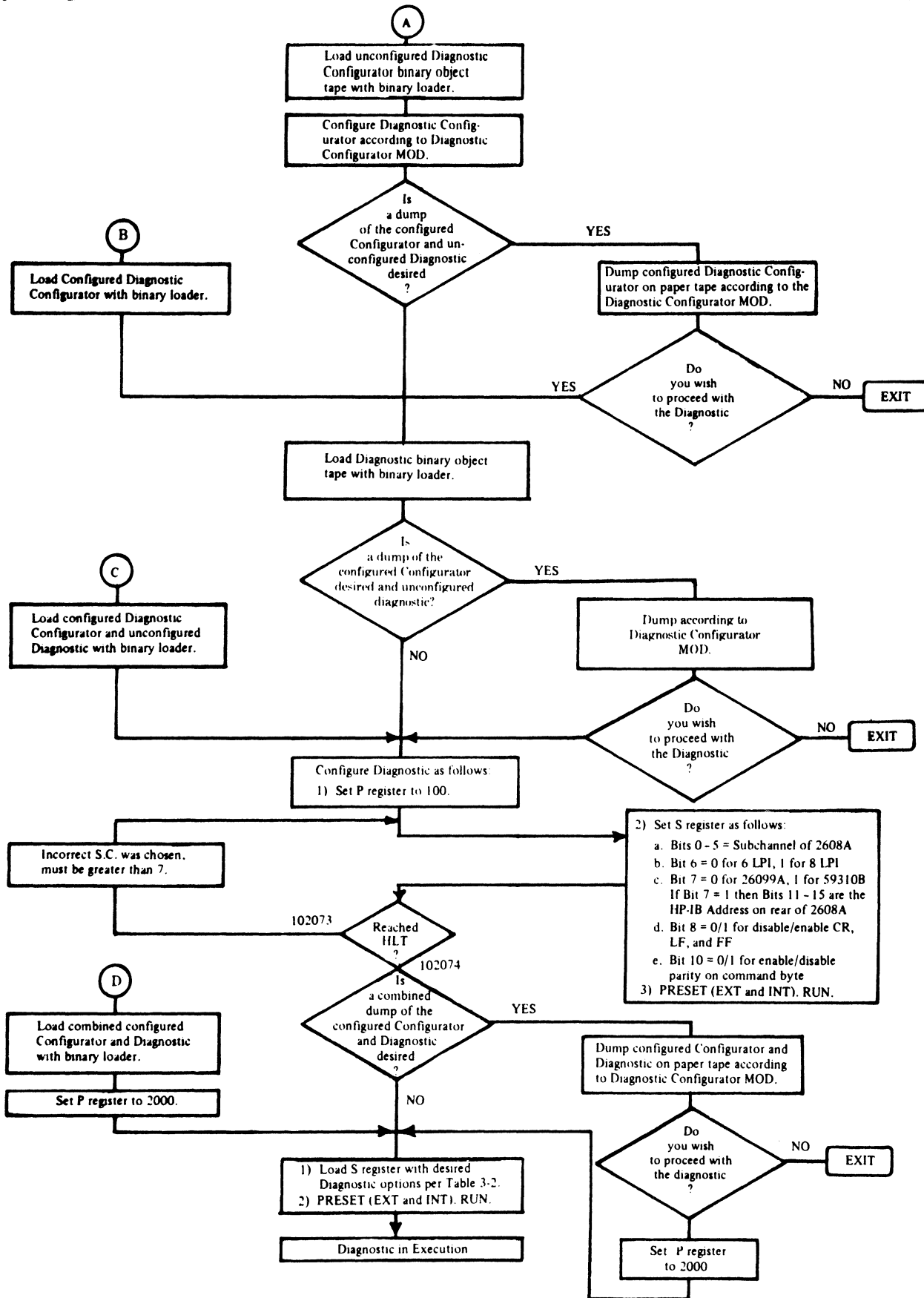
Figure 3-1. Operating Procedures Flowchart
