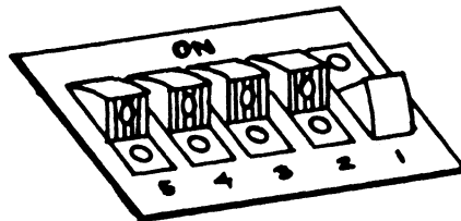
Figure 4-1. HP-IB Address Switch
