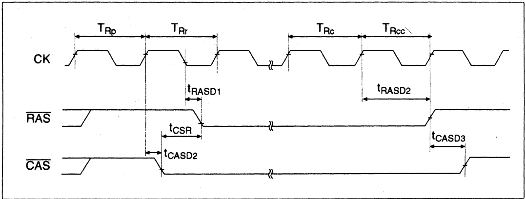
Figure 20.31 Self Refresh
