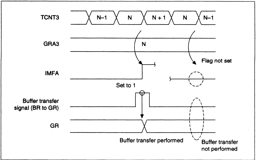
Figure 10.36 Overshoot Timing
