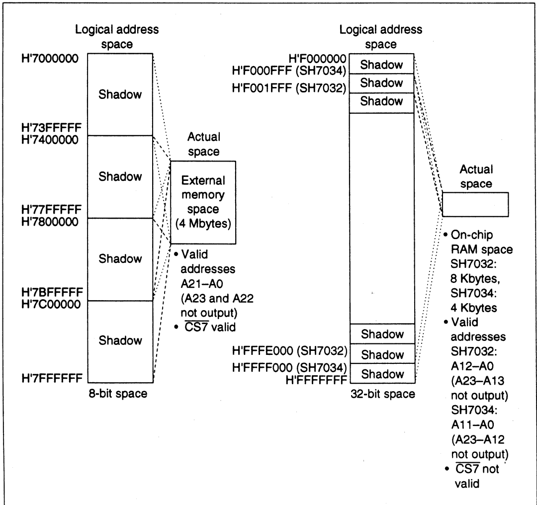
Figure 8 10 Memory Map of Area 7
