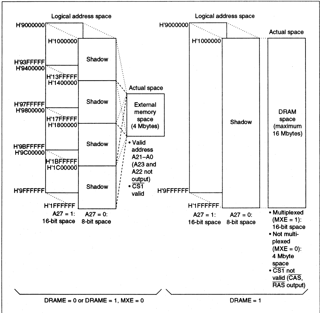
Figure 8.6 Memory Map of Area 1
