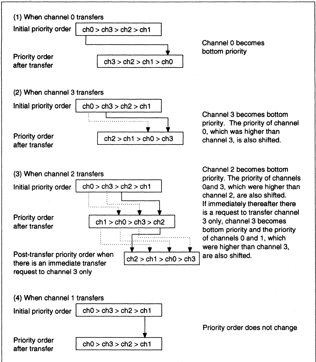
Figure 9.3 Round-Robin Mode
