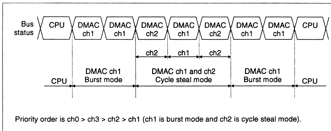
Figure 9.12 Bus Handling when Multiple Channels Are Operating
