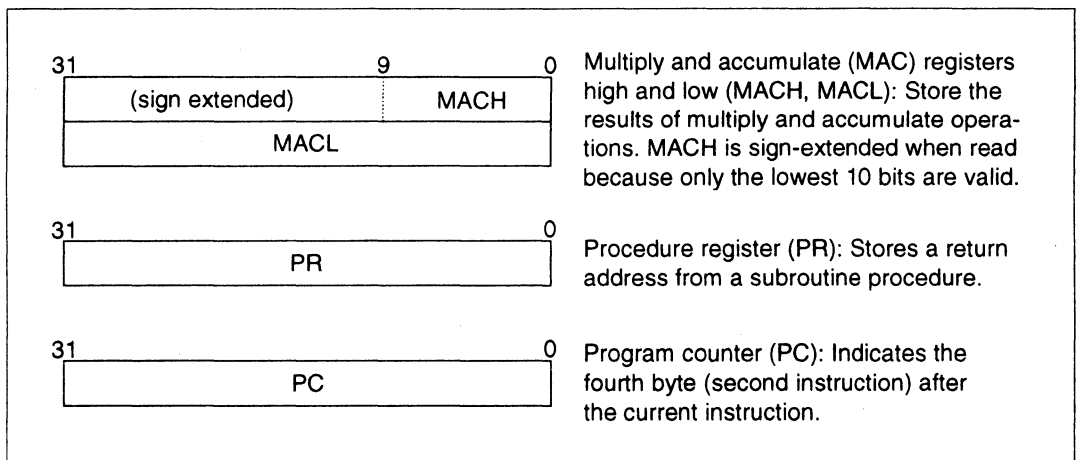
Figure 2.3 System Registers
