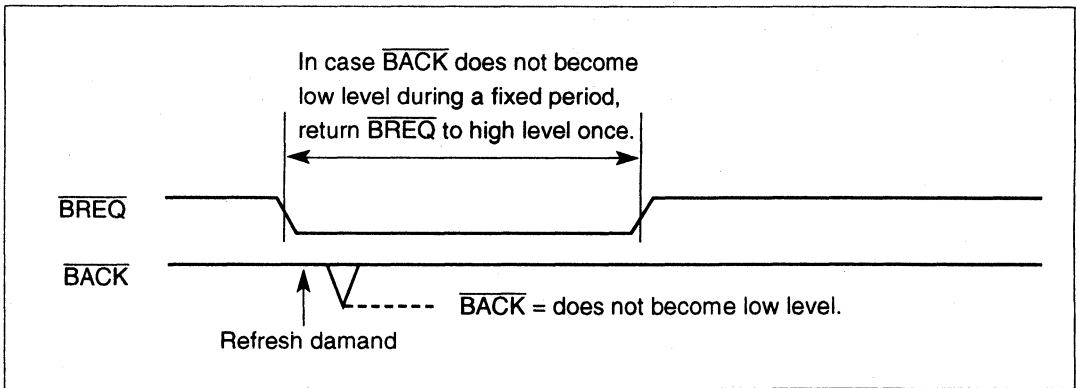
Figure 8.37 \overline{\text{BACK}} Operation by Refresh Demand (2)
