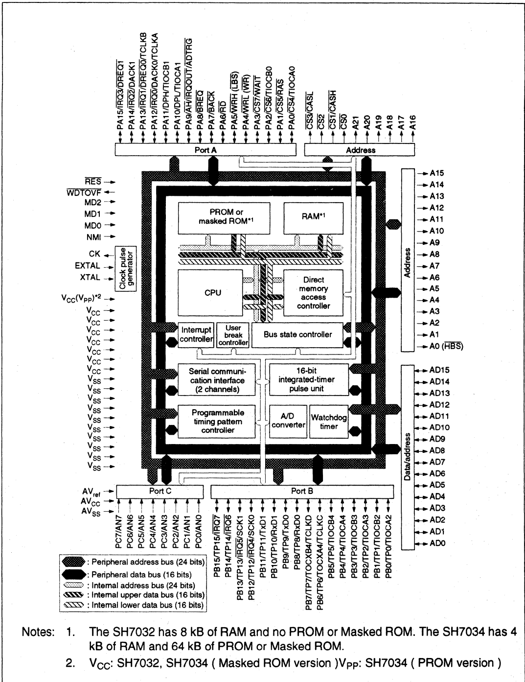
Figure 1.1 Block Diagram
