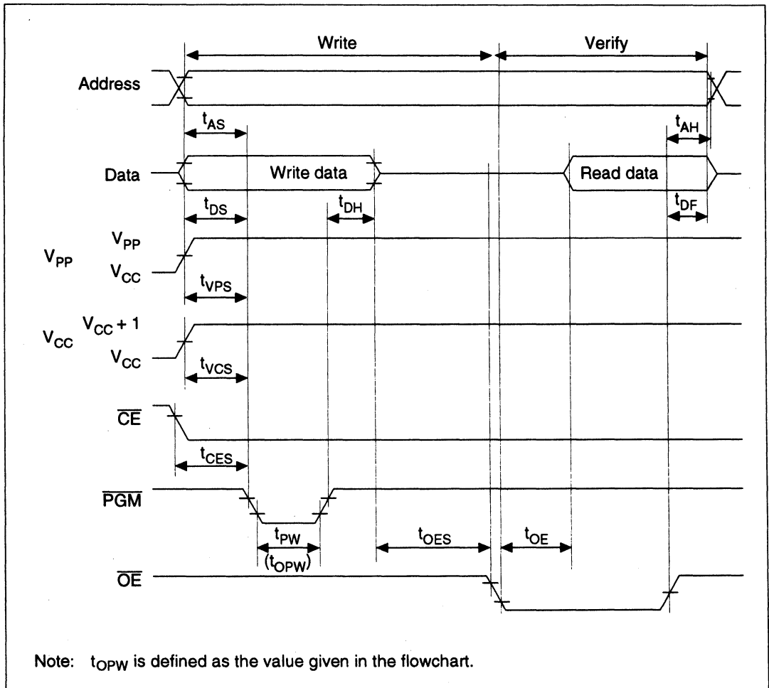
Figure 17.5 Write/Verify Timing
