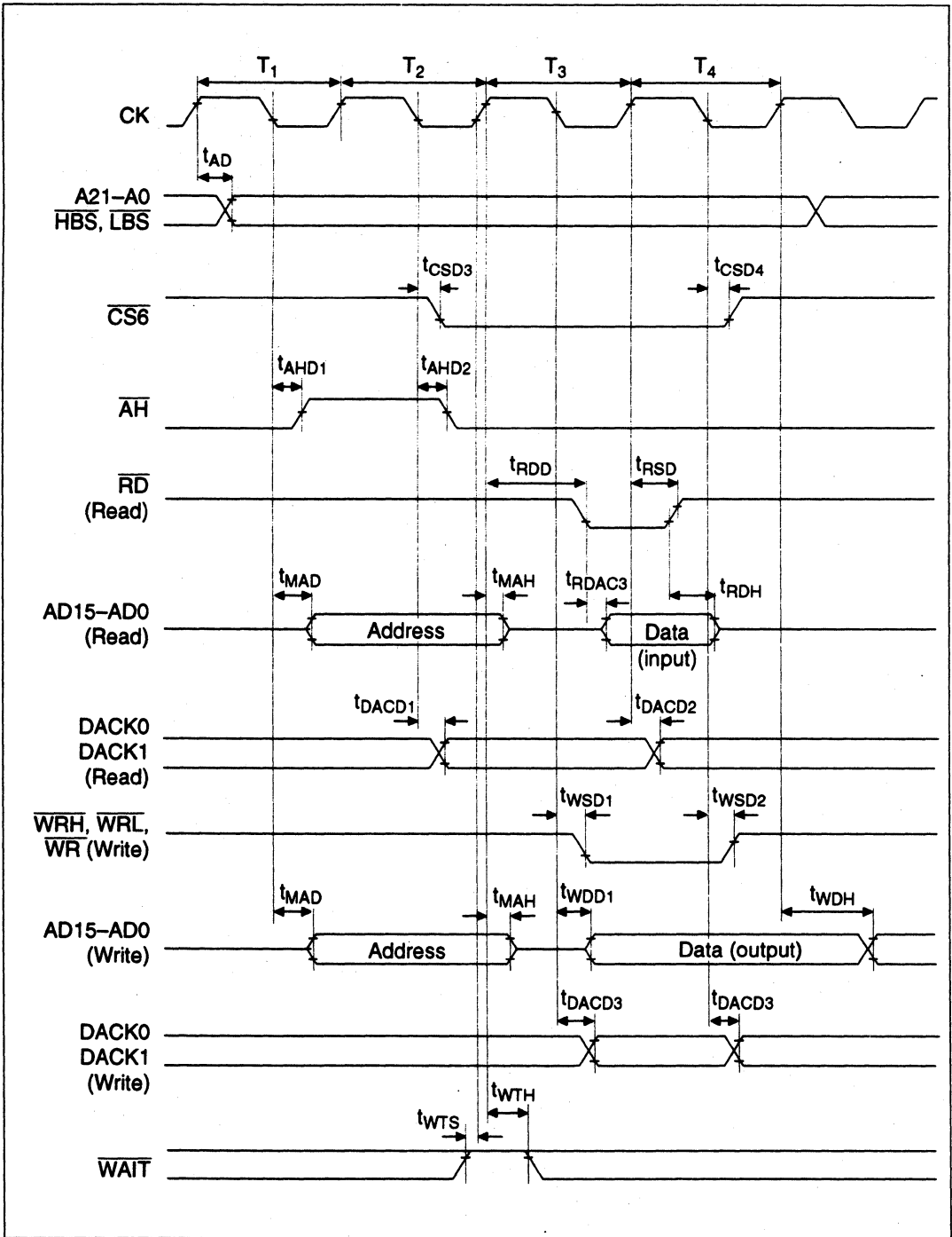
Figure 20.19 Address/Data Multiplex I/O Bus Cycle
