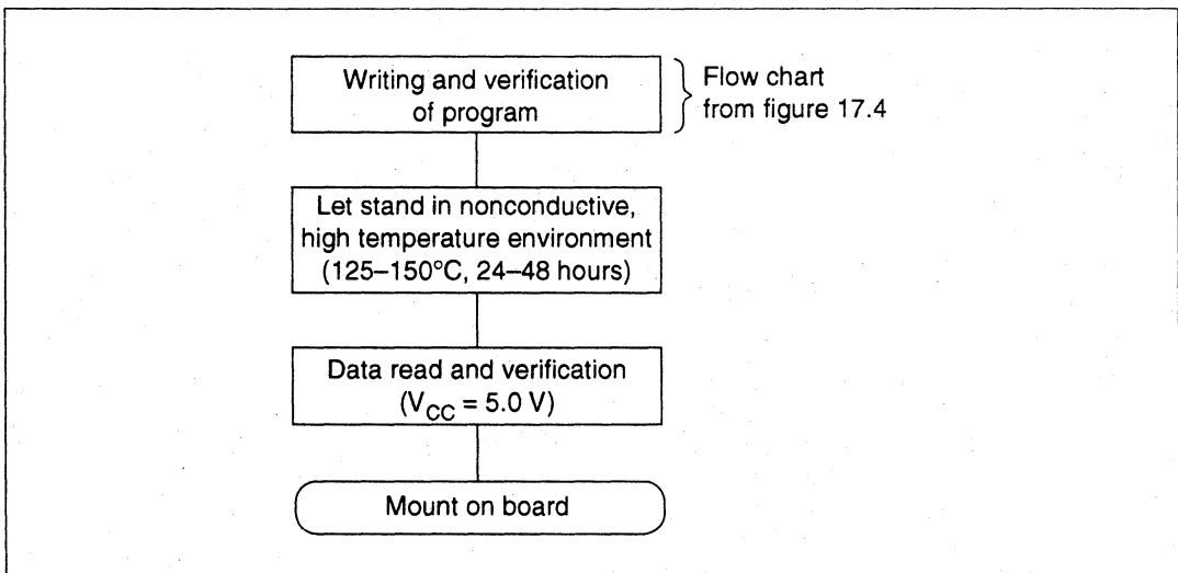
Figure 17.6 Screening Flow
