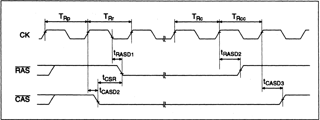
Figure 20.18 Self Refresh
