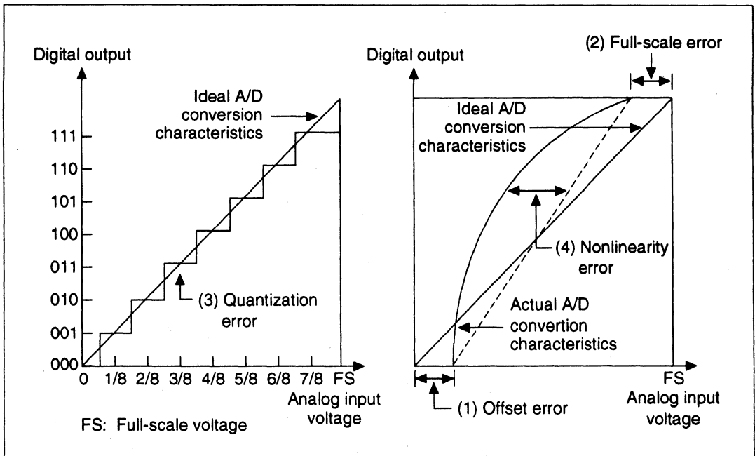
Figure 14.7 Definitions of A/D Conversion Accuracy
