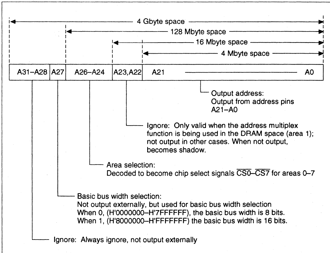
Figure 8.3 Address Format
