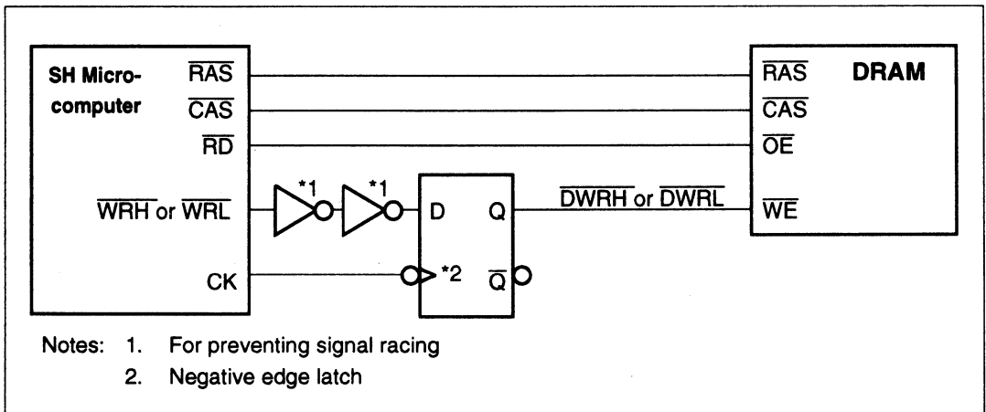
Figure 8.42 Delayed-Write Control Circuit
