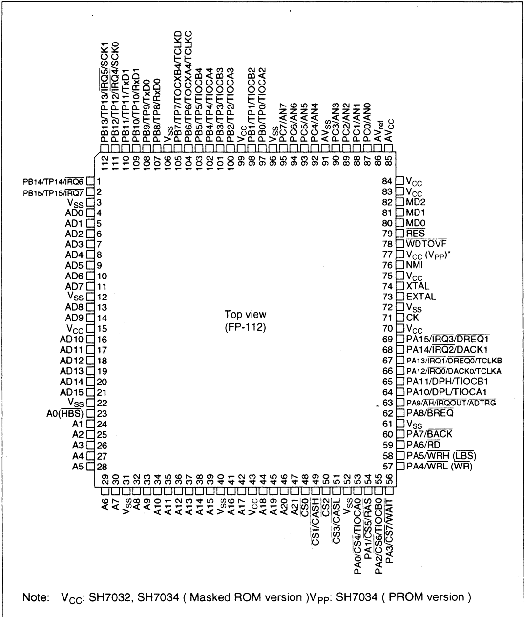
Figure 1.2 Pin Arrangement
