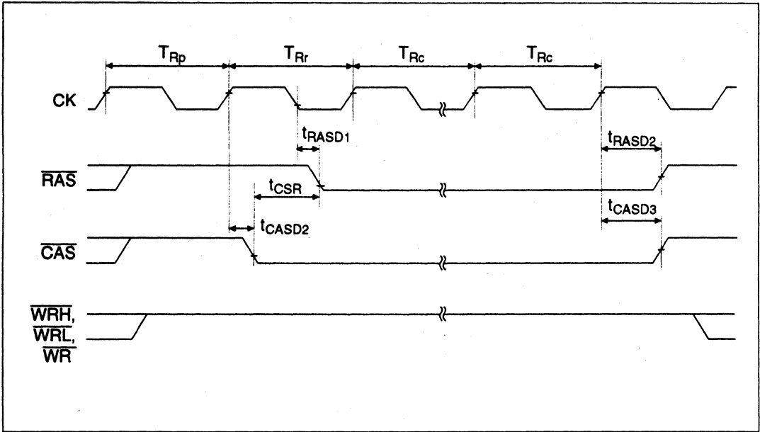
Figure 20.16 CAS-before-RAS Refresh (Short Pitch)
