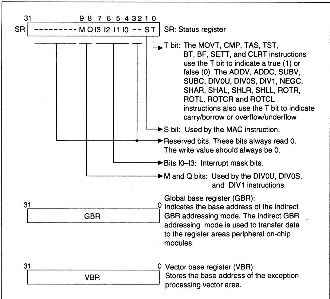
Figure 2.2 Control Registers
