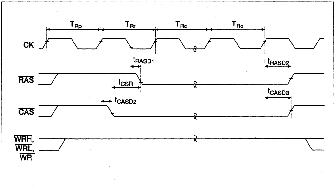
Figure 20.17 CAS-before-RAS Refresh (Long Pitch)
