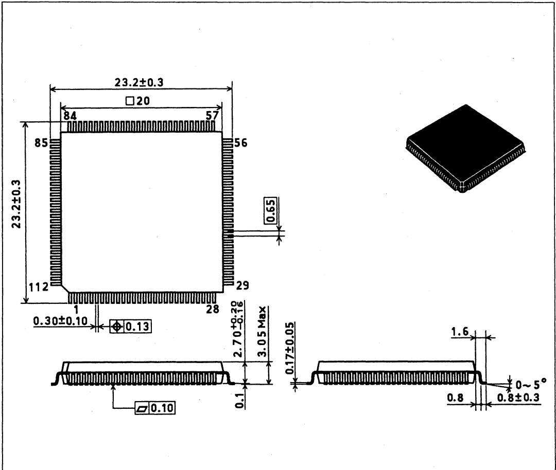
Figure C.1 External Dimensions
