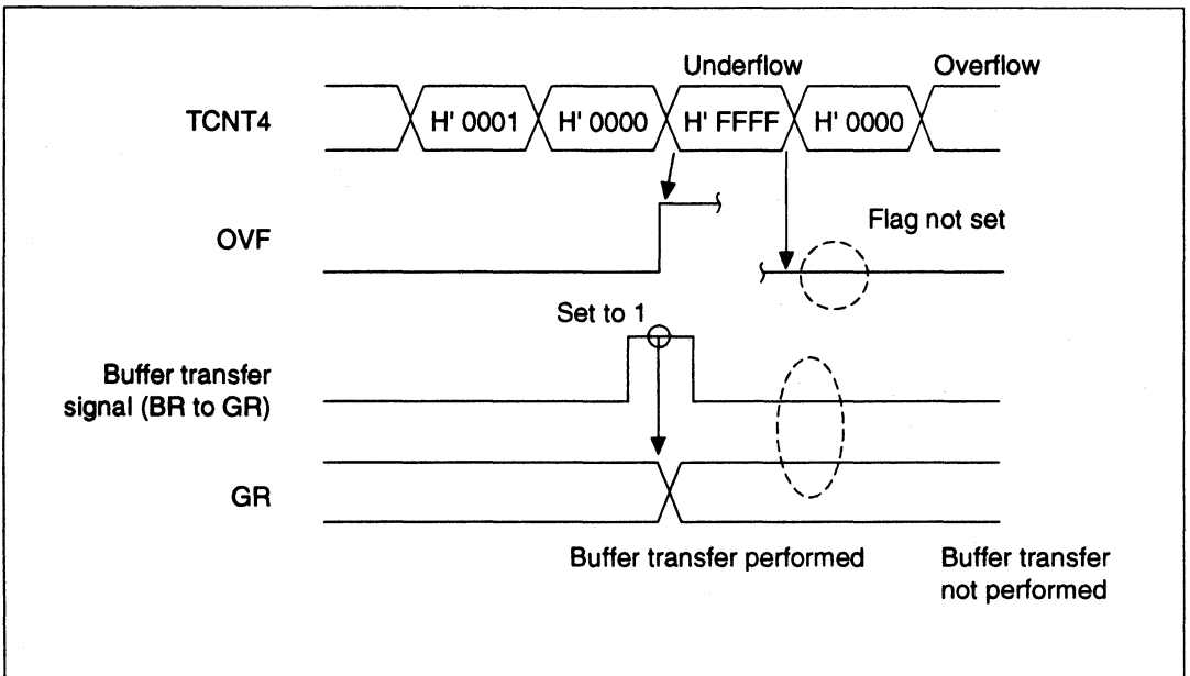
Figure 10.37 Undershoot Timing
