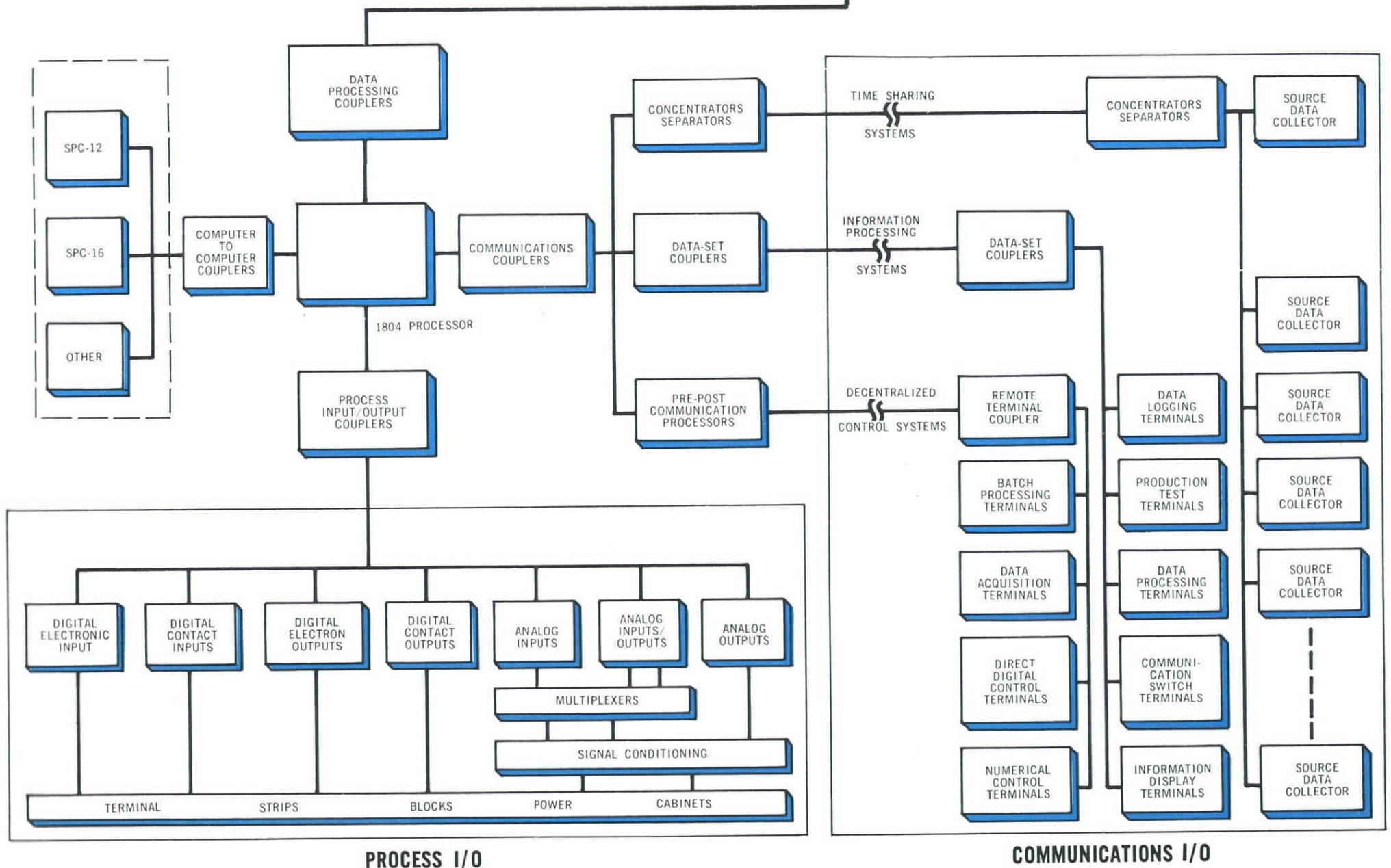
DATA PROCESSING I/O
