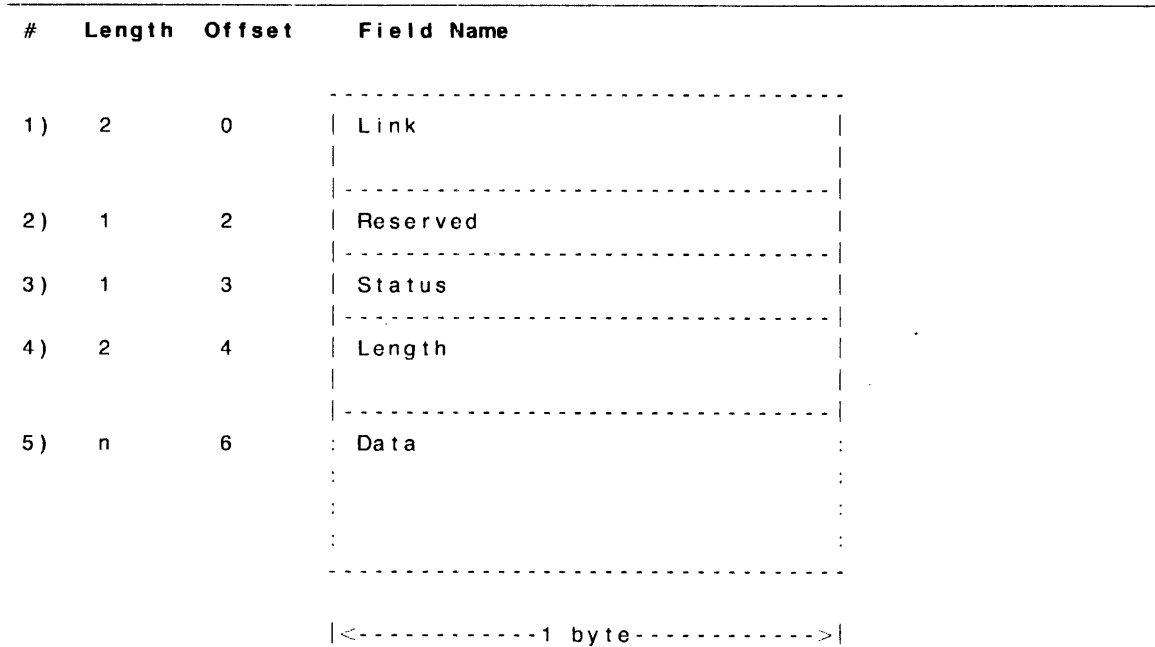
Figure 5-5: Message Buffer Format
