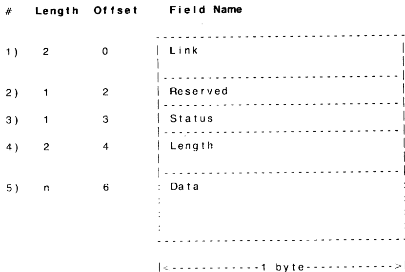
Figure 2-5: Message Buffer Format
