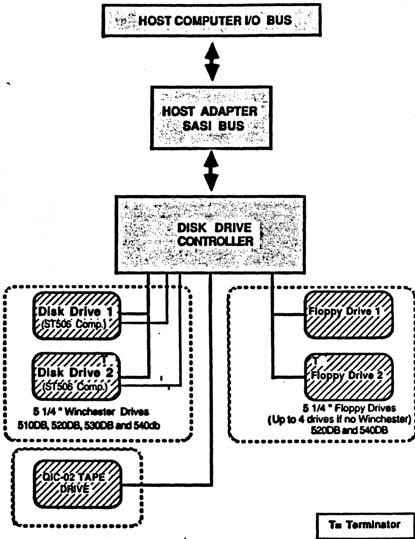
Figure 3-1 Typical System Configuration
