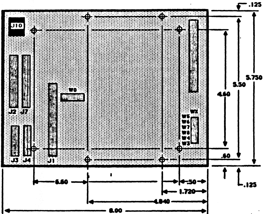
Figure 540db BOARD DIMENSIONS
