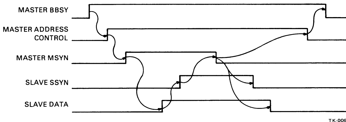
Figure 2-30 Typical DATI Transaction, Timing Diagram
