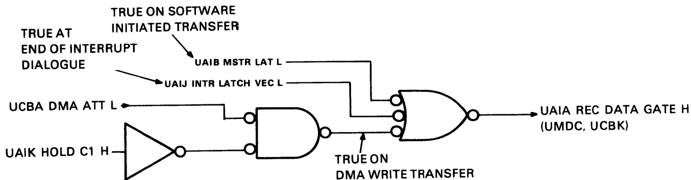
Figure 3-45 Qualifying the REC DATA GATE Signal
