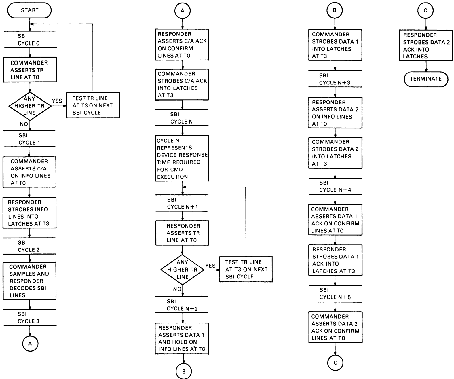
Figure 2-22 Extended Read Timing Chart and Flow (Sheet 2 of 2)
