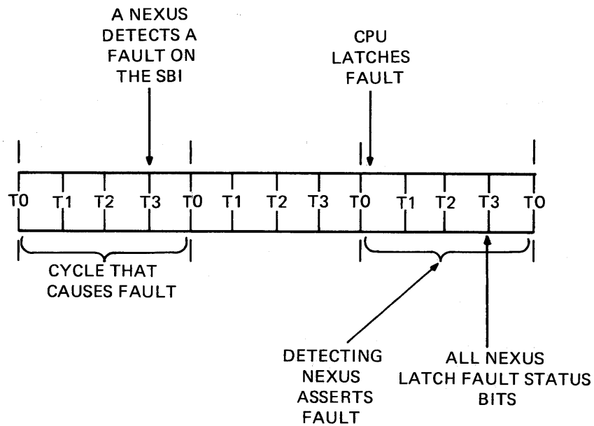
Figure 2-13 Fault Timing
