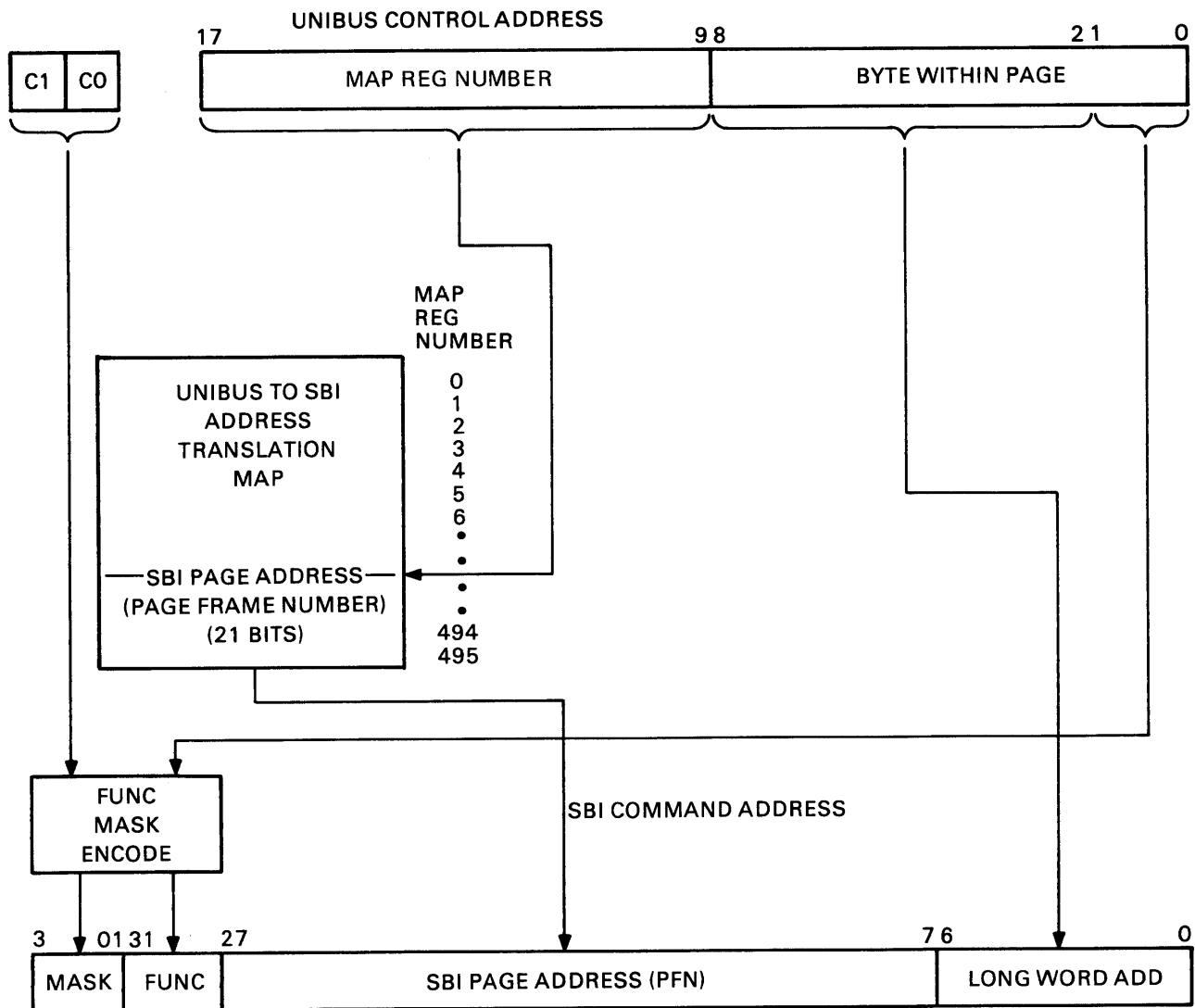
Figure 2-38 Unibus to SBI Address Translation
