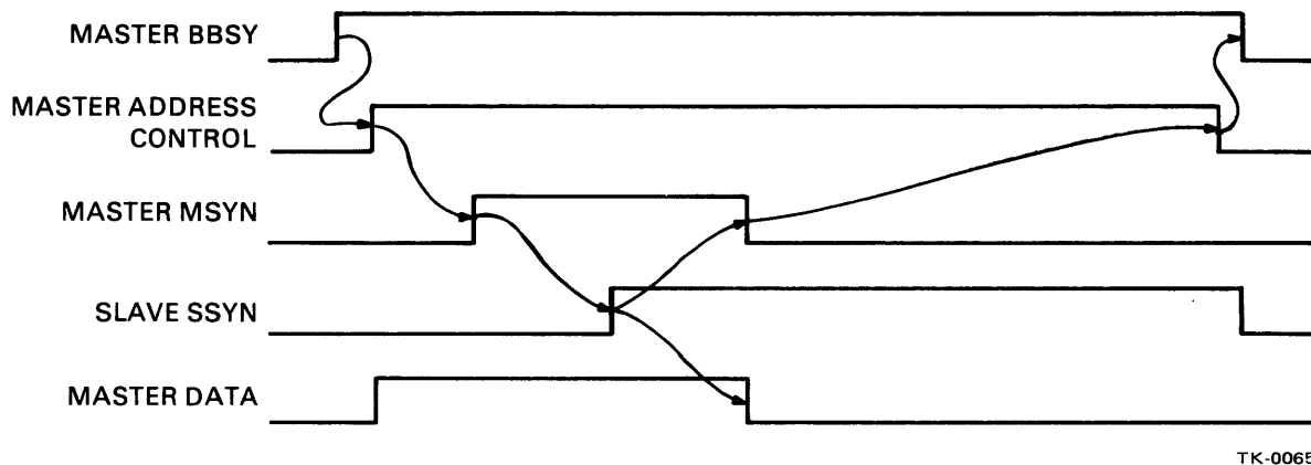
Figure 2-29 Typical DATO Transaction, Timing Diagram
