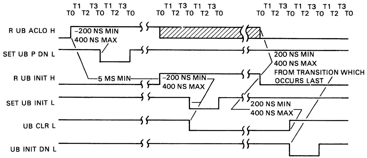
Figure 3-63 Unibus Status Sequencer, Timing Diagram
