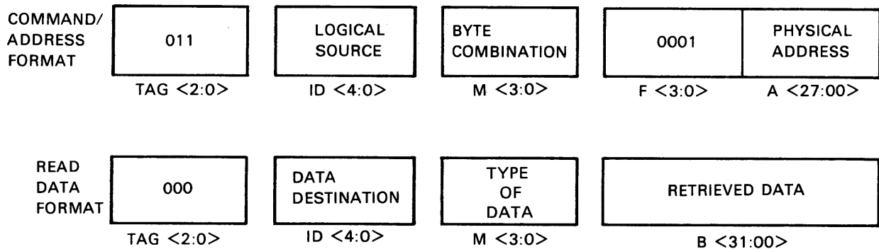
Figure 2-19 Read Masked Function Format
