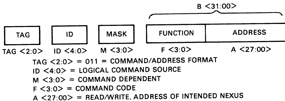
Figure 2-6 Command/Address Format
