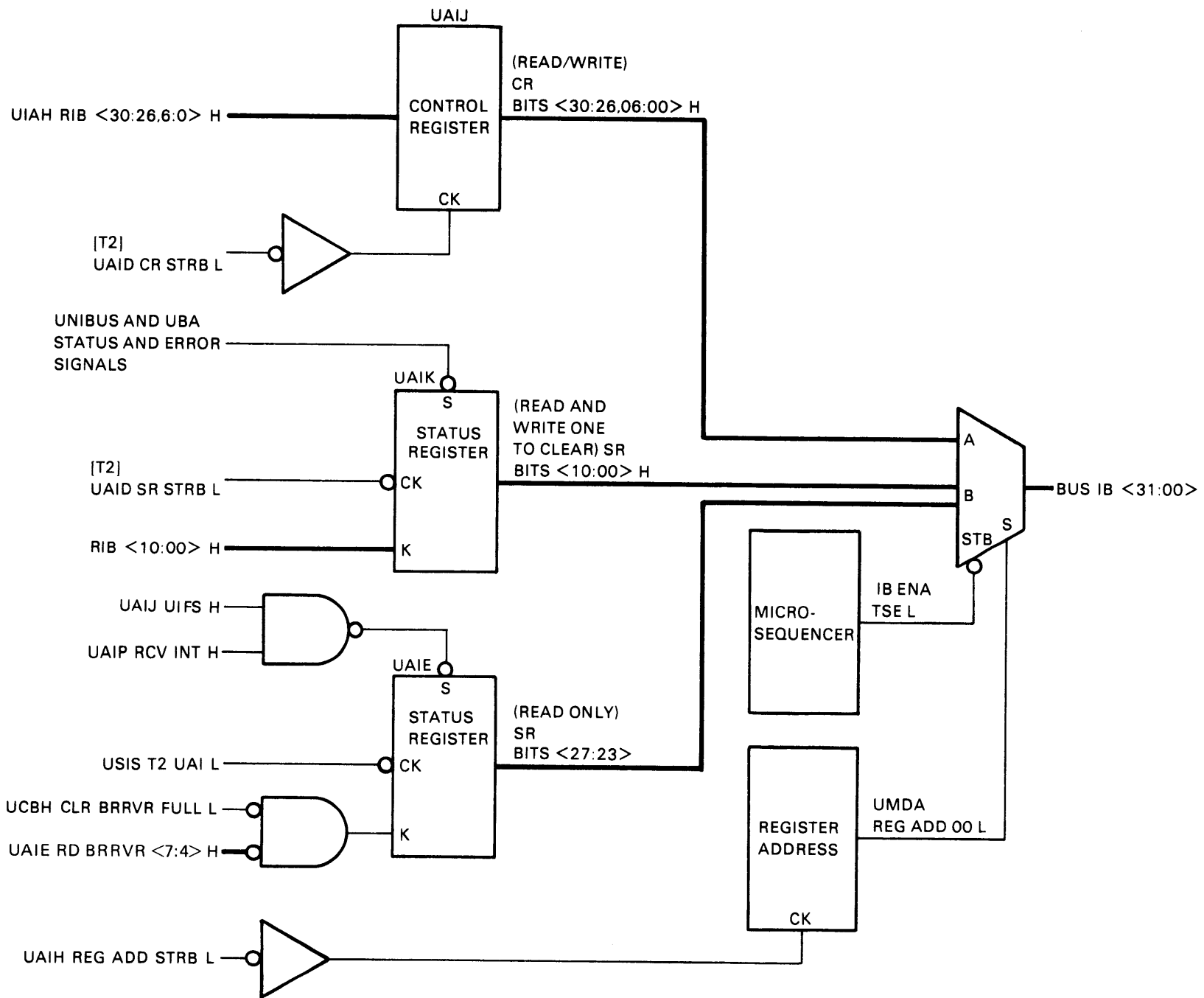
Figure 3-68 Control and Status Registers, Block Diagram
