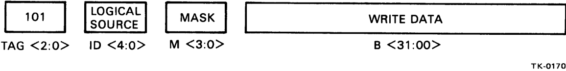
Figure 2-9 Write Data Formats
