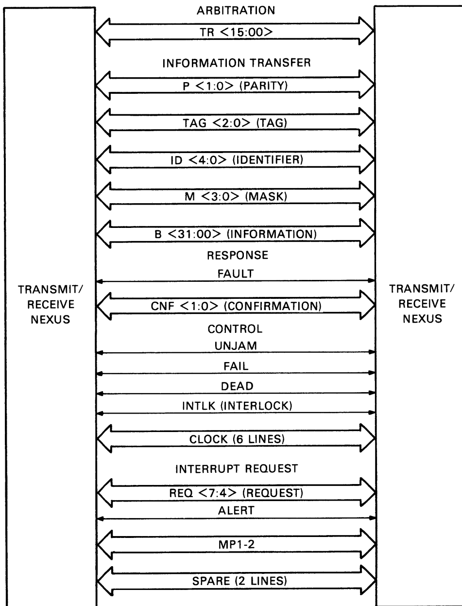
Figure 2-4 SBI Configuration
