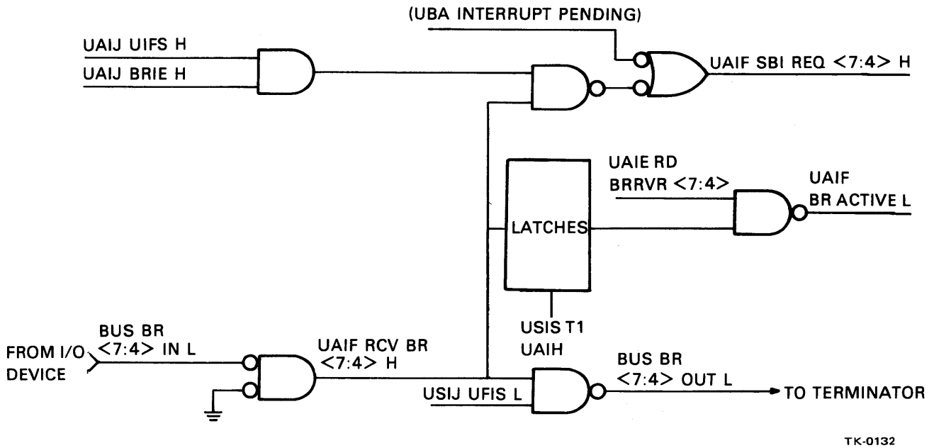
Figure 3-49 BR Logic
