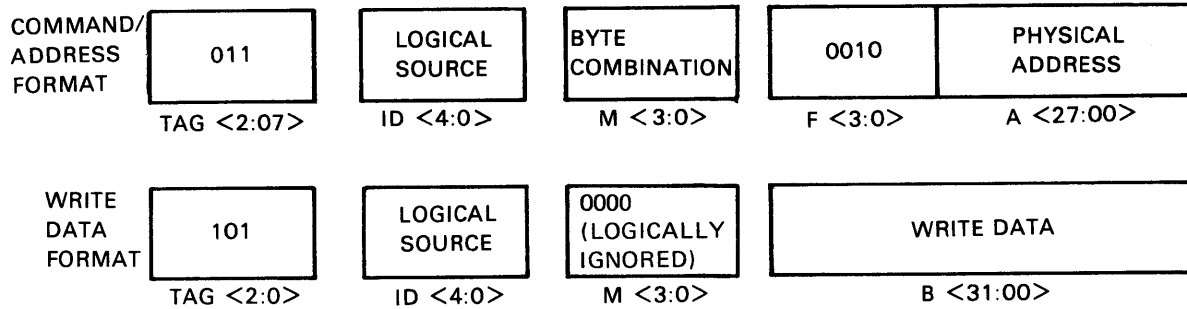
Figure 2-23 Write Masked Function Format
