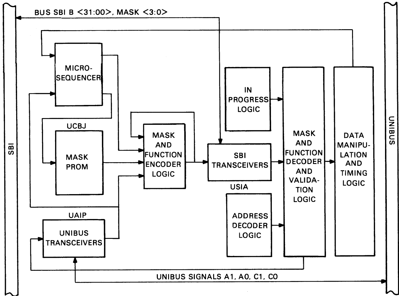
Figure 2-58 Mask and Function Logic, Block Diagram
