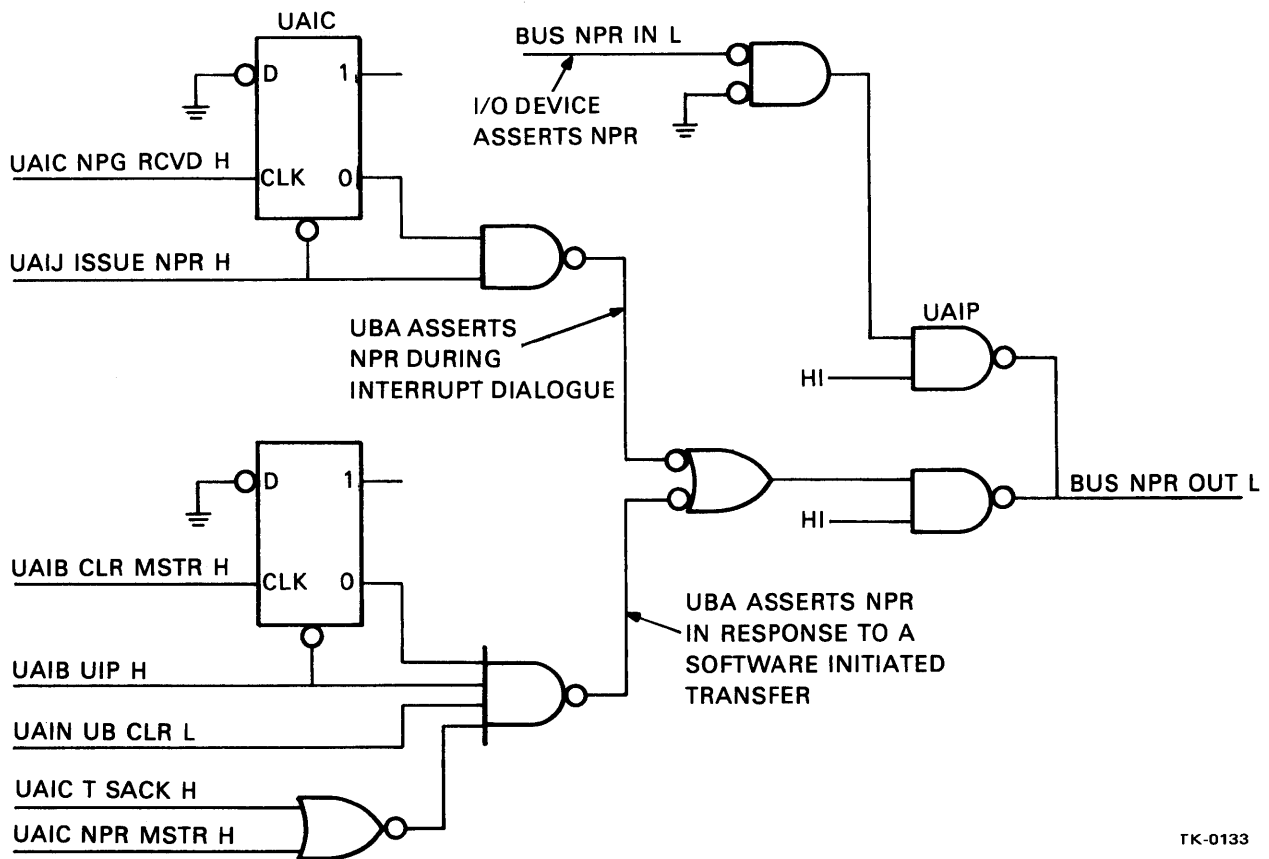
Figure 3-50 NPR Logic
