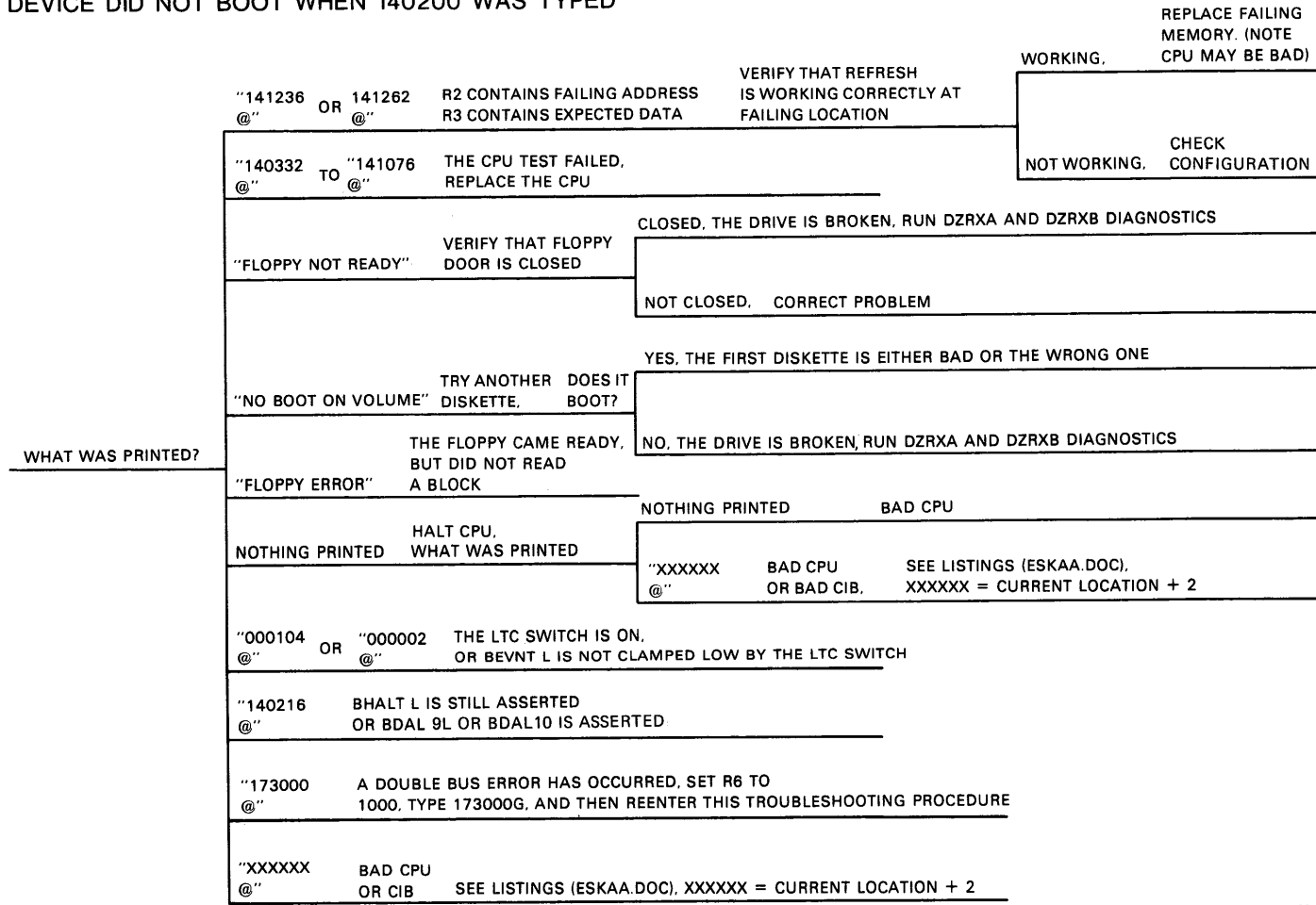
Figure C-3 140200G Console Boot Failure Flowchart
