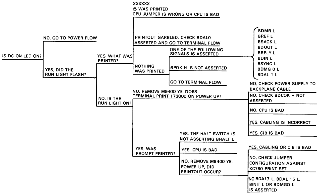
Figure C-1 Console DC ON Flowchart
