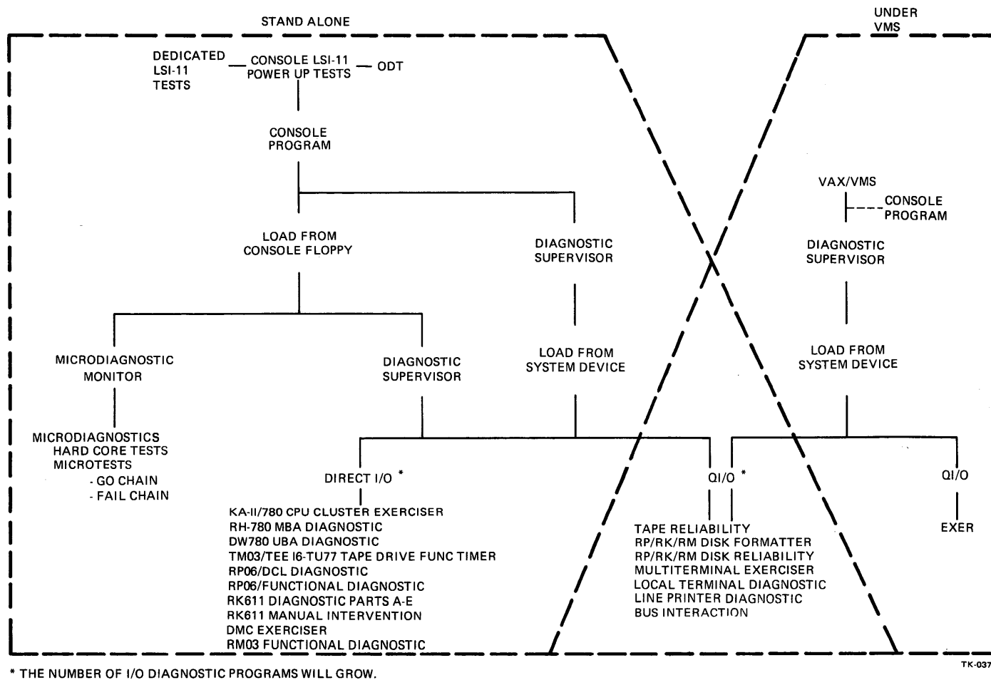
Figure 1-2 VAX-11/780 Diagnostic System Execution Environments
