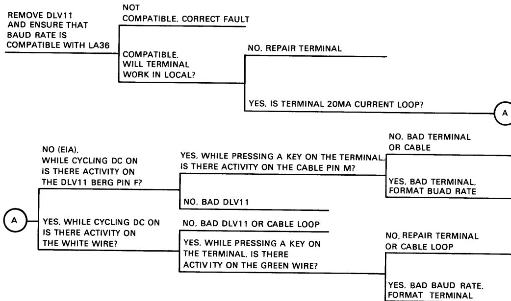
Figure C-5 Console Terminal Troubleshooting Flowchart
