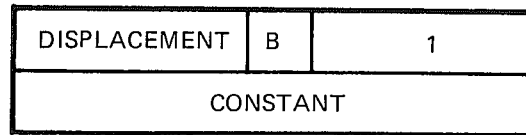
Figure 8–17: Internal Relocation (Entry Type 1)
