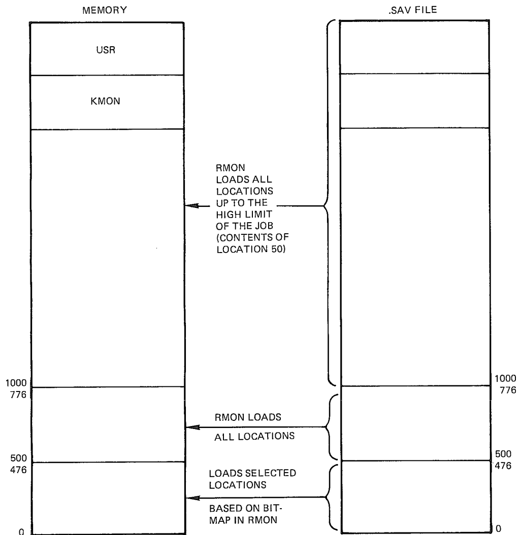
Figure 2-10: R Command
