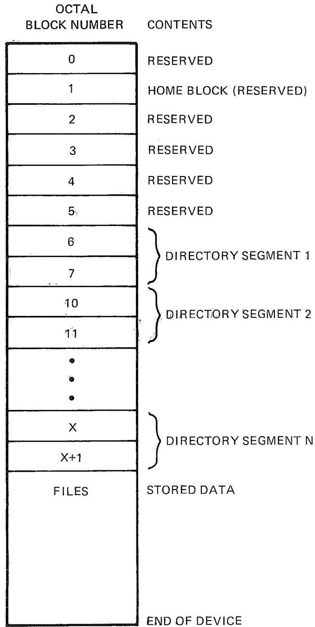
Figure 9-1: Random-Access Device
