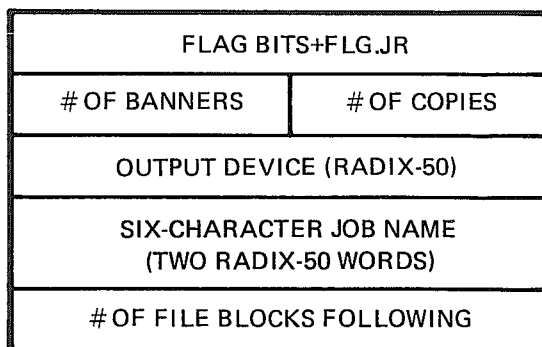
Figure 3-19: Job Block
