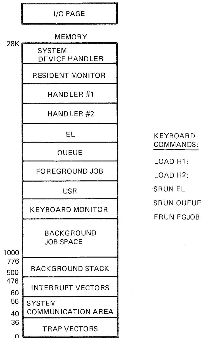
Figure 2-16: FB System
