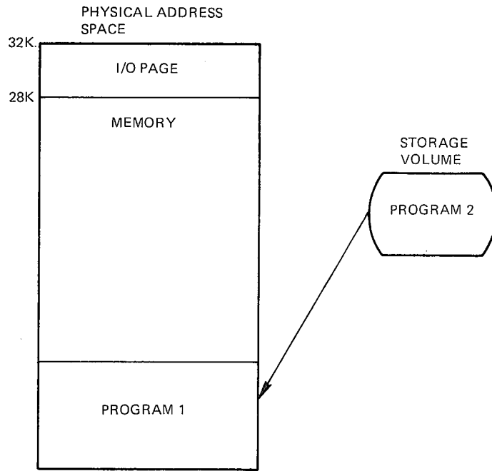
Figure 4-3: Chaining
