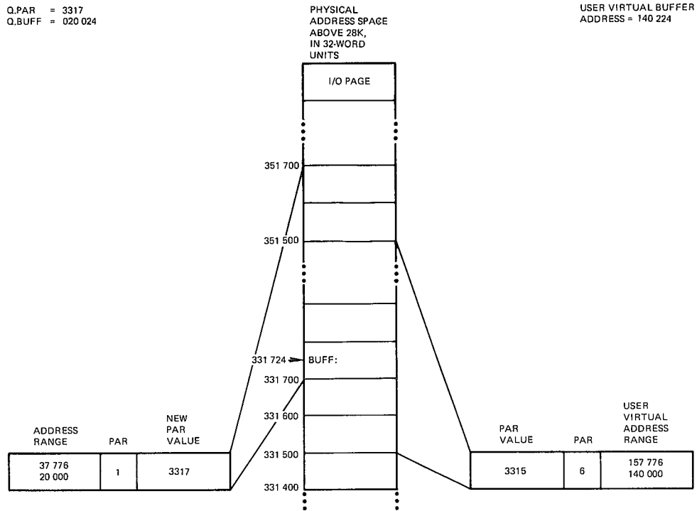
Figure 7-6: PAR1 Mapping
