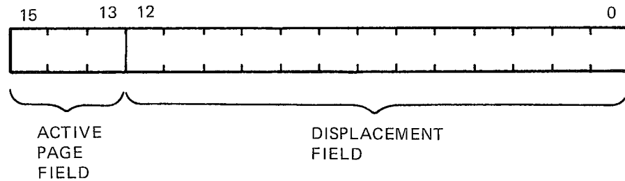
Figure 4-17: Virtual Address
