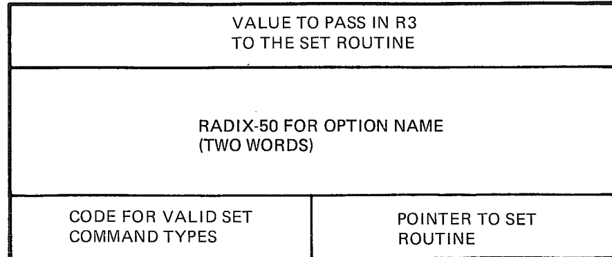
Figure 7-2: SET Option Table
