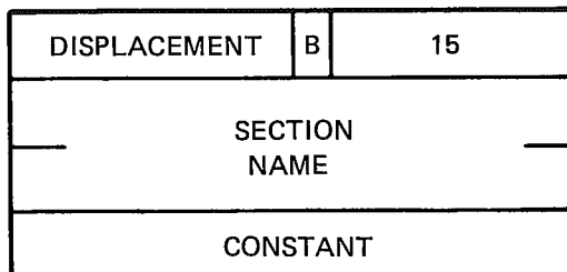
Figure 8–28: P-sect Additive Relocation (Entry Type 15)
