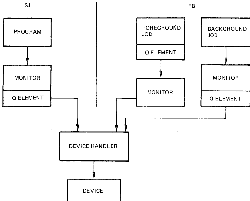
Figure 3-6: Components of the Queued I/O System
