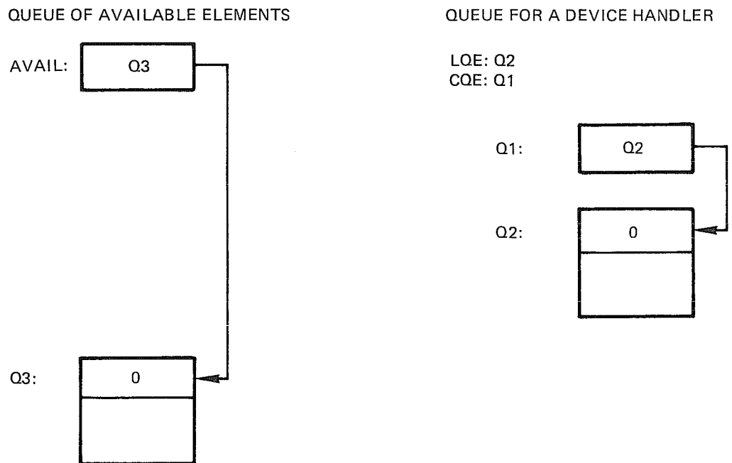
Figure 3-10: I/O Queue with One Available Element
