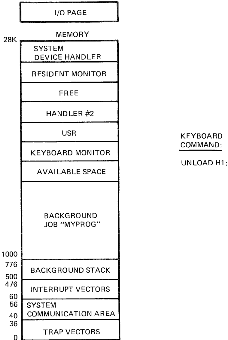
Figure 2-12: SJ System with One Handler Unloaded
