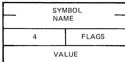
Figure 8–10: Global Symbol Name Entry Format (Entry Type 4)
