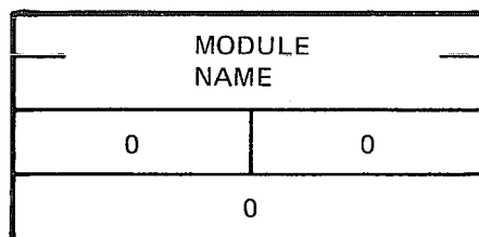
Figure 8-6: Module Name Entry Format (Entry Type 0)
