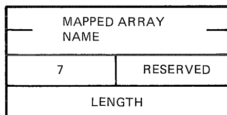
Figure 8–13: Mapped Array Declaration Entry Format (Entry Type 7)
