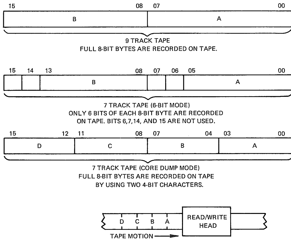
Figure 10-3: Seven-Track Tape
