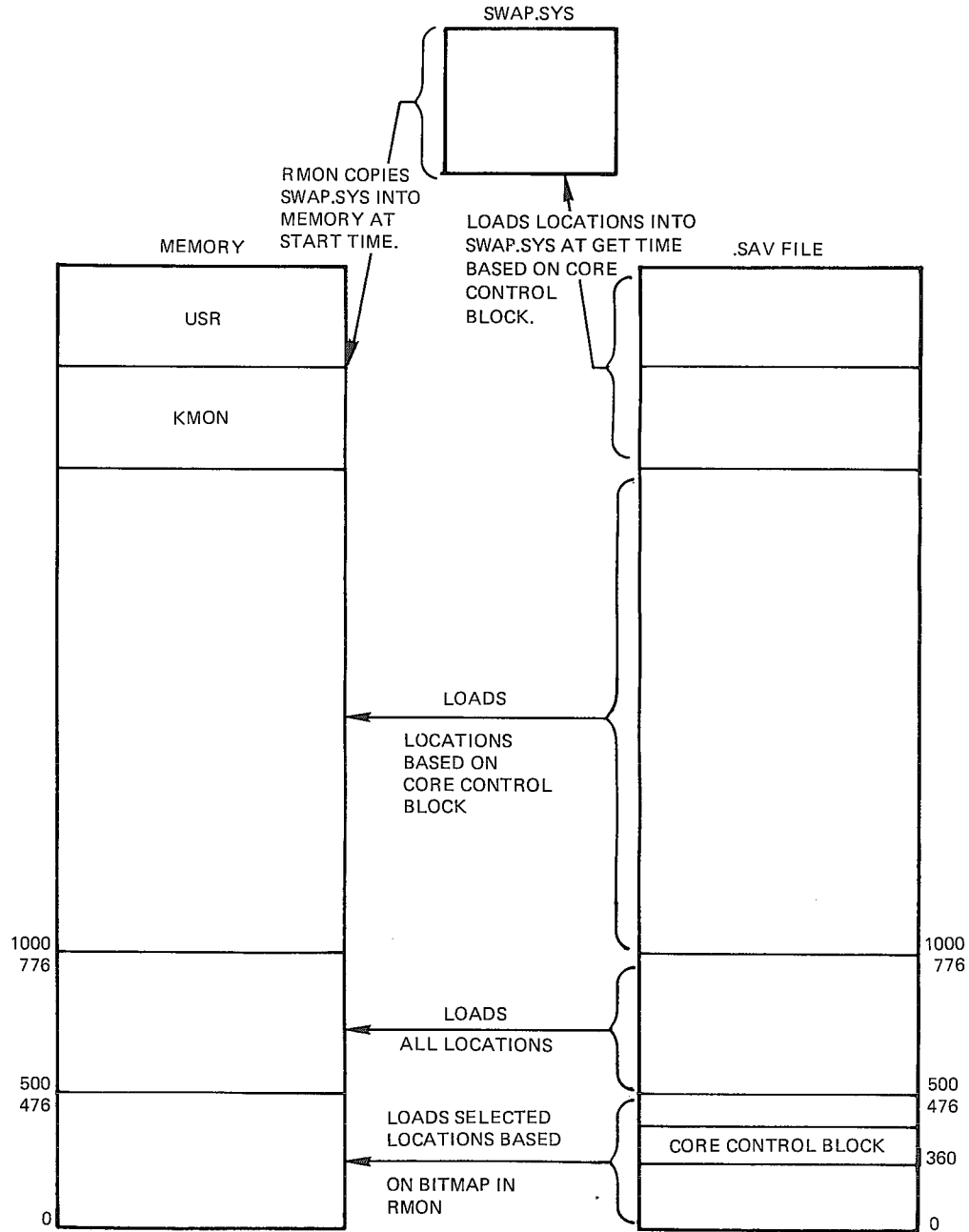
Figure 2-9: RUN Command
