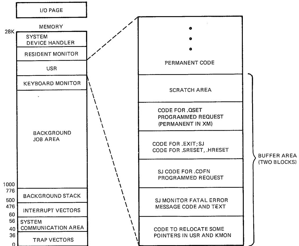
Figure 2-17: USR
