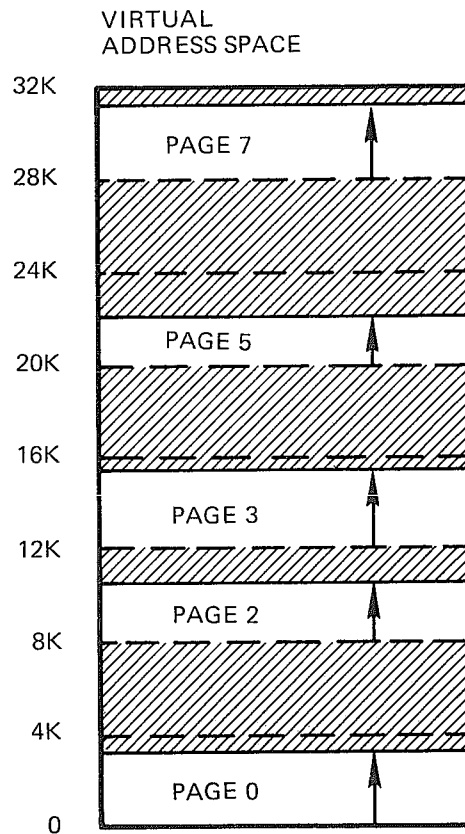
Figure 4-10: Smaller Pages
