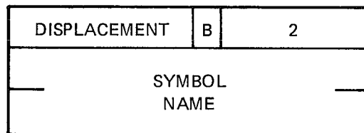
Figure 8–18: Global Relocation (Entry Type 2)
