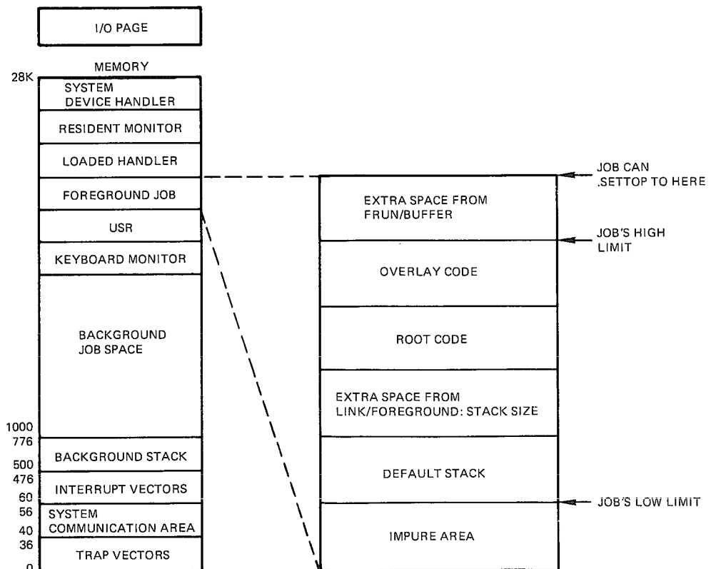
Figure 2-14: Foreground Job
