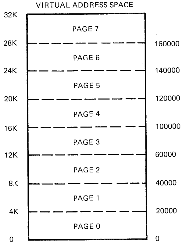
Figure 4-10: Smaller Pages
