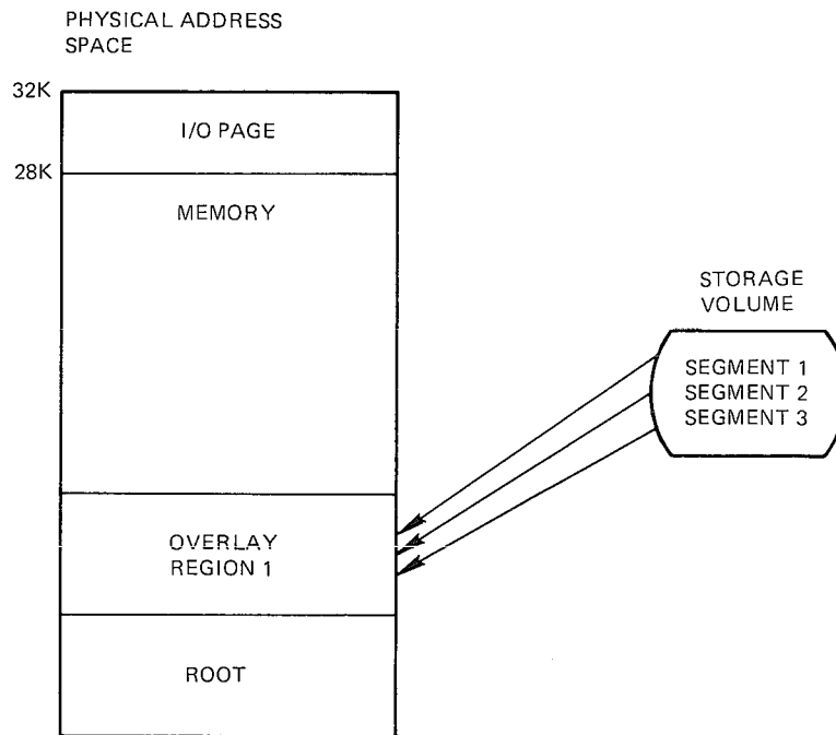
Figure 4-4: Overlaying
