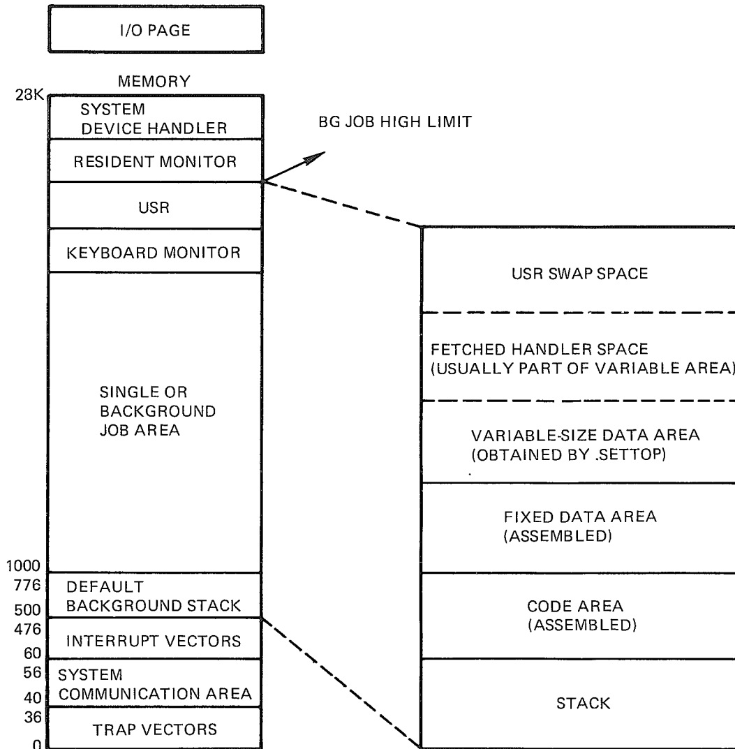
Figure 2-8: Background Job
