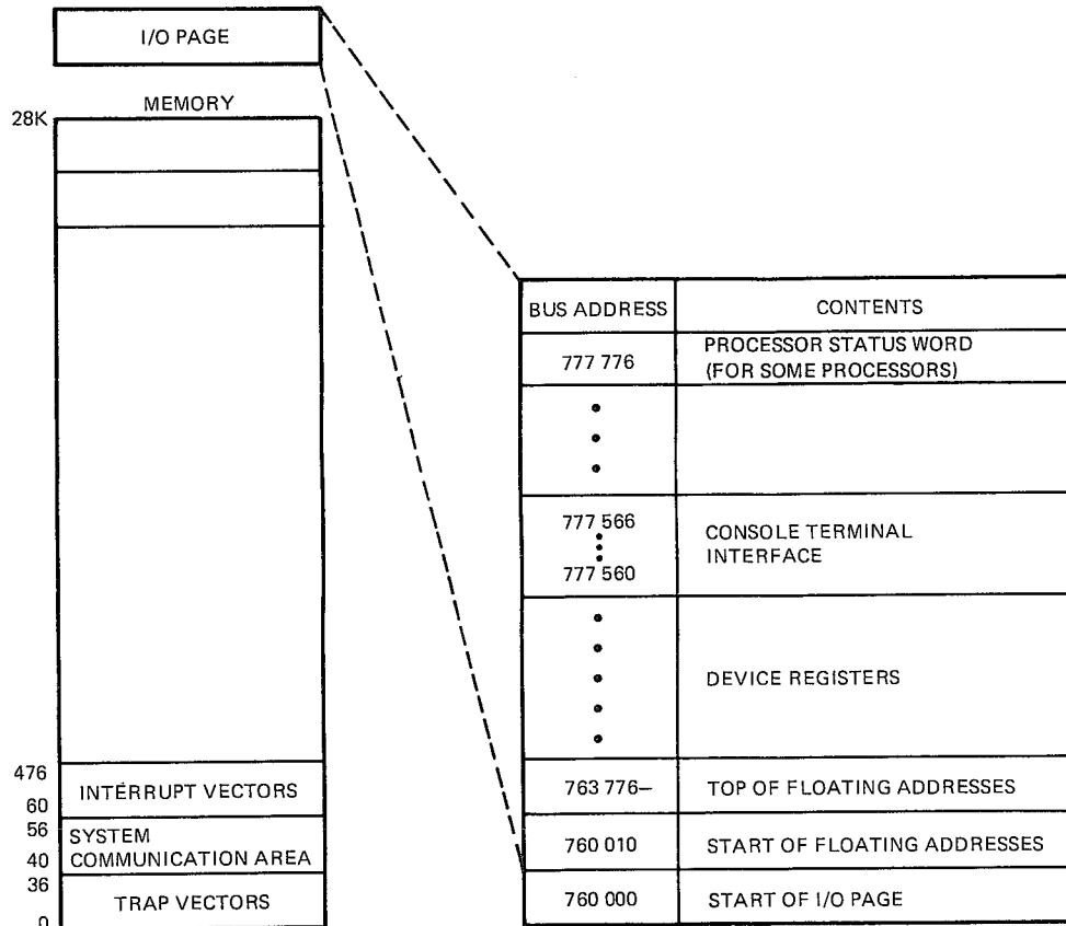
Figure 2-5: I/O Page
