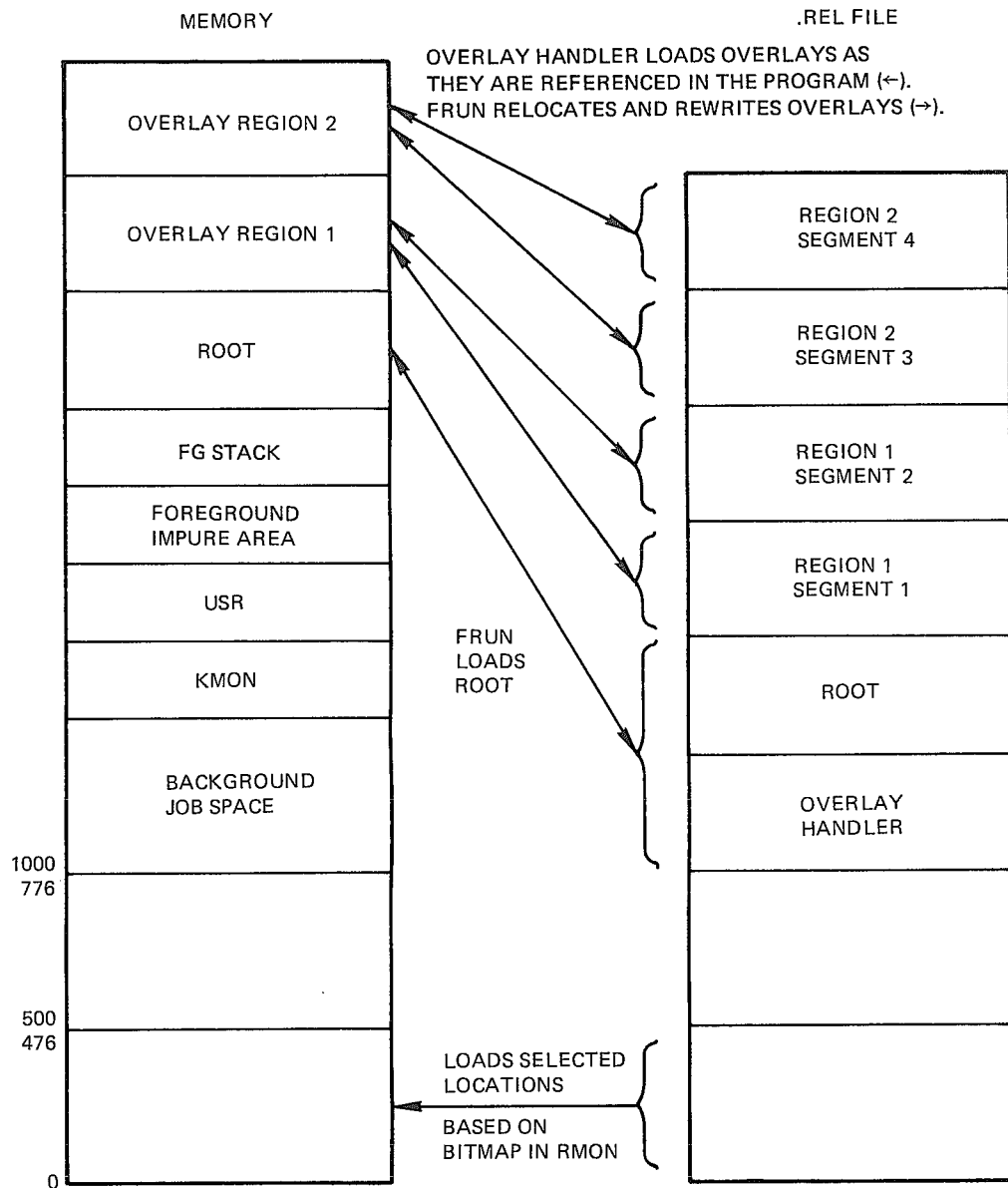
Figure 2-15: FRUN Command
