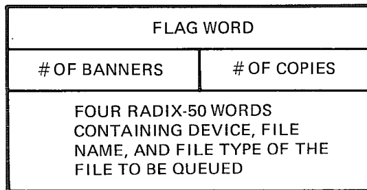
Figure 3-20: File Block
