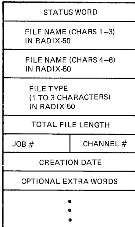
Figure 9-4: Directory Entry Format
