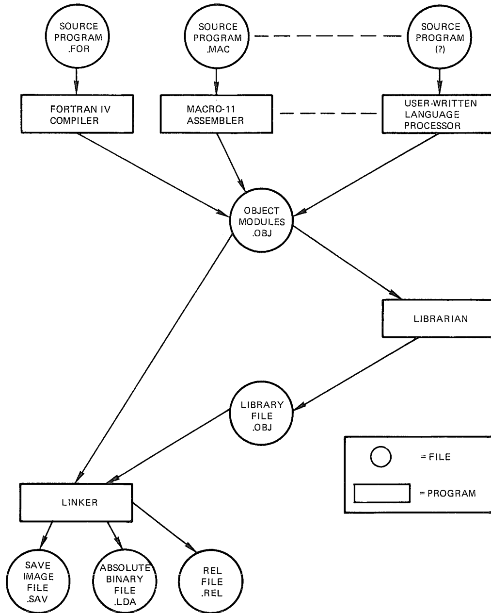
Figure 8-1: Object Module Processing
