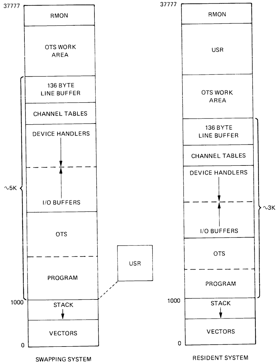
Figure 2-3 RT-11 8K System Runtime Memory Organization
