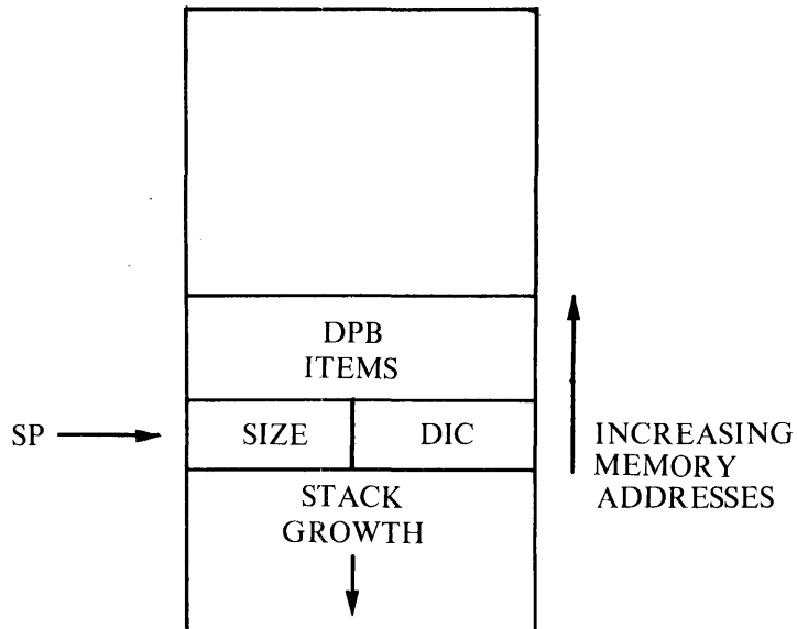
Figure 1-2 Directive Parameter Block (DPB) On The Stack
