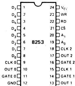
PIN CONFIGURATION
