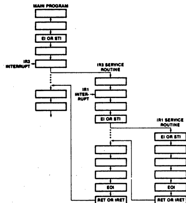
Figure 12. Fully Nested Mode Example (MCS 80/85™ or MCS 86/88™)
