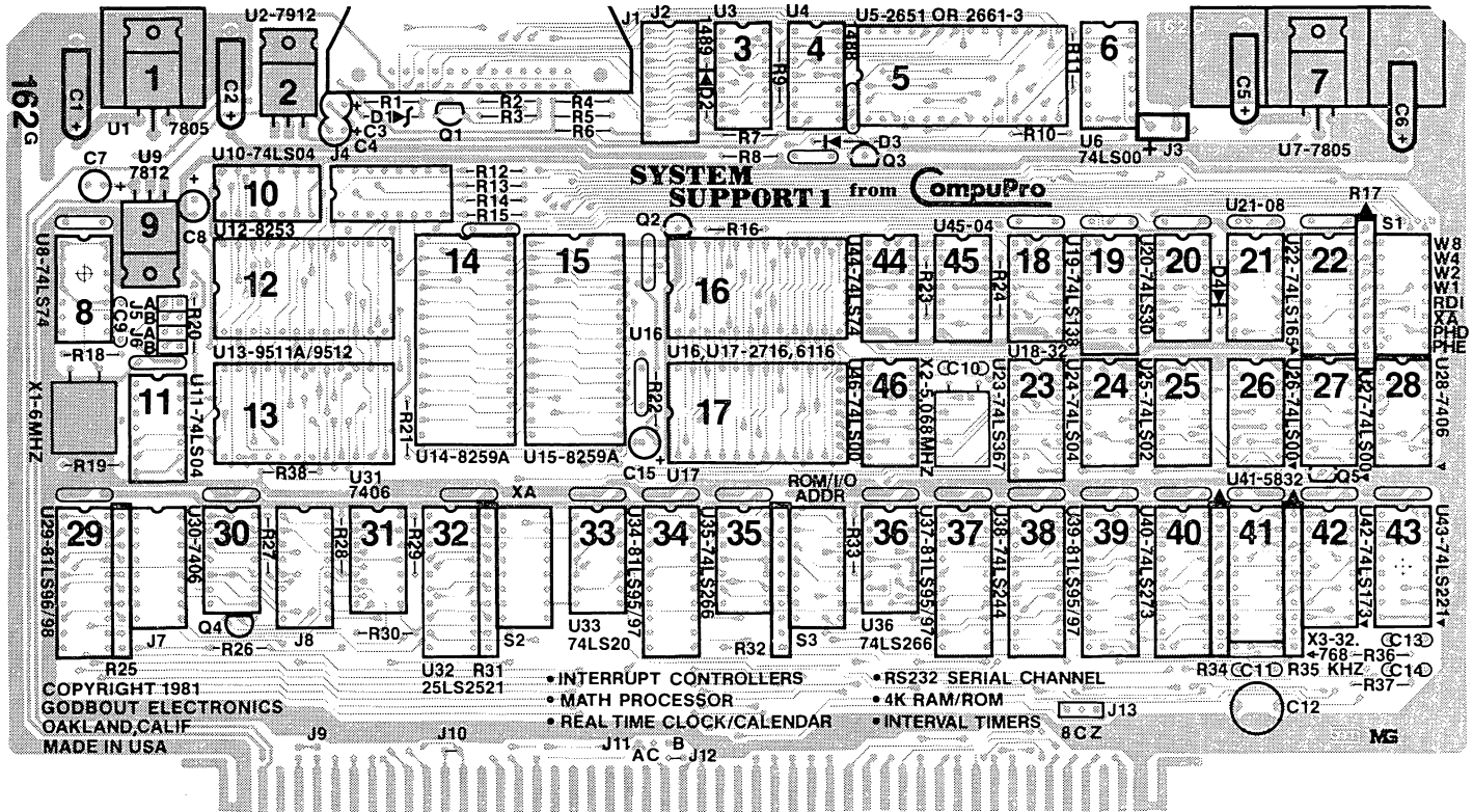
COMPONENT LAYOUT
