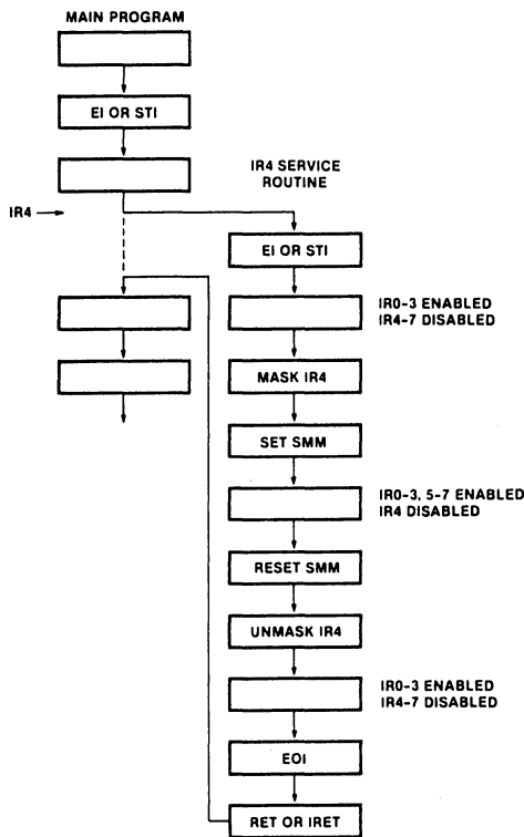
Figure 15. Special Mask Mode Example (MCS 80/85™ or MCS 88/88™)
