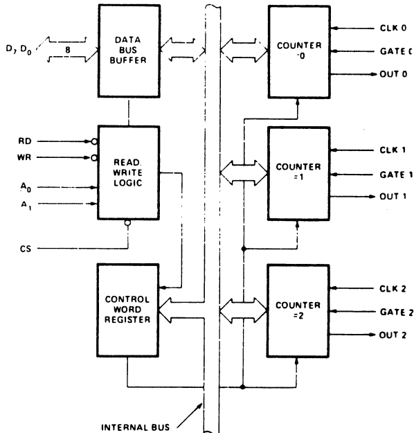
BLOCK DIAGRAM
