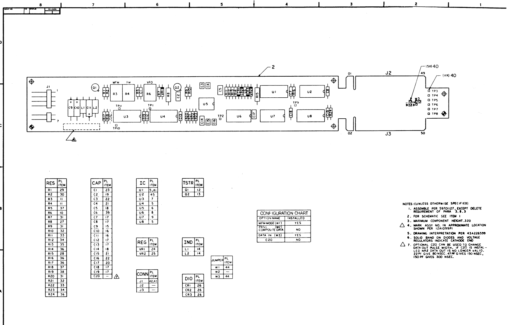
FIGURE 1-6. PWB (SHEET 1 OF 3)
