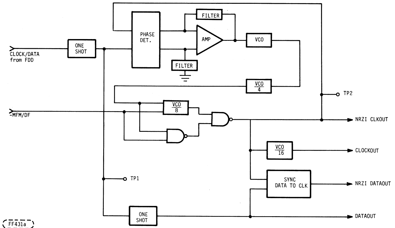
FIGURE 1-1. PLO BLOCK DIAGRAM
