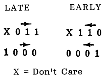
FIGURE 3-3. PEAK SHIFT WORST CASE DATA PATTERNS
