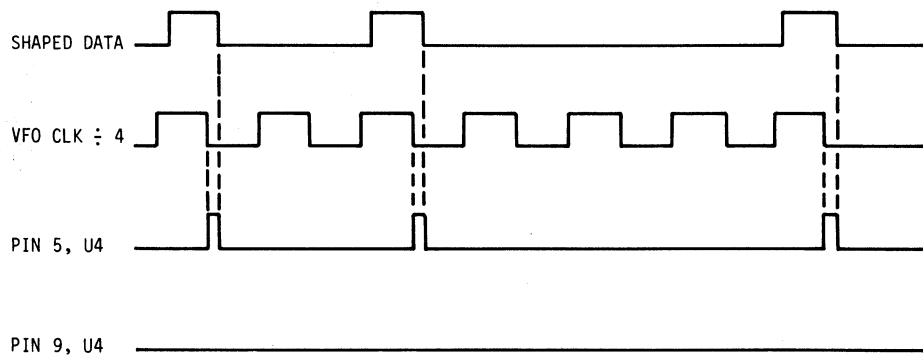
FIGURE 1-2. VFO CLK ÷ 4 LAGGING SHAPED DATA
