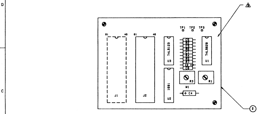
FIGURE 1-10. PWB (SHEET 1 OF 3)
