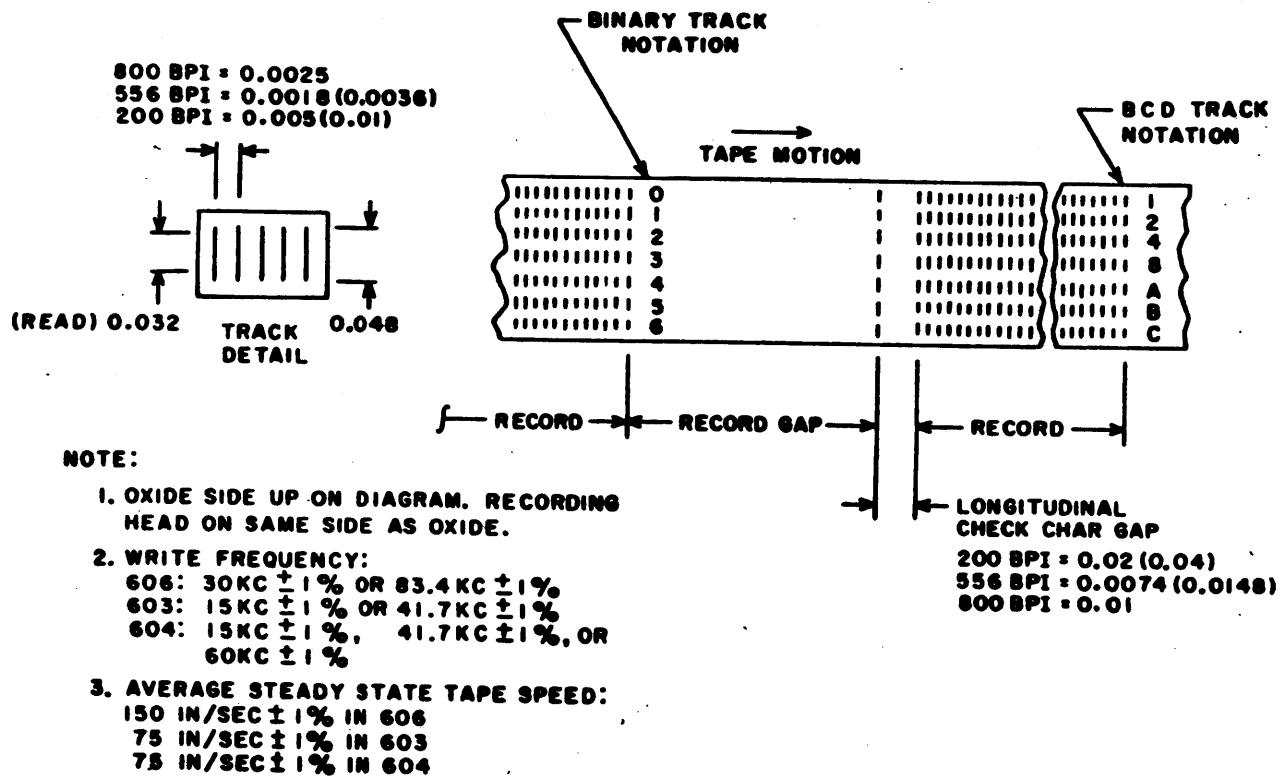
Figure A-1. Bit Assignments on Tape
