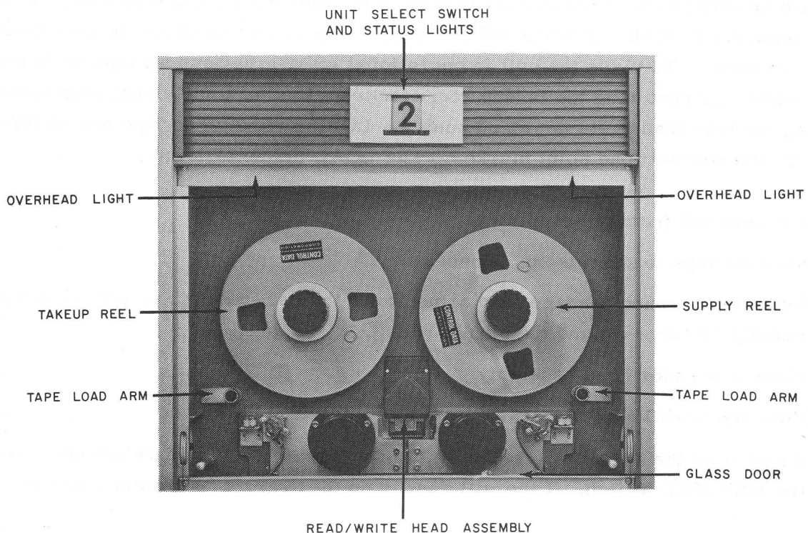
Figure A-4. Tape Load and Unload Mechanics
