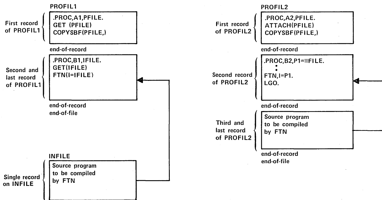
Figure 1-4-2. Procedure Access to a Data Record
