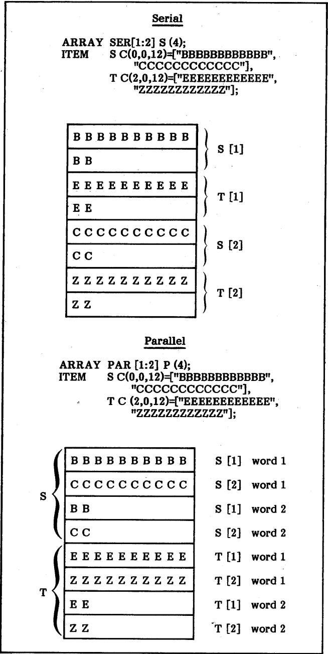
Figure 6-6. Serial and Parallel Allocation of Multiword Items
