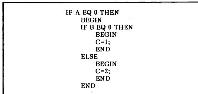
Figure 8-4. IF Statement Example B
