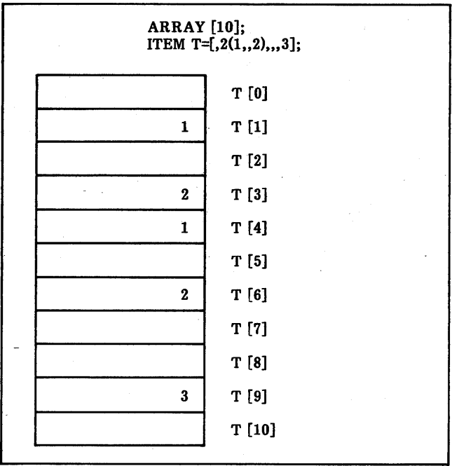
Figure 6-8. Array Presetting Example B
