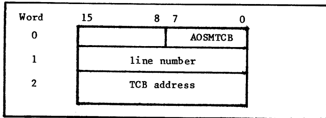
Figure 8-3. TCB Configured Worklist
