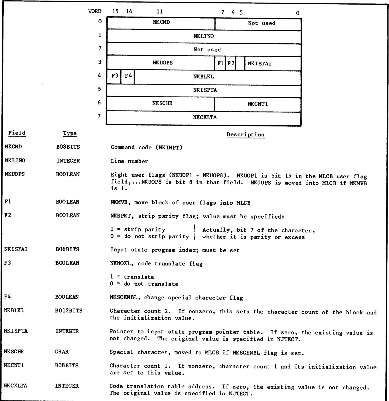
Figure 11-4. Input Command Format
