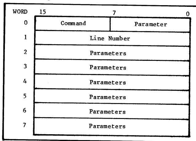
Figure 11-2. Command Packet General Format
