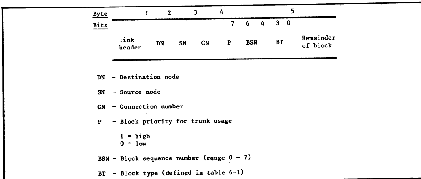
Figure 6-2. Block Header Format
