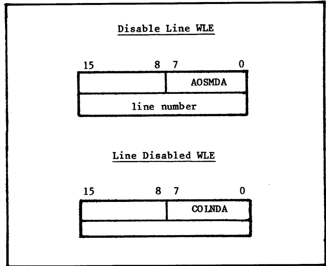
Figure 8-2. Disable Line Worklists
