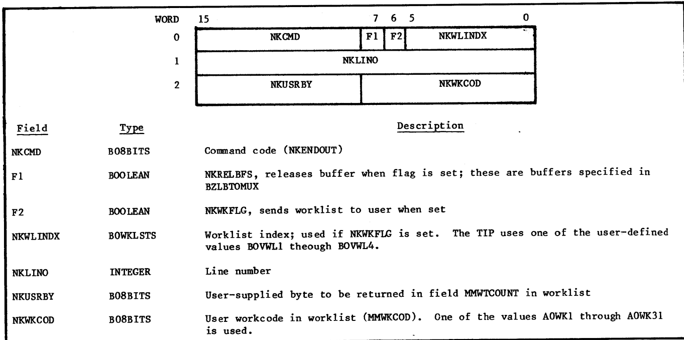
Figure 11-8. Terminate Output Command Format
