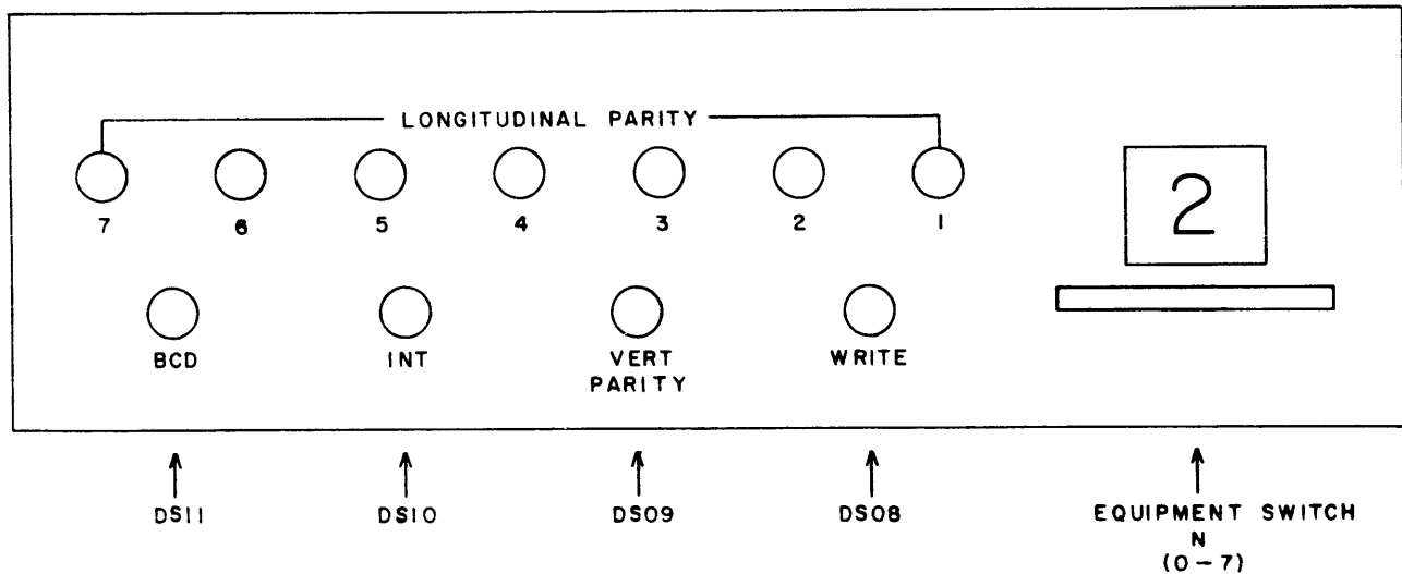
Figure 1-2 3228/3229 Control Panel
