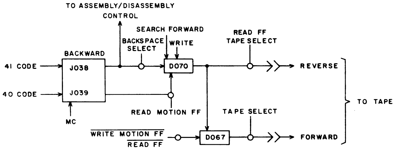
Figure 2-14. Tape Motion Signals
