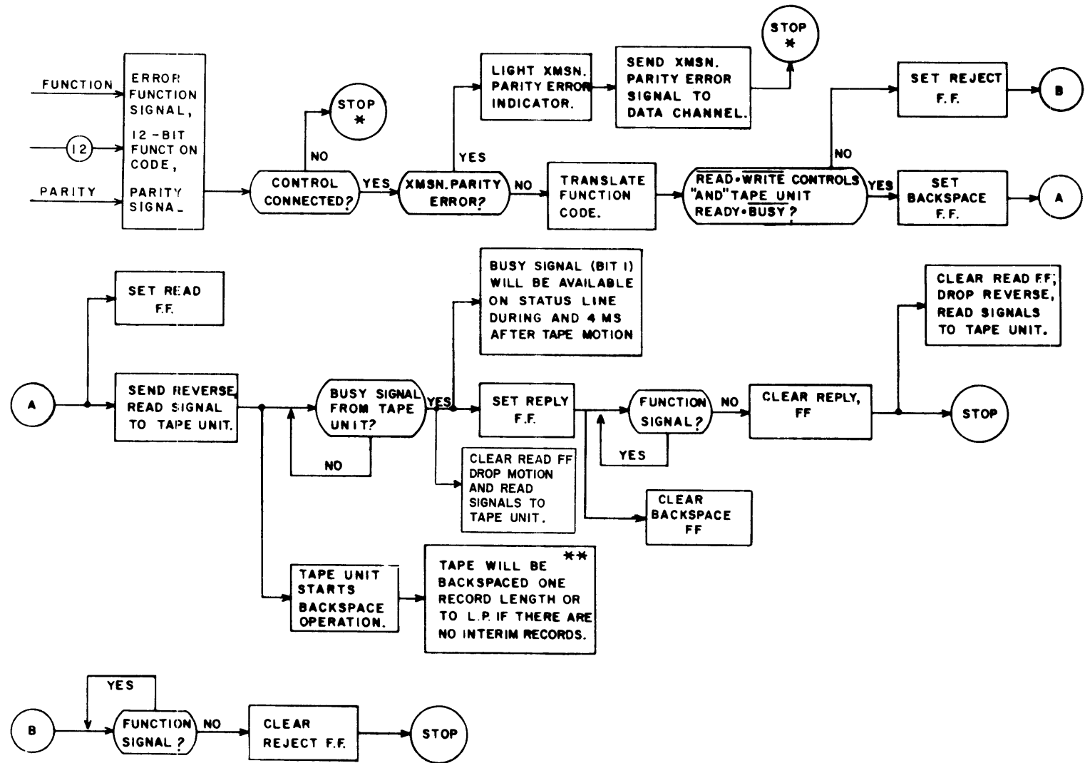
Figure 2-22. Backspace.
