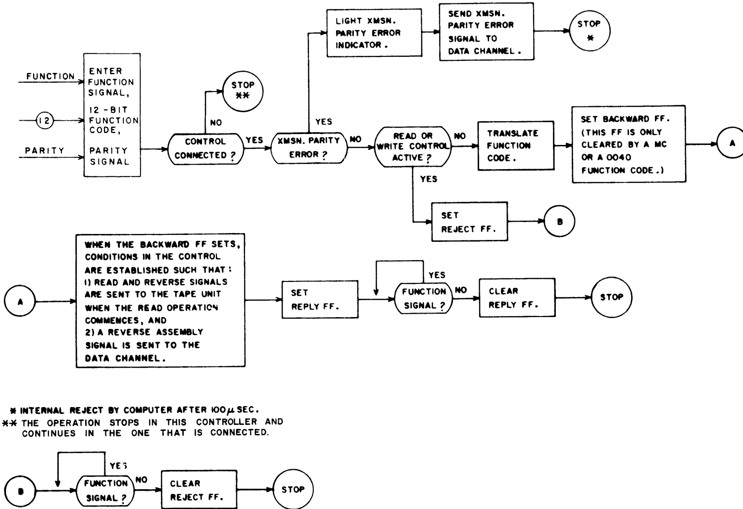
Figure 2-12. Reverse Operation
