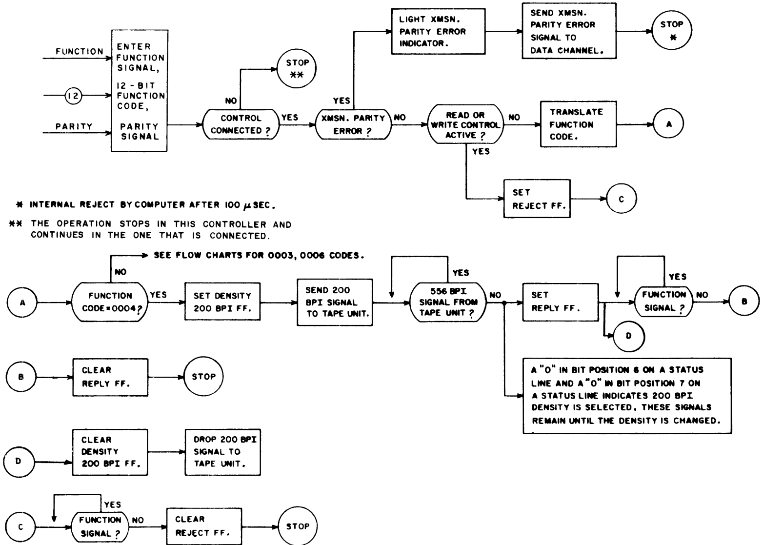
Figure 2-8. 200 BPI Operation
