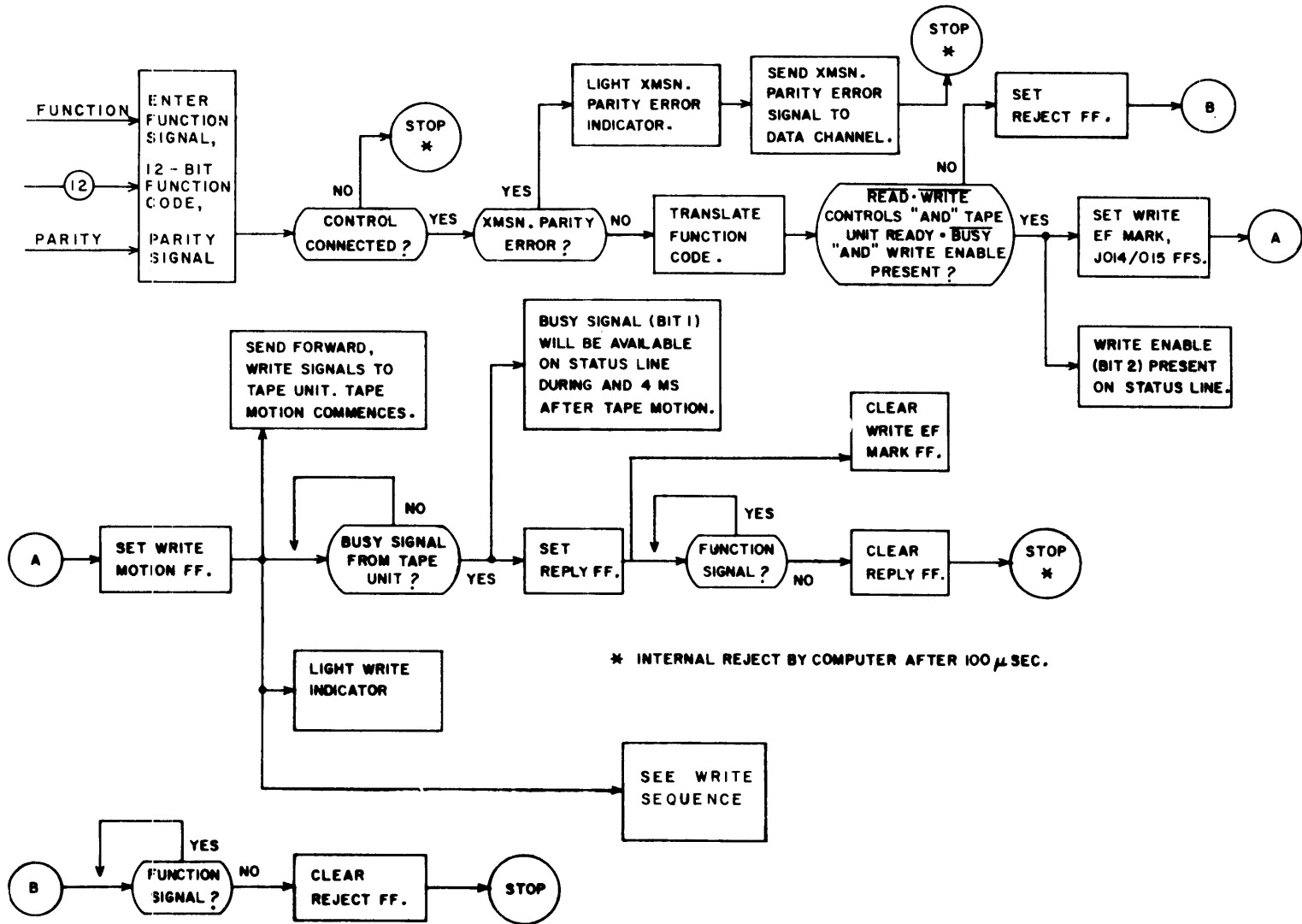
Figure 2-19. Write File Mark.
