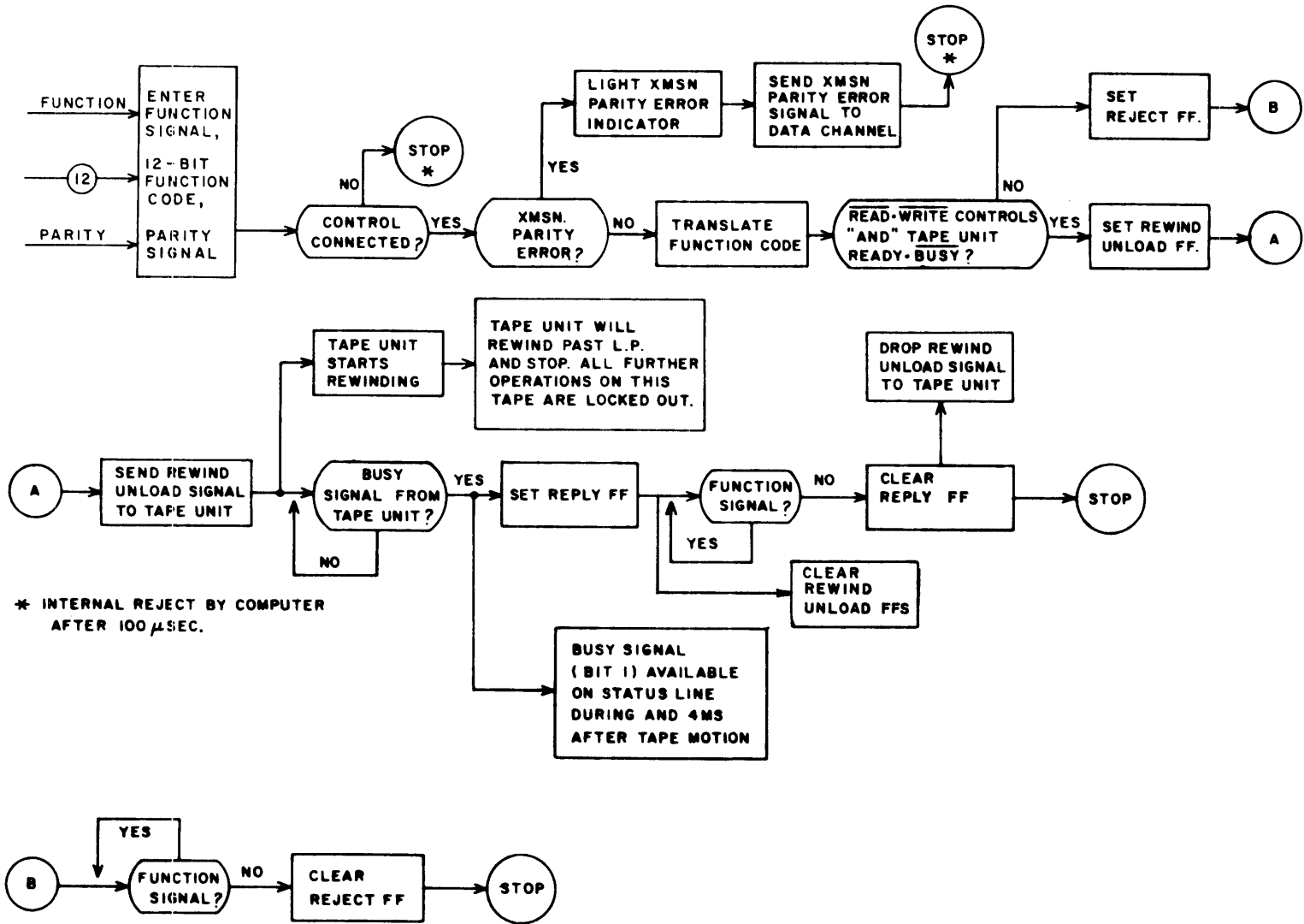
Figure 2-24. Rewind Unload.
