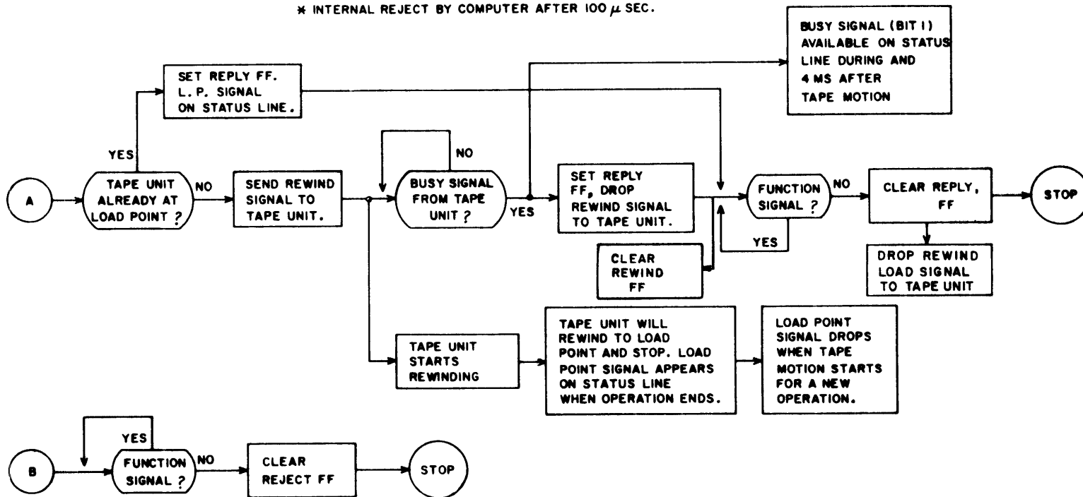
Figure 2-23. Rewind.
