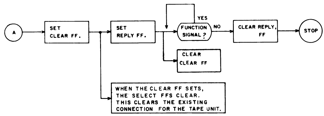
Figure 2-4. Clear Operation
