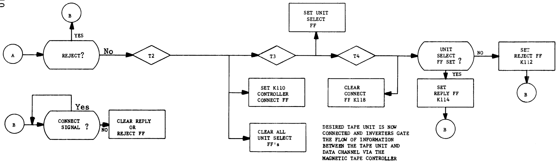
Figure 2-1. Connect Operation
