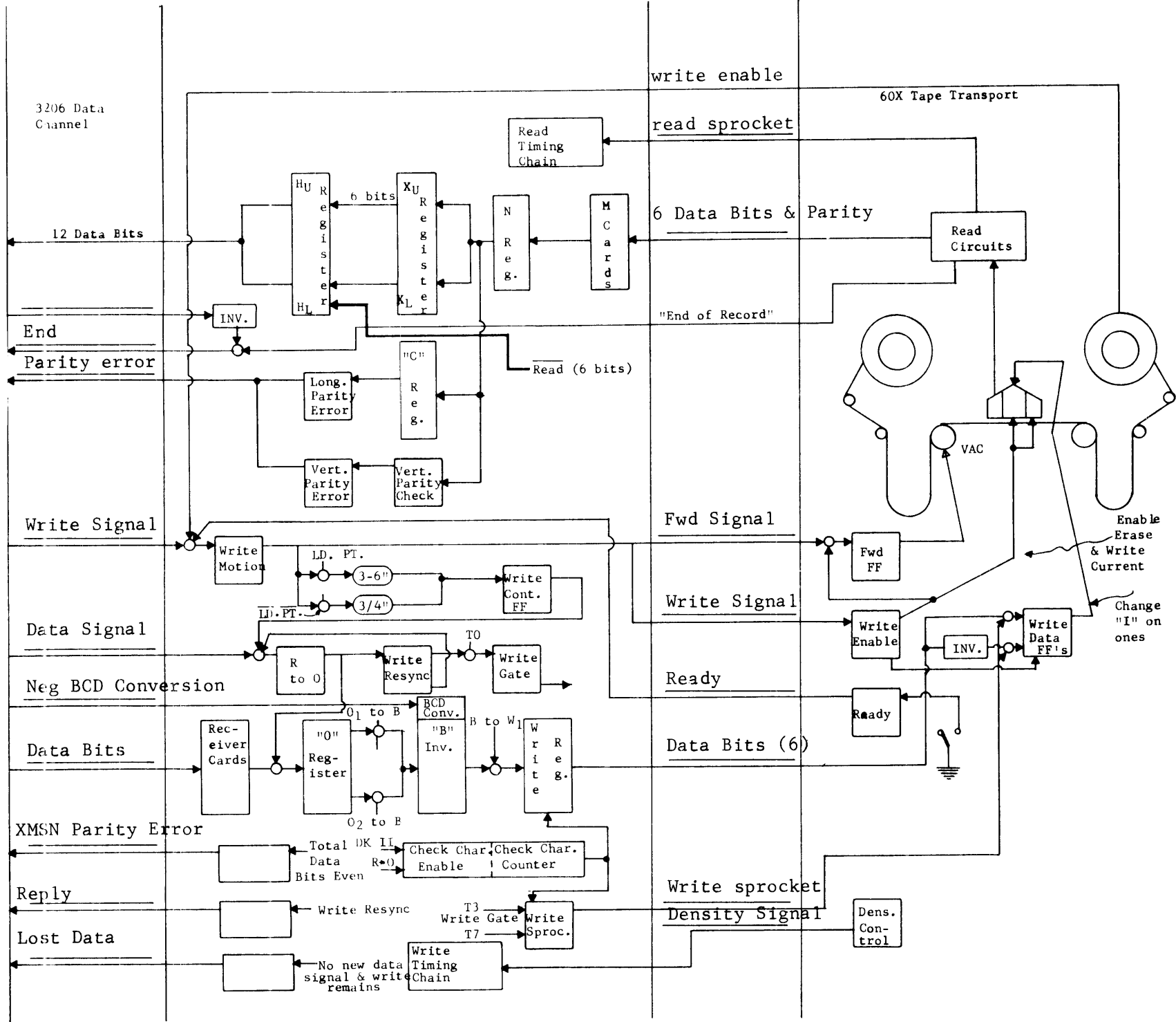
VII. WRITE OPERATION (12 AND 6 BIT MODE) I. COMPLETE THE FOLLOWING BLOCK DIAGRAM.
