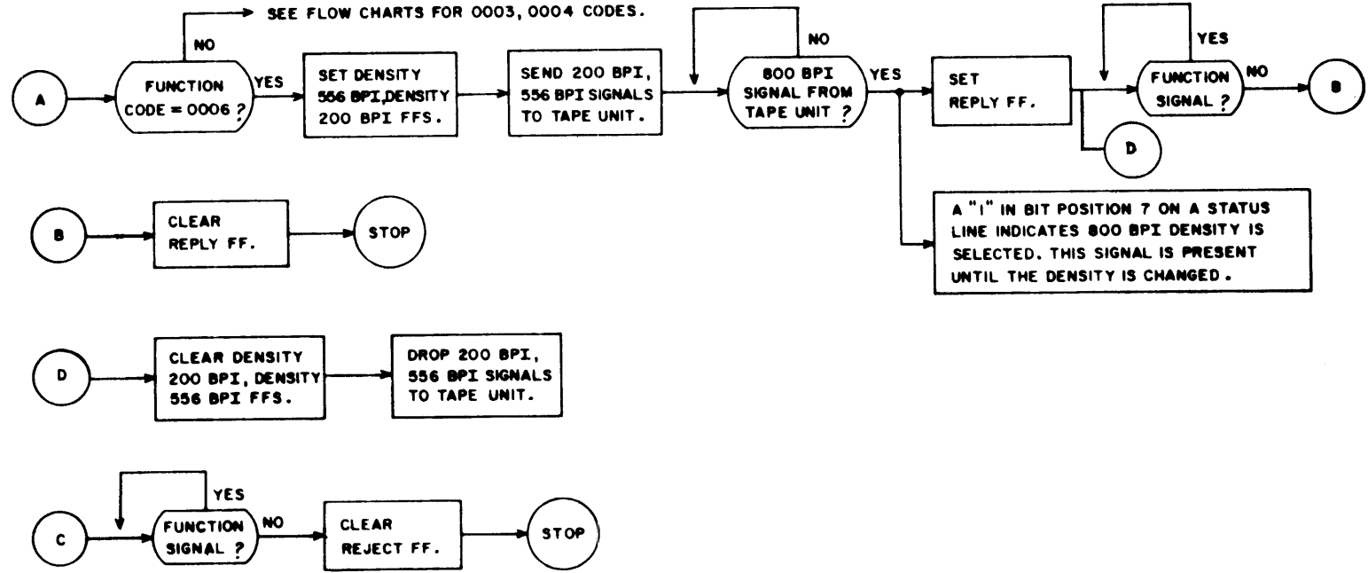
Figure 2-10. 800 BPI Operation
