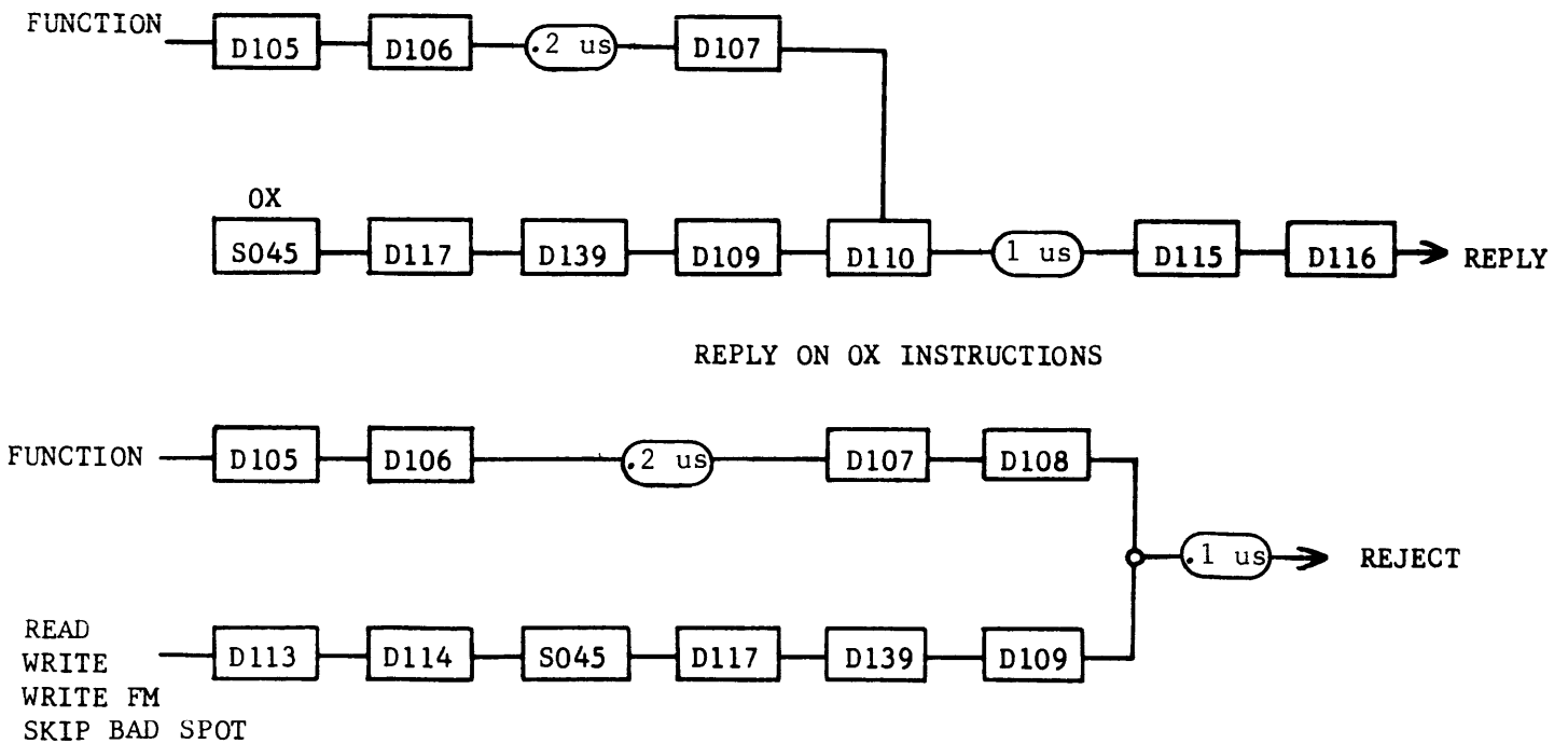
Figure 2-15. Reject on OX Instructions
