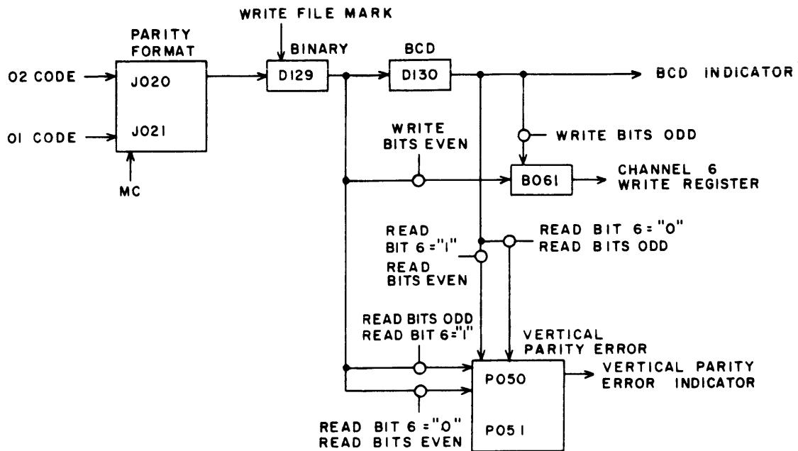
Figure 3-2-6. Parity Mode
