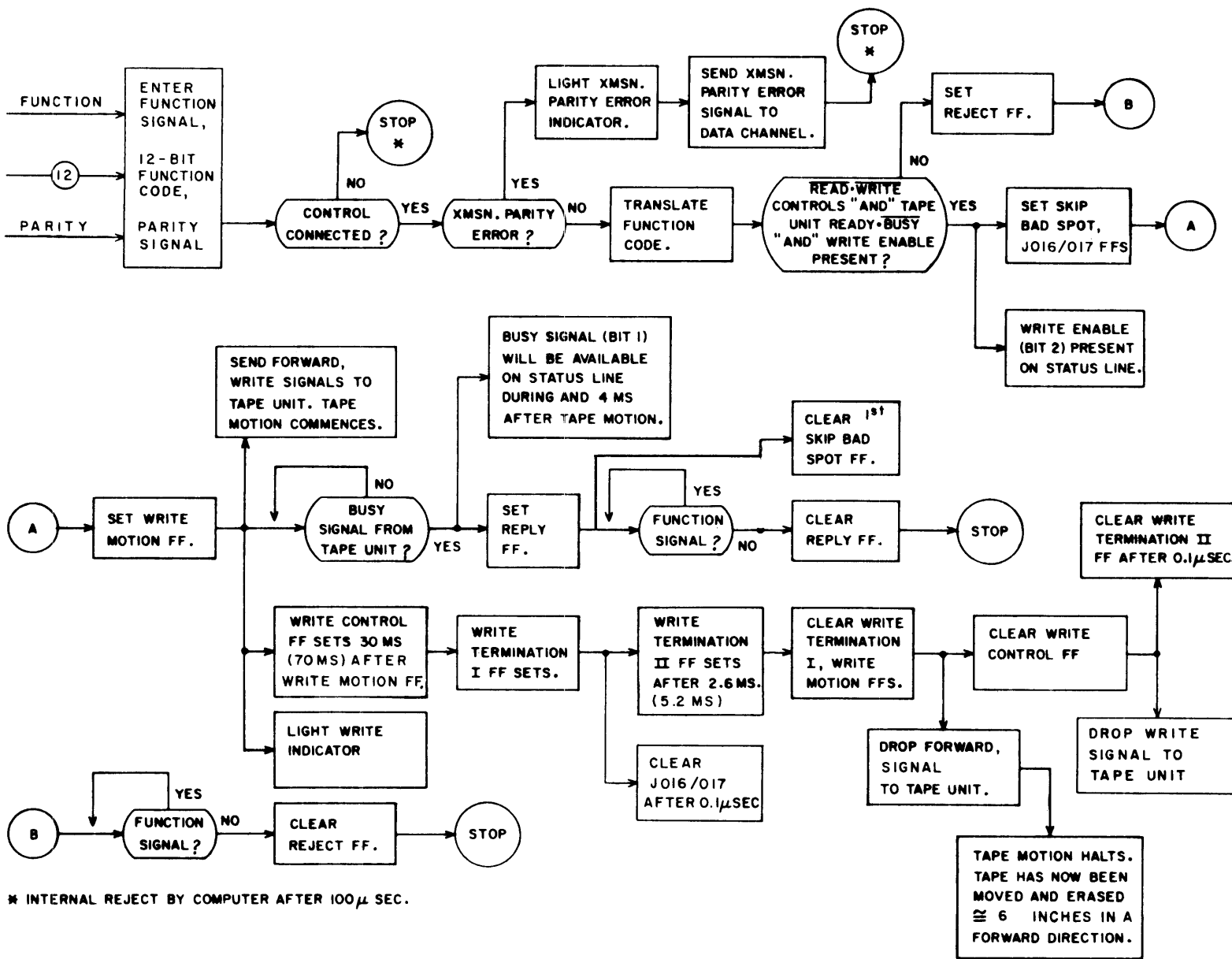
Figure 2-17. Skip Bad Spot
