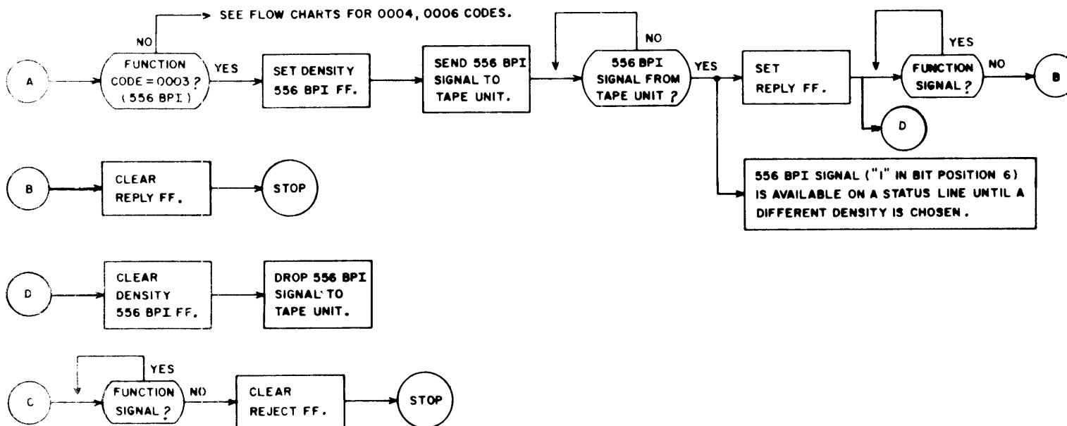
Figure 2-9. 556 BPI Operation
