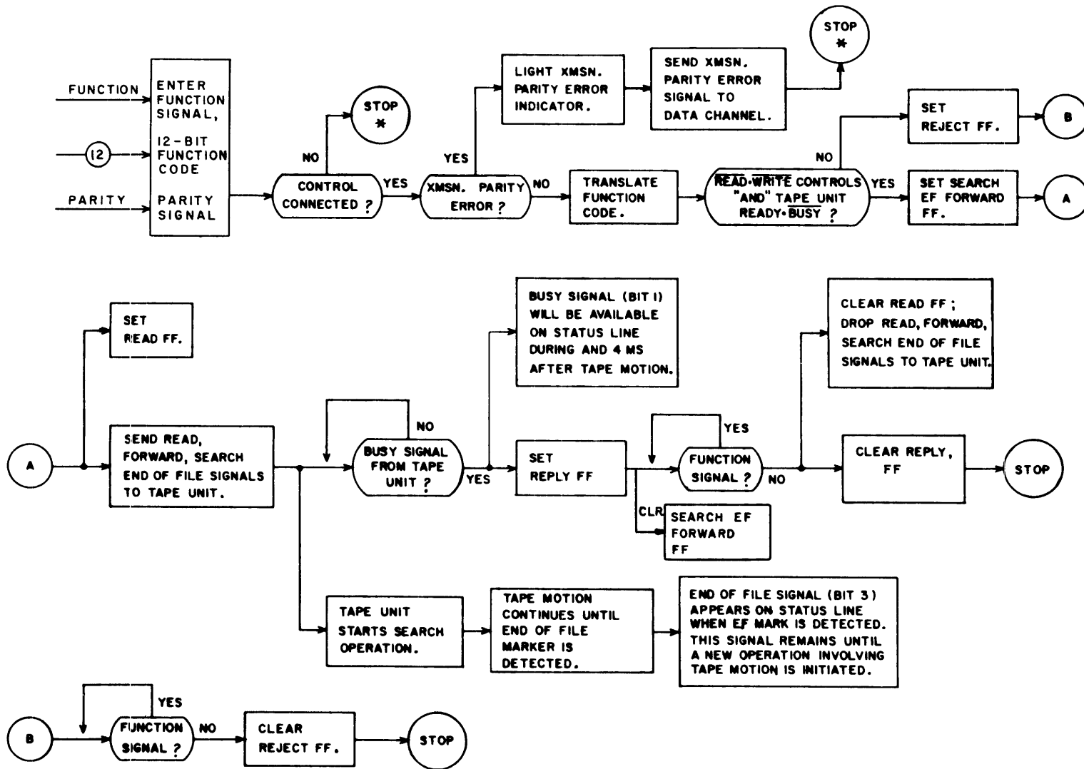
Figure 2-20. Search Forward to File Mark.
