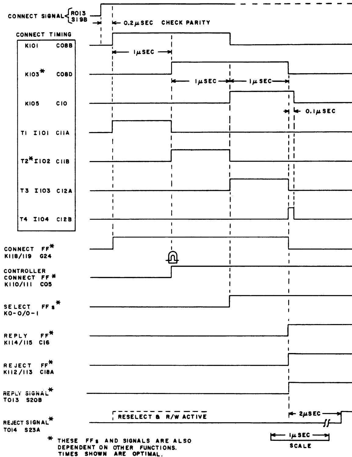
Figure 2-2. Connect Operation Timing
