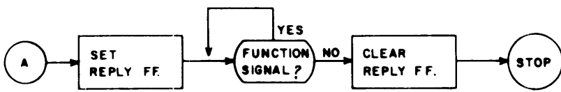
Figure 2-13. Clear Reverse Operation
