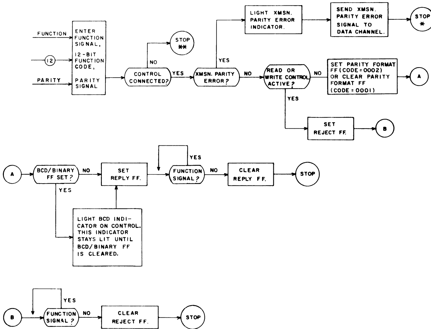
Figure 2-3. Parity Mode Operation
