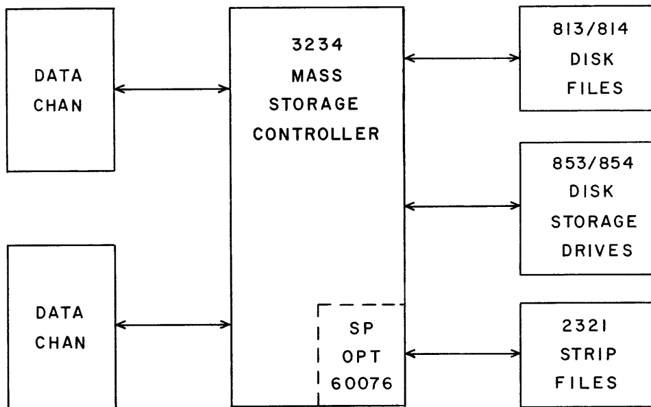
Figure C-1. Typical Configuration
