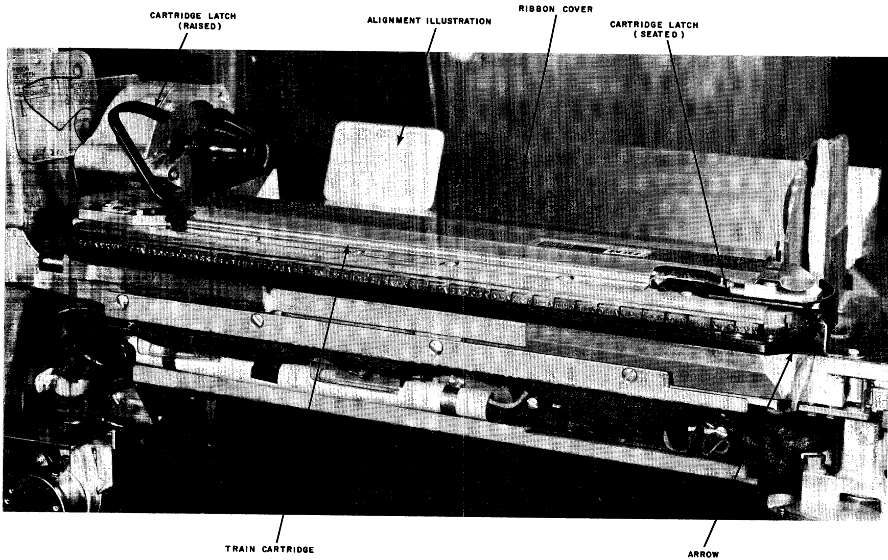
Figure D-11. Train Assembly (Mod 3 Printer)
