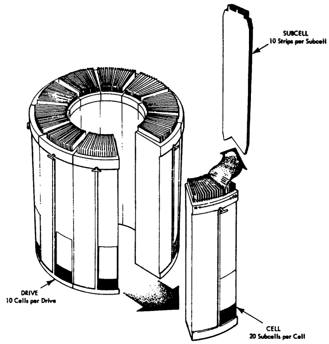
Figure C-8. Array Subdivisions
