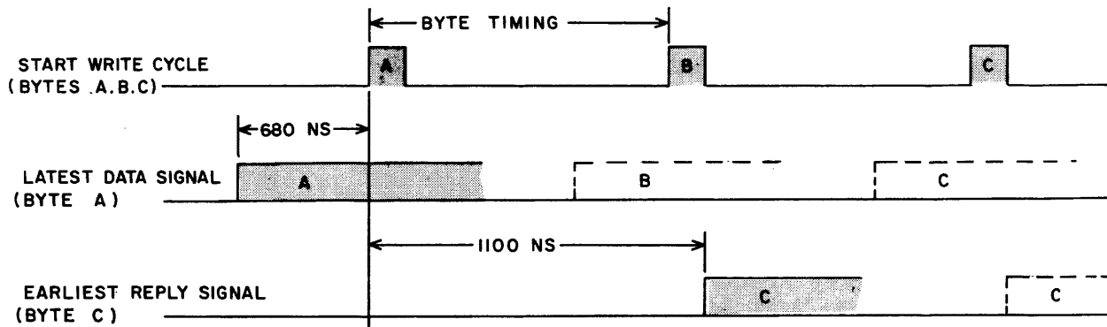
Figure A-5. Write Timing
