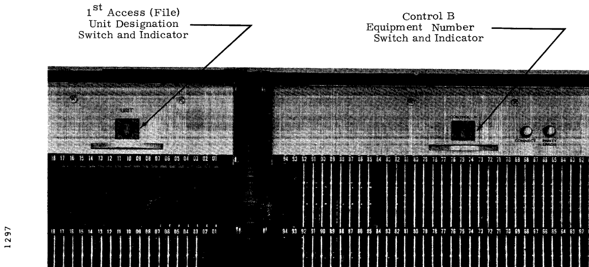
Figure B-11. Controller Switches and Indicators
