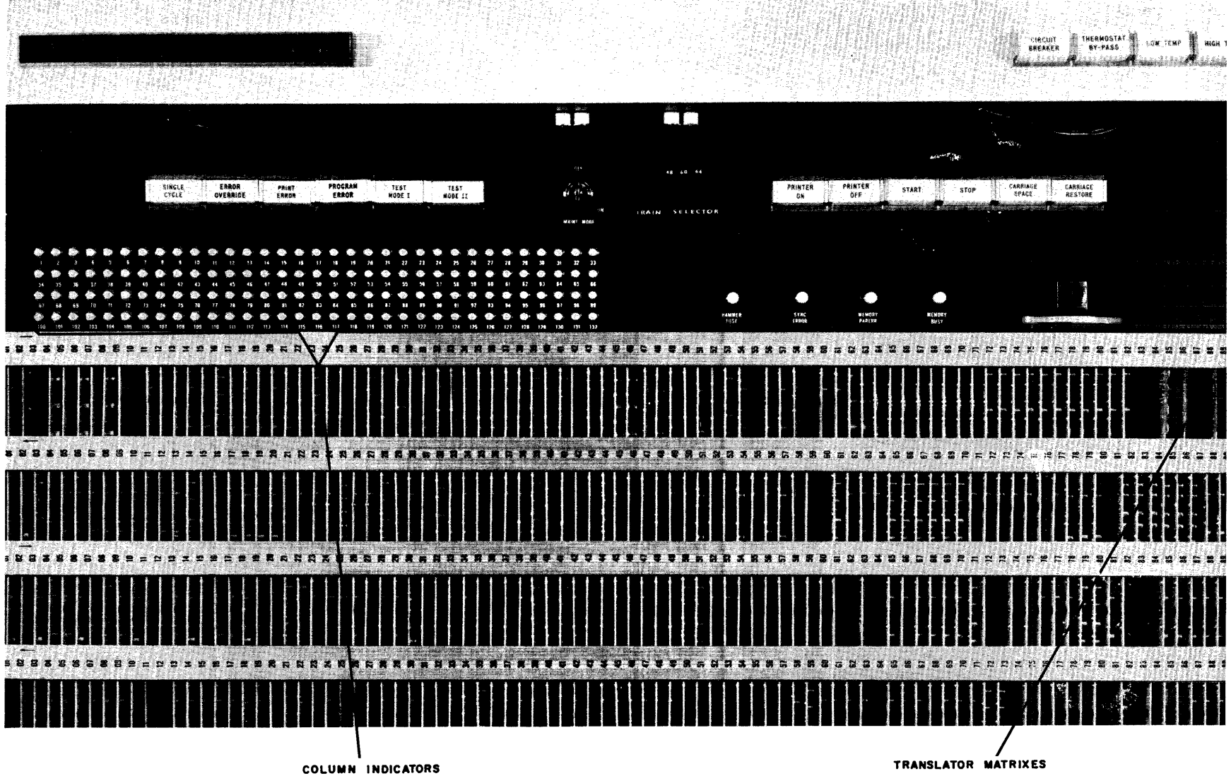
Figure D-3. 3458 Maintenance Panel
