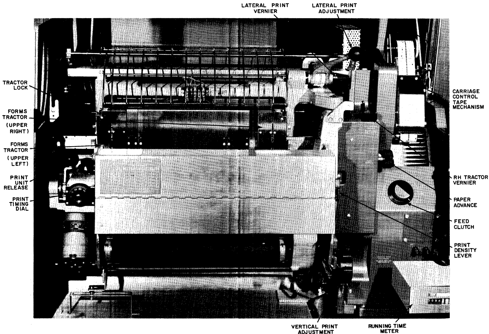
Figure D-4. 1403 Printer, Mod 2 (Front View - Cover Raised)
