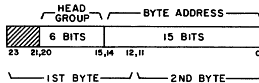
Figure A-9. 863 Drum Address Format
