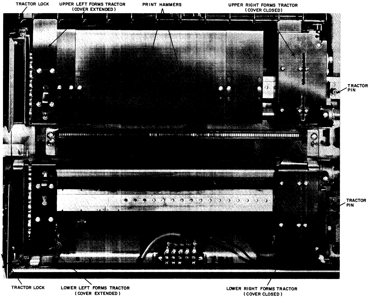
Figure D-8. Forms Tractor Mechanism (Mod 2 Printer)
