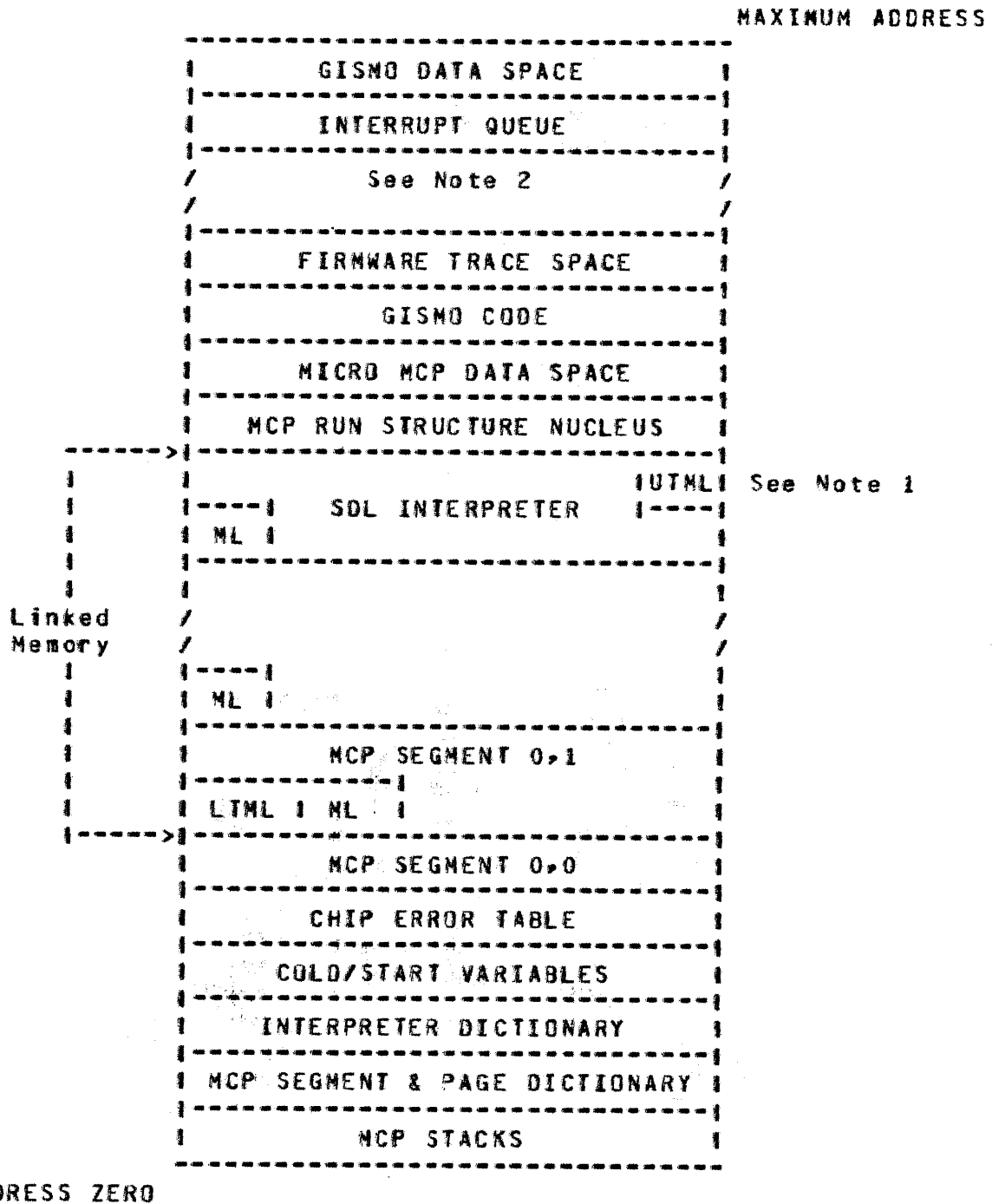
Figure 4.2 Memory Format After Initialization
