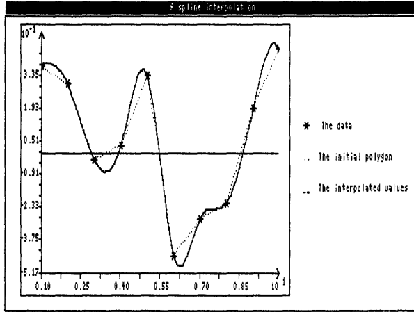
Figure 2-20 Finding a Smooth Curve with Cubic Splines (INTERP.PAS Example)
