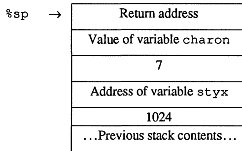
Figure 4-2. Stack contents after entry to the function call
