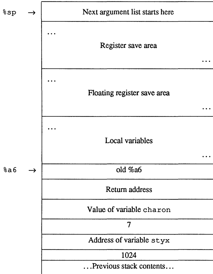
Figure 4-3. Stack contents after execution of prolog code
