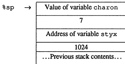
Figure 4-1. Stack contents after evaluation of function call
