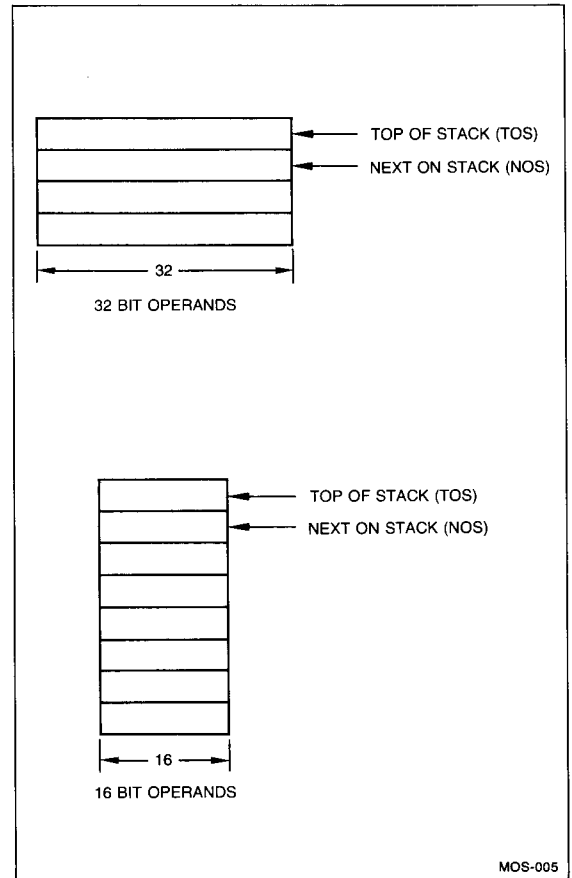
Figure 5. Stack Configurations.
