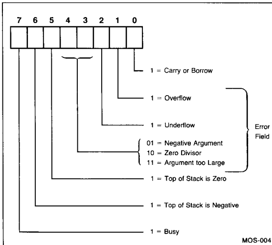
Figure 4. Status Register.
