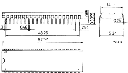
40-PIN PLASTIC DUAL IN-LINE PACKAGE
