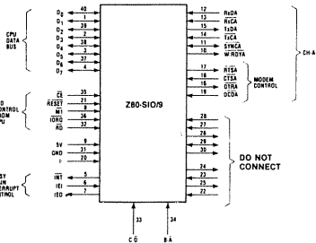
FUNCTIONAL PIN CONFIGURATION
