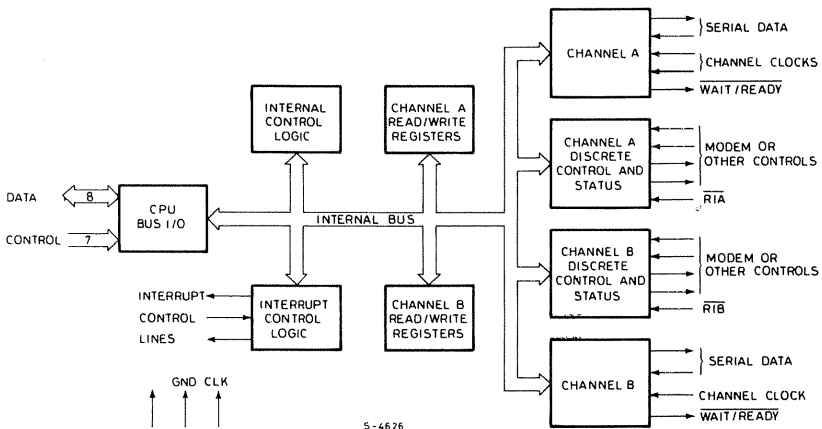
Fig. 3 - BLOCK DIAGRAM
