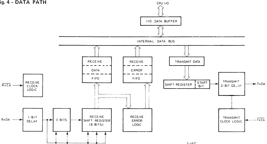
Fig. 4 - DATA PATH
