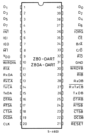
Fig. 2 - PIN ASSIGNMENTS
