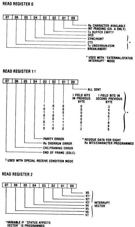
FIG. 12 — READ REGISTER BIT FUNCTIONS
