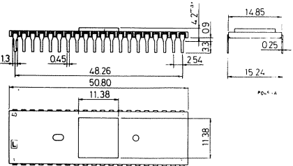
40-PIN CERAMIC DUAL IN-LINE SLAM PACKAGE
