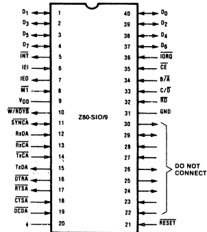
PACKAGE CONFIGURATION
