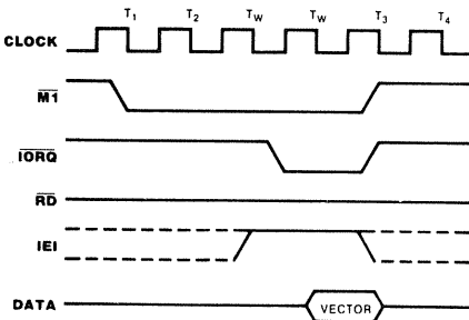
Fig. 5c - INTERRUPT ACKNOWLEDGE CYCLE
