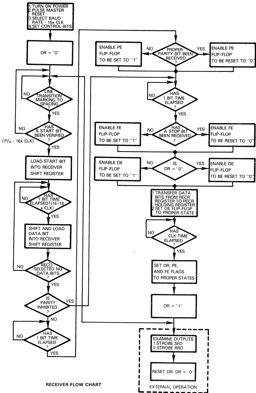
Figure 4-44 Operations Flow Chart For \mu PD369 Asynchronous Serial I/O Operations (Continued)
