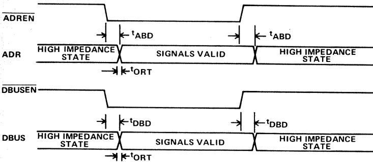
TRI-STATE BUS TIMING
