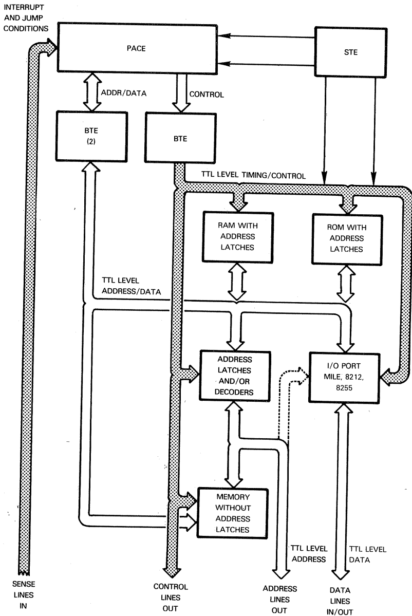
Figure 14-1. A National Semiconductor PACE Microcomputer System
