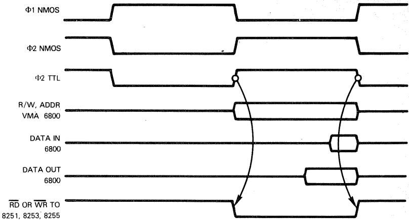
Figure 8-12. Timing For 8080A Support Devices Used With An MC6800 CPU
