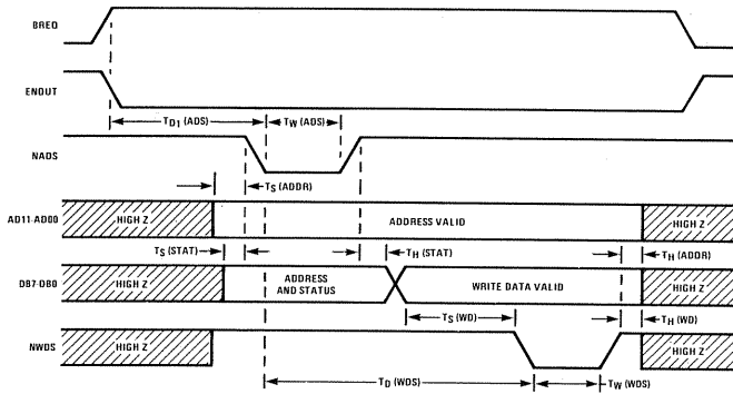
FIGURE 6. SC/MP Data Output Timing
