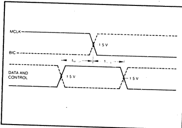
Setup and Hold Times
