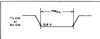
FIGURE 1 – CLOCK PULSE WIDTH, LOW-STATE
