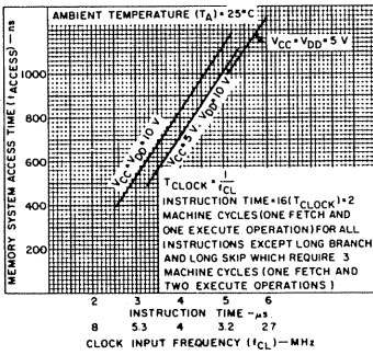
Typical instruction time vs. memory system access time.
