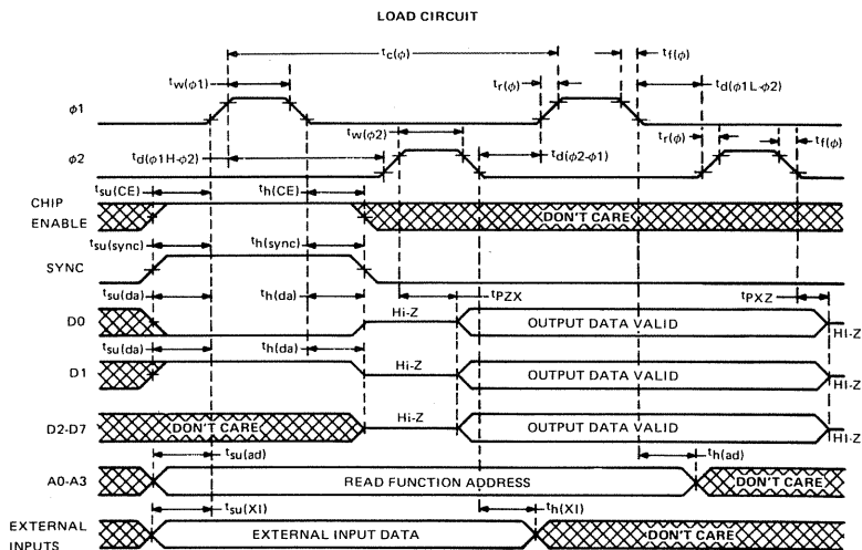
FIGURE 6—READ CYCLE TIMING
