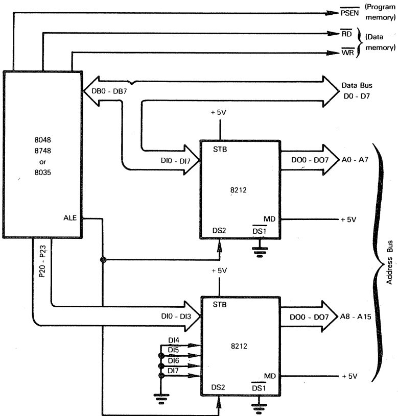
Figure 6-10. Demultiplexing DB0 - DB7 To Create Separate Address And Data Busses
