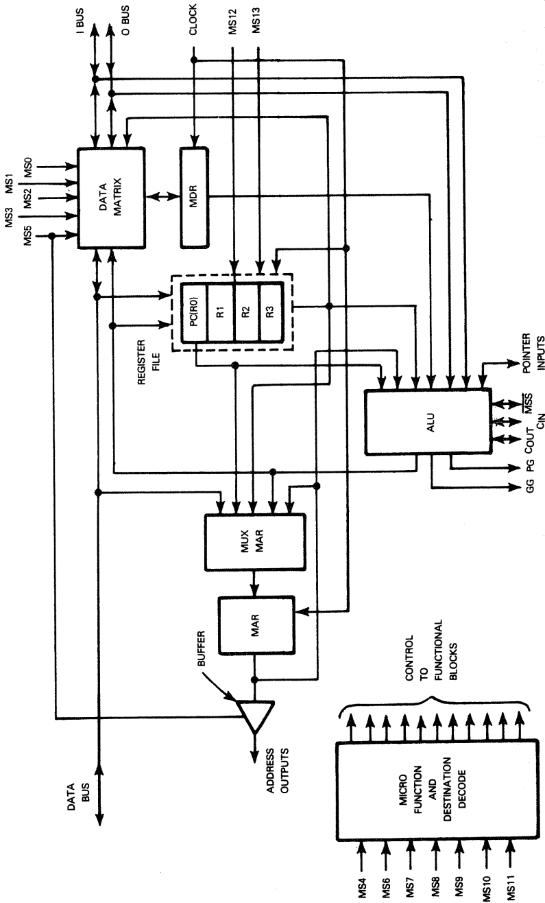
Figure 19-3. MC10803 Memory Interface Device Block Diagram
