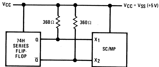
External Clock Generation
