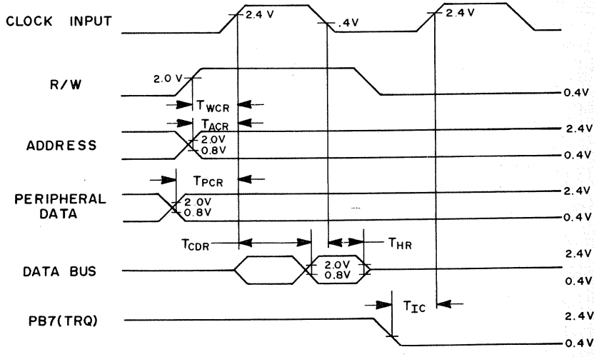
READ TIMING CHARACTERISTICS
