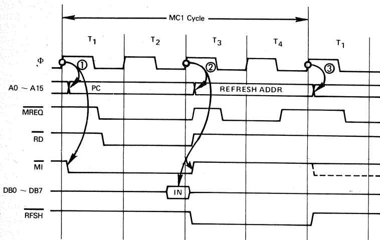
Figure 7-5. Z80 Instruction Fetch Sequence.
