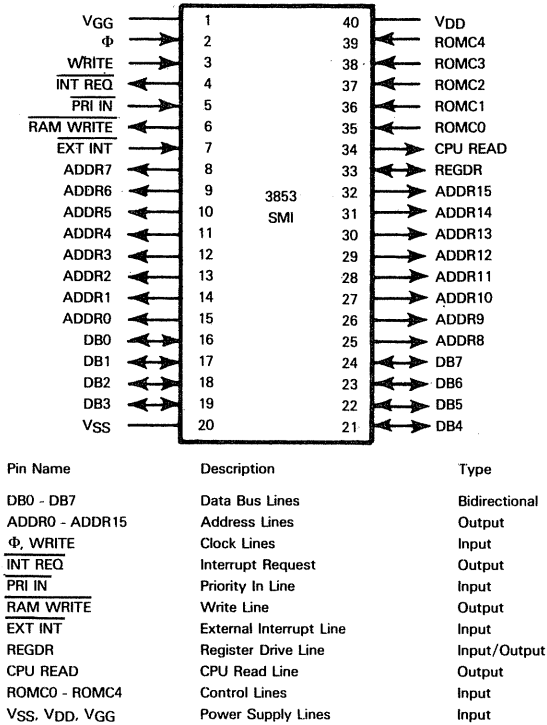
Figure 2-13. 3853 SMI Signals And Pin Assignments
