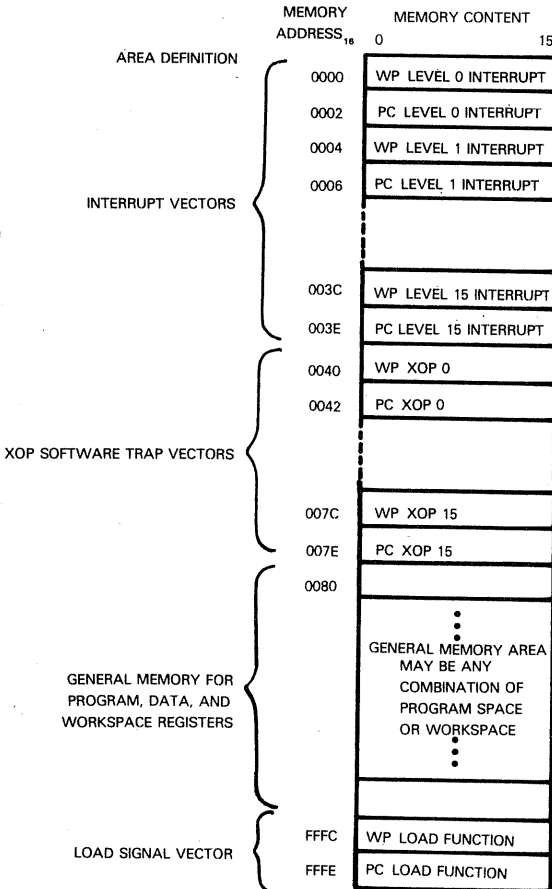
Figure 16-3 TMS9900 Memory Map
