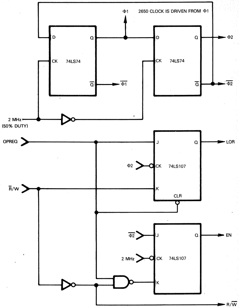
Figure 10-11. Synchronization Circuits In A 2650 — MC68XX Interface
