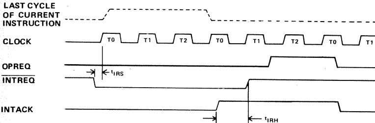
INTERRUPT TIMING
