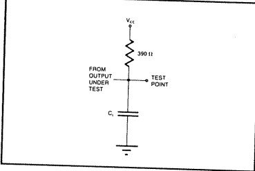
Load Circuit for Open Collector Outputs
