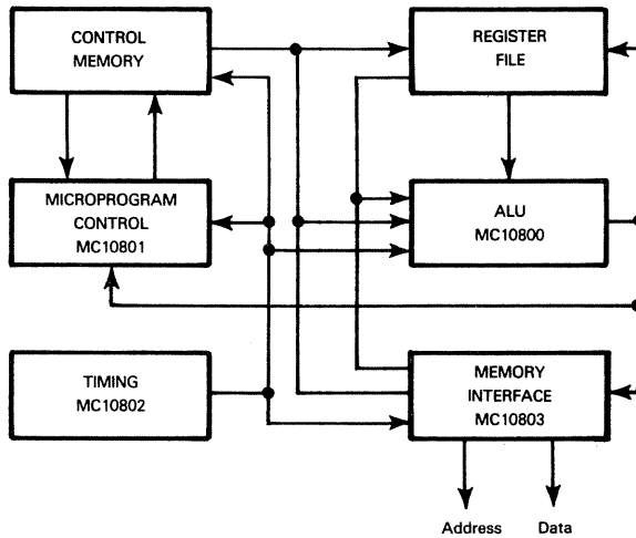
Figure 19-1. MC10800 Series Devices In A Central Processing Unit Configuration
