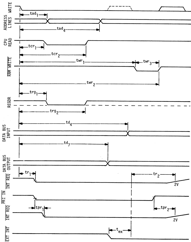
3853 Signal Timing
