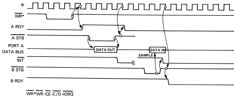
Figure 7-20 Port A, Mode 2 (Bidirectional) Timing
