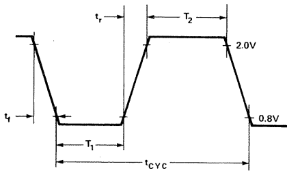
CLOCK SPECIFICATION FOR 8355.
