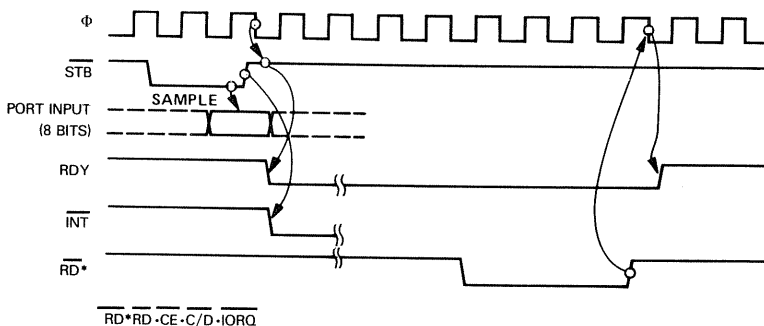
Figure 7-19. Mode 1 (Input) Timing
