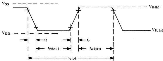
EXTERNALLY DRIVEN CLOCK INPUT WAVEFORM
