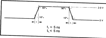
Data Delay Times
