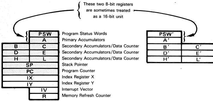
Figure 7-3 Z80 Programmable Registers
