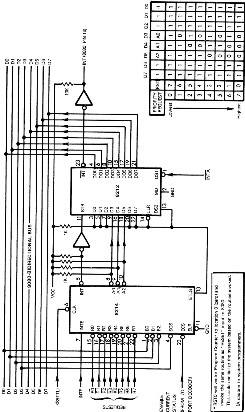
Figure 4-58. Generation Of The Restart Instruction Code Following An Interrupt. For An 8080A Microcomputer System
