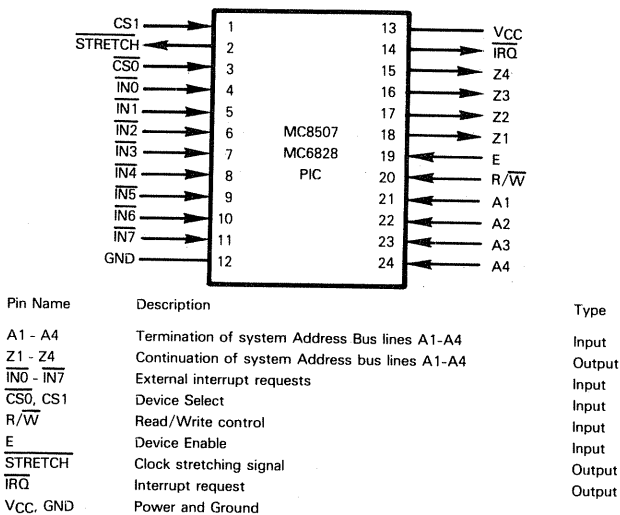
Figure 8-29. MC6828 Signals And Pin Assignments
