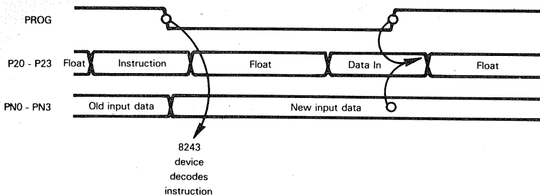
Figure 6-20. Timing For Data Input From An 8243 Port
