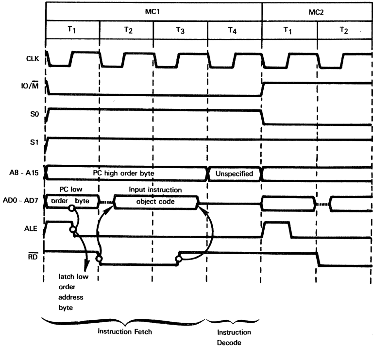
Figure 5-4. A Four Clock Period Instruction Fetch Machine Cycle
