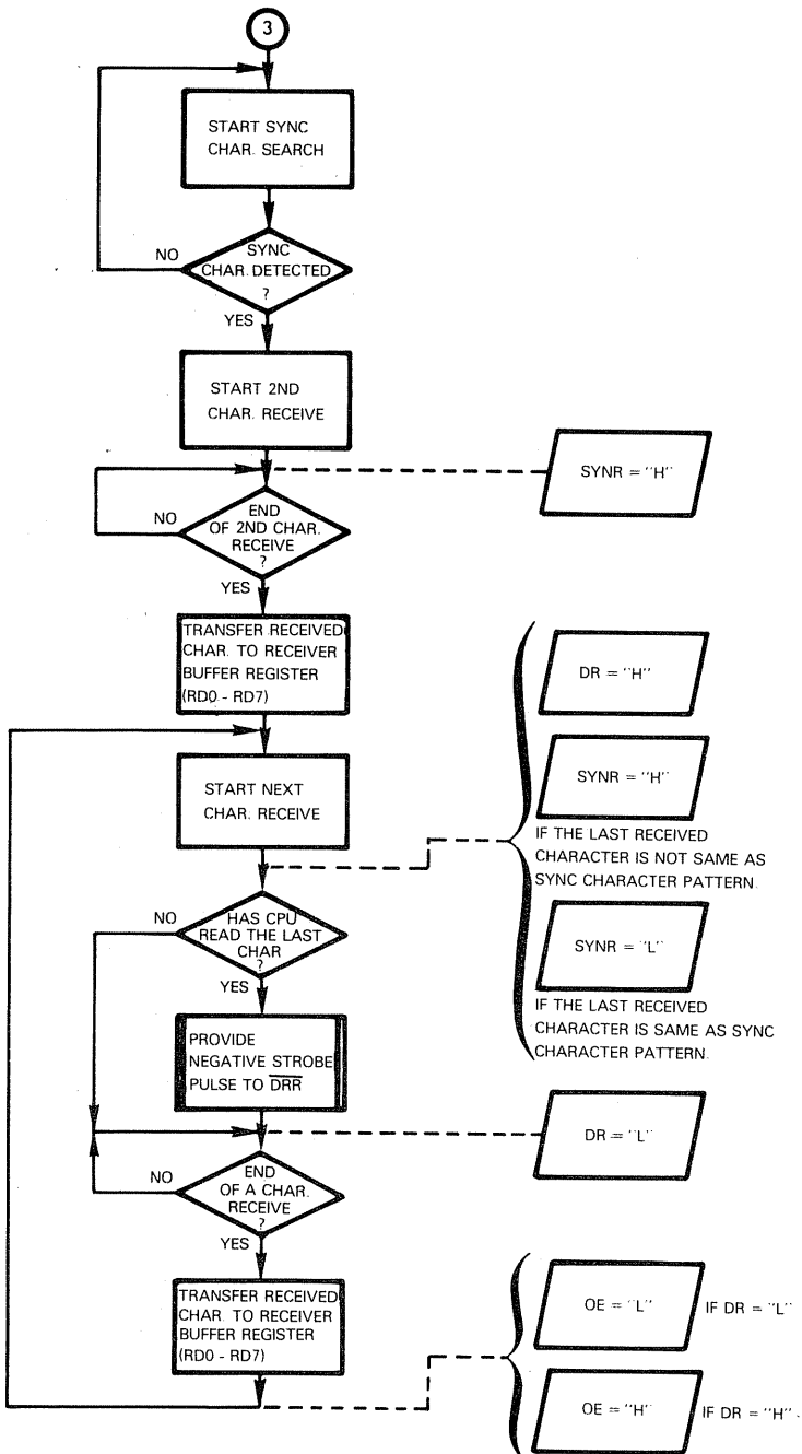
Figure 4-40. Standard Synchronous Receiving Operations Flowchart
