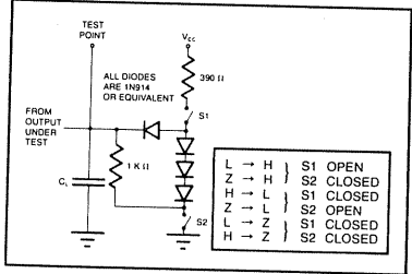
Load Circuit for Tri-state Outputs
