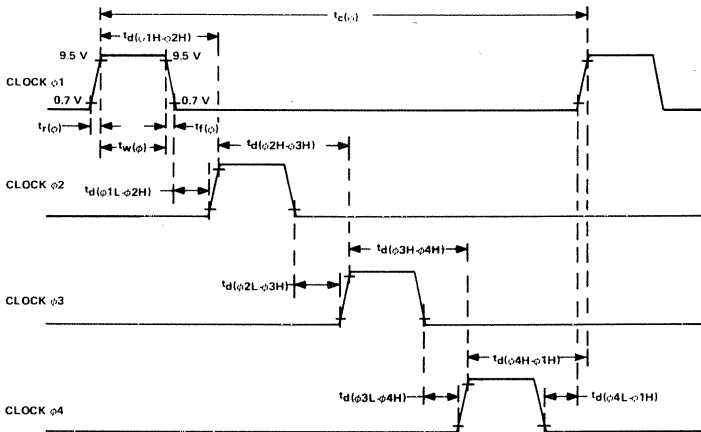
FIGURE 12 – CLOCK TIMING
