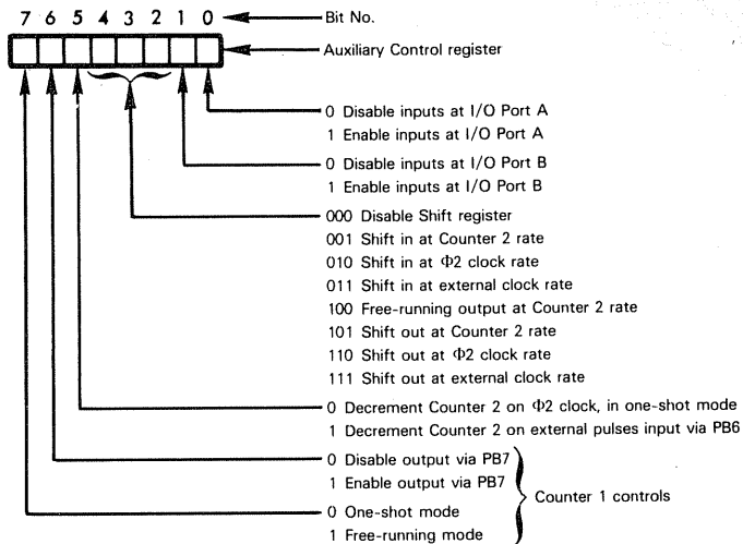
Figure 9-14. Auxiliary Control Register Bit Assignments
