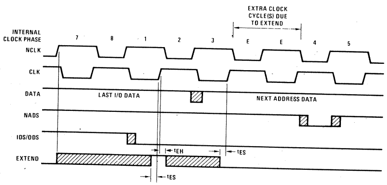
FIGURE 10. Suspend I/O Signal Timing
