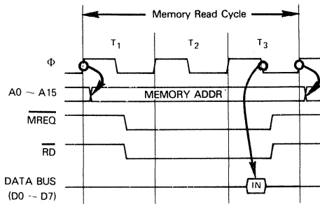
Figure 7-6. Z80 Memory Read Timing
