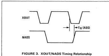
FIGURE 3. XOUT/NADS Timing Relationship
