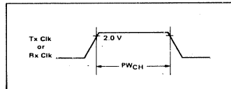
FIGURE 2 – CLOCK PULSE WIDTH, HIGH-STATE
