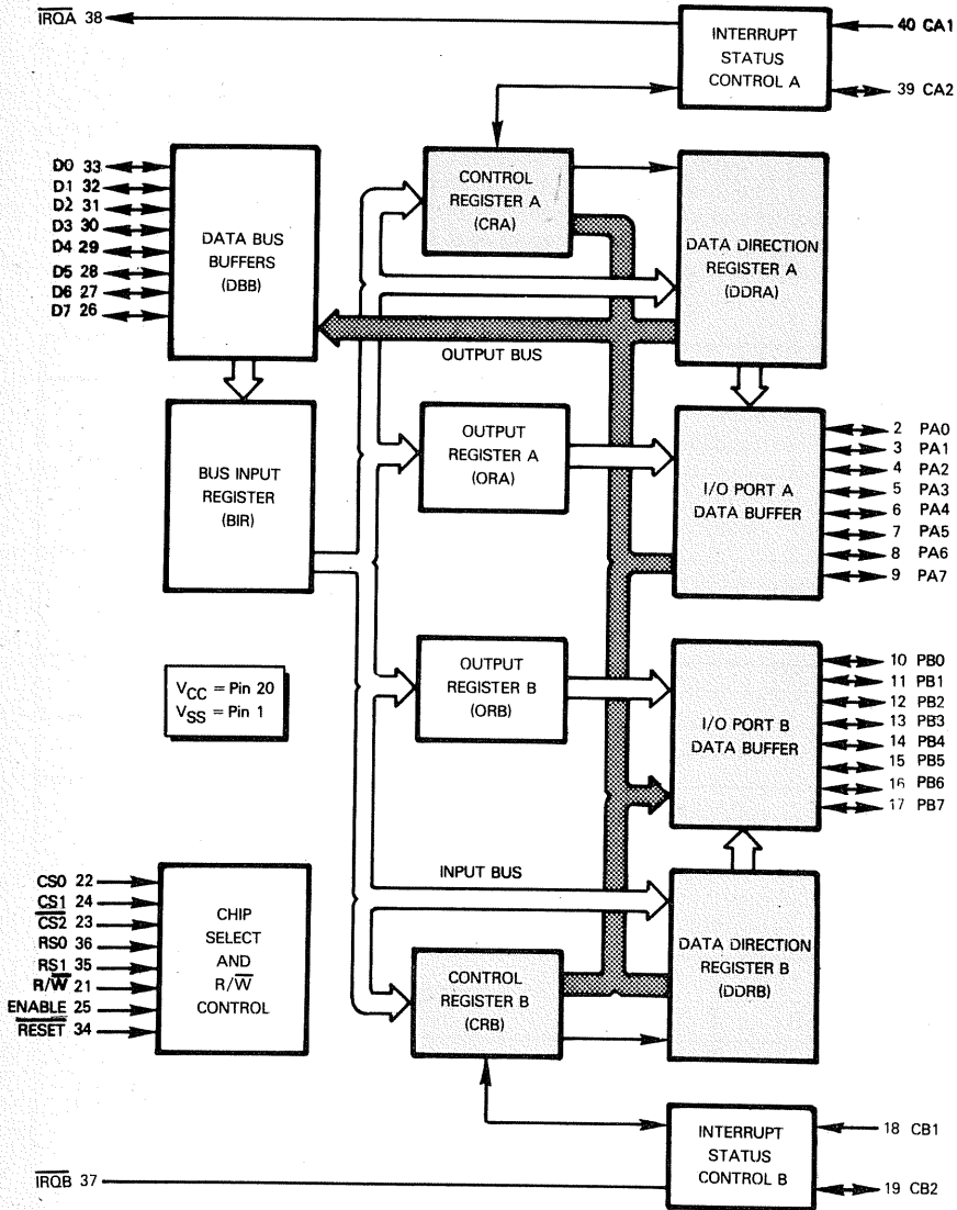
Figure 8-21. Functional Block Diagram For The MC6820 PIA
