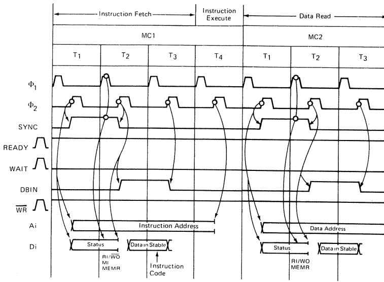
Figure 4-15. Signal Sequences And Timing For Instructions: LDAX, MOV REG M, ADI, ACI, SUI, SBI, ANI, XRI, ORI, CPI, MVI R, ADD M, ADC M, SUB M, SBB M, ANA M, XRA M, ORA M, CMP M
