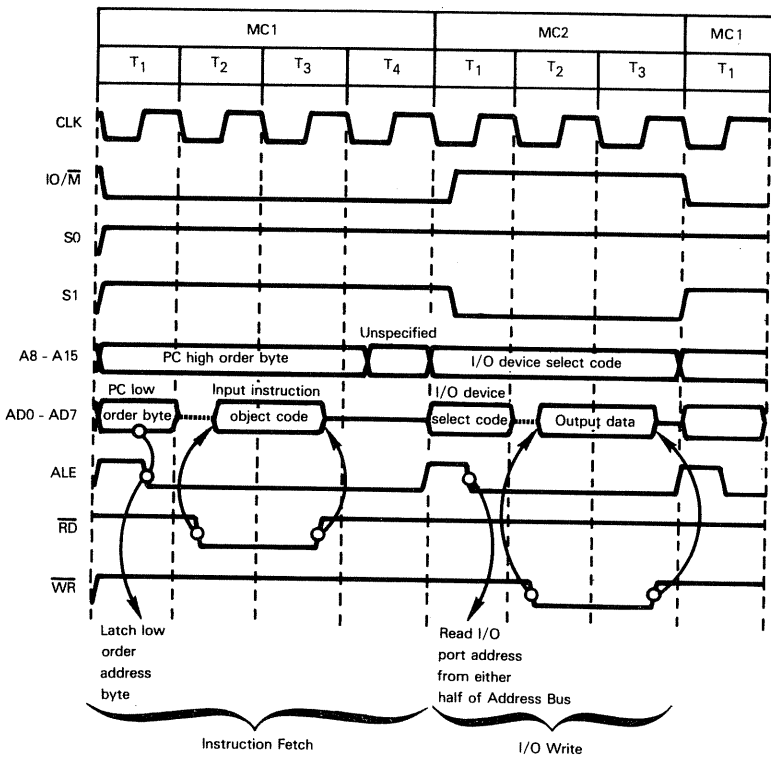
Figure 5-9. An I/O Write Machine Cycle Following An Instruction Fetch
