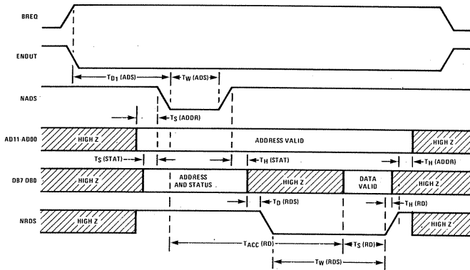
FIGURE 5. SC/MP Data Input Timing
