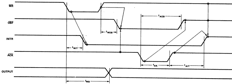
Mode 1 (Strobed Output)
