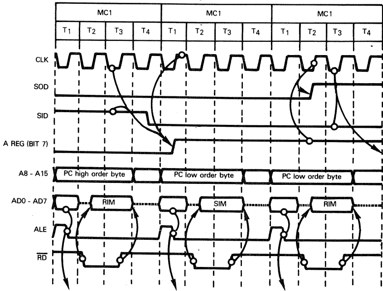
Figure 5-12. A RIM Instruction Followed By A SIM Instruction
