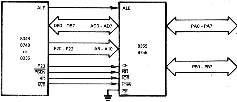
Figure 6-9. An 8048-8355 Configuration
