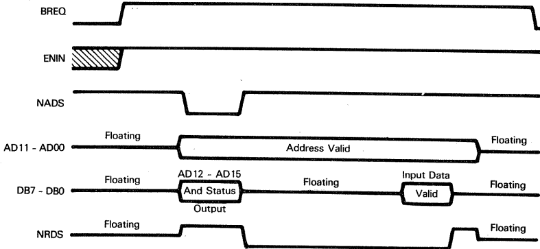
Figure 3-5. SC/MP Data Input Cycle
