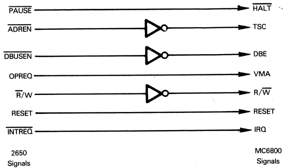
Figure 10-5. 2650 — MC6800 Signal Equivalents
