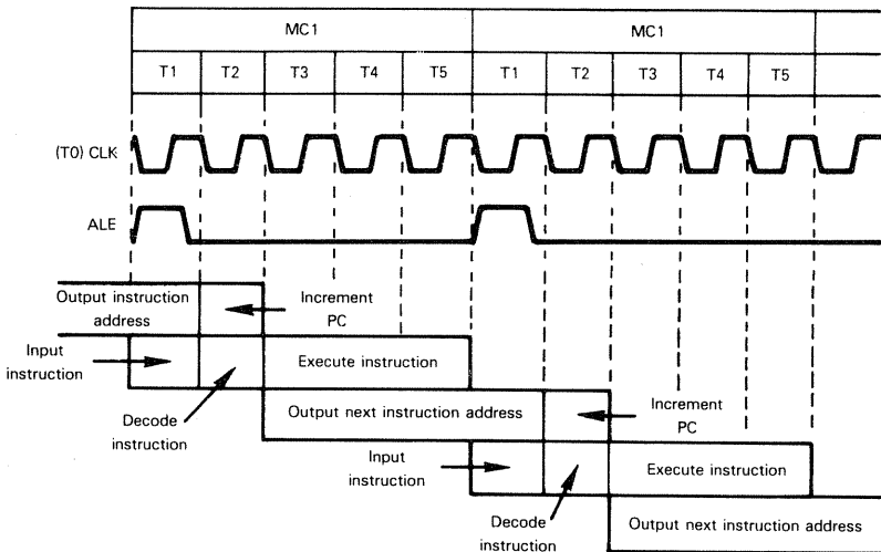
Figure 6-6 Execution Of 8048 Single Machine Cycle Instructions Without Any External Access
