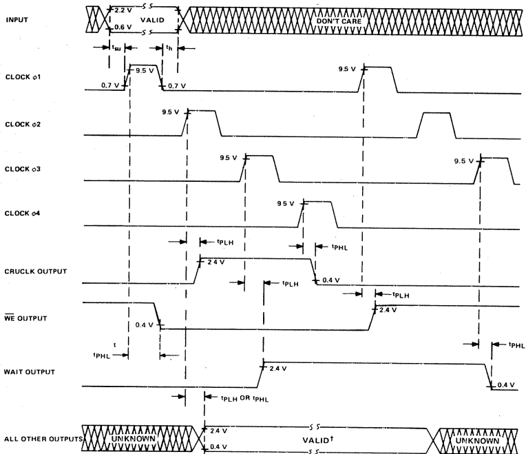
FIGURE 13—SIGNAL TIMING
