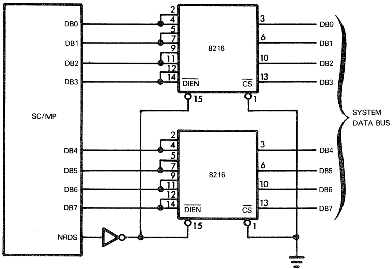
Figure 3-14. SC/MP Data Lines Buffered Using 8216 Devices
