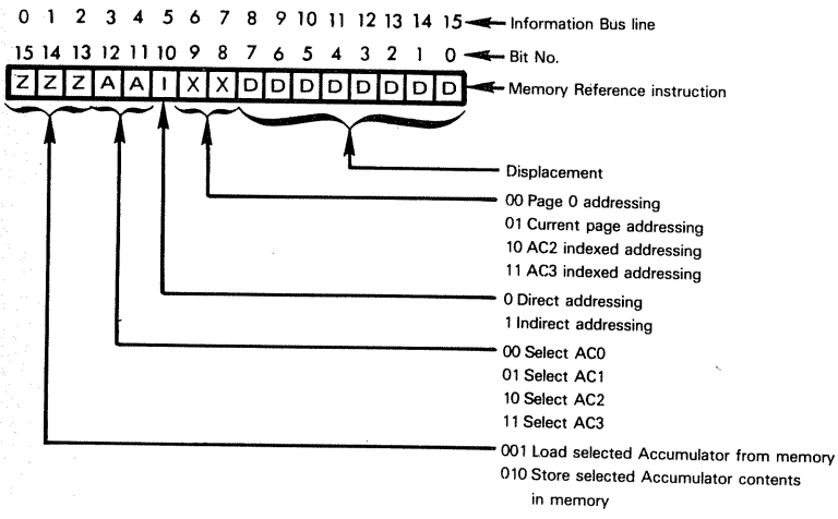
Figure 17-6 Load And Store Instruction Object Codes
