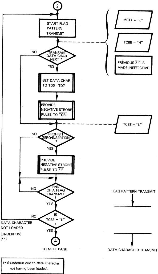
Figure 4-41. SDLC Transmit Operations Flow Chart
