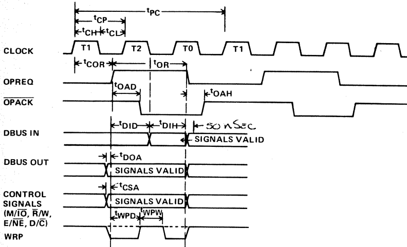
GENERAL TIMING
