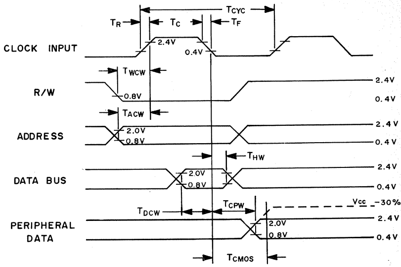
WRITE TIMING CHARACTERISTICS
