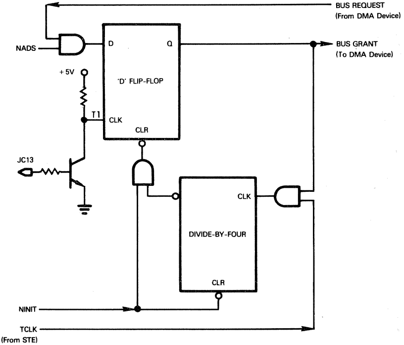
Figure 14-11. Idealized Circuit For Cycle-Stealing DMA During PACE Internal Machine Cycles
