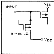
TYPICAL OF ALL K INPUTS
