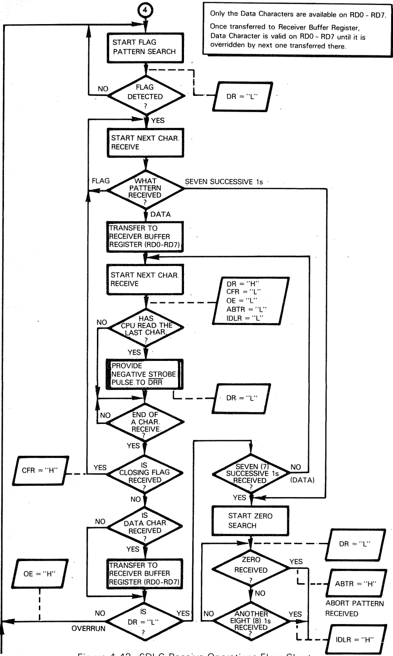
Figure 4-42. SDLC Receive Operations Flow Chart.
