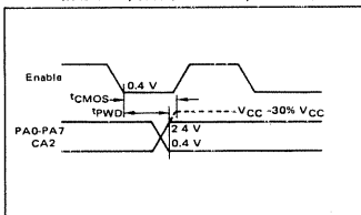
FIGURE 4 - PERIPHERAL CMOS DATA DELAY TIMES (Write Mode; CRA-5 = CRA-3 = 1, CRA-4 = 0)
