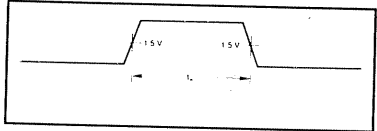
Data Delay Times
