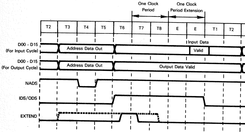
Figure 14-6. Using PACE EXTEND Signal To Lengthen I/O Cycles
