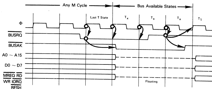
Figure 7-11. Z80 Bus Timing
