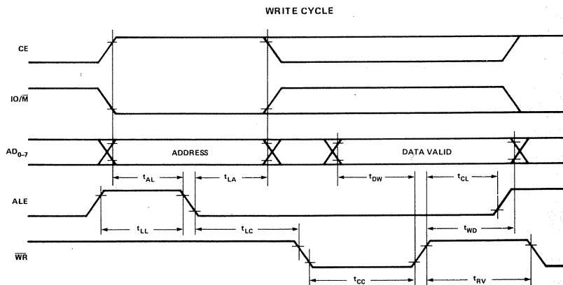
8155 READ/WRITE TIMING DIAGRAM.
