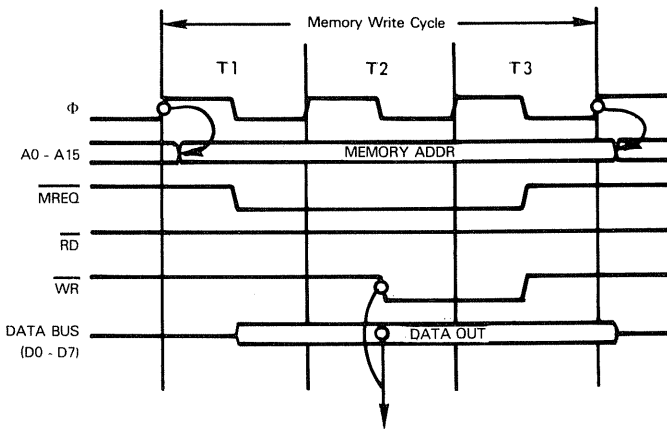
Figure 7-7. Z80 Memory Write Timing
