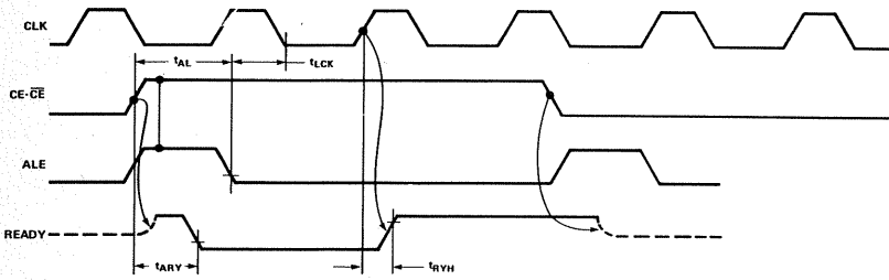
WAIT STATE TIMING (READY = 0).
