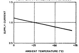
TYPICAL SUPPLY CURRENT VS. TEMPERATURE, NORMALIZED. [3]
