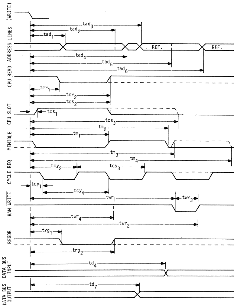
Timing Characteristics for 3852 DMI Output Signals
