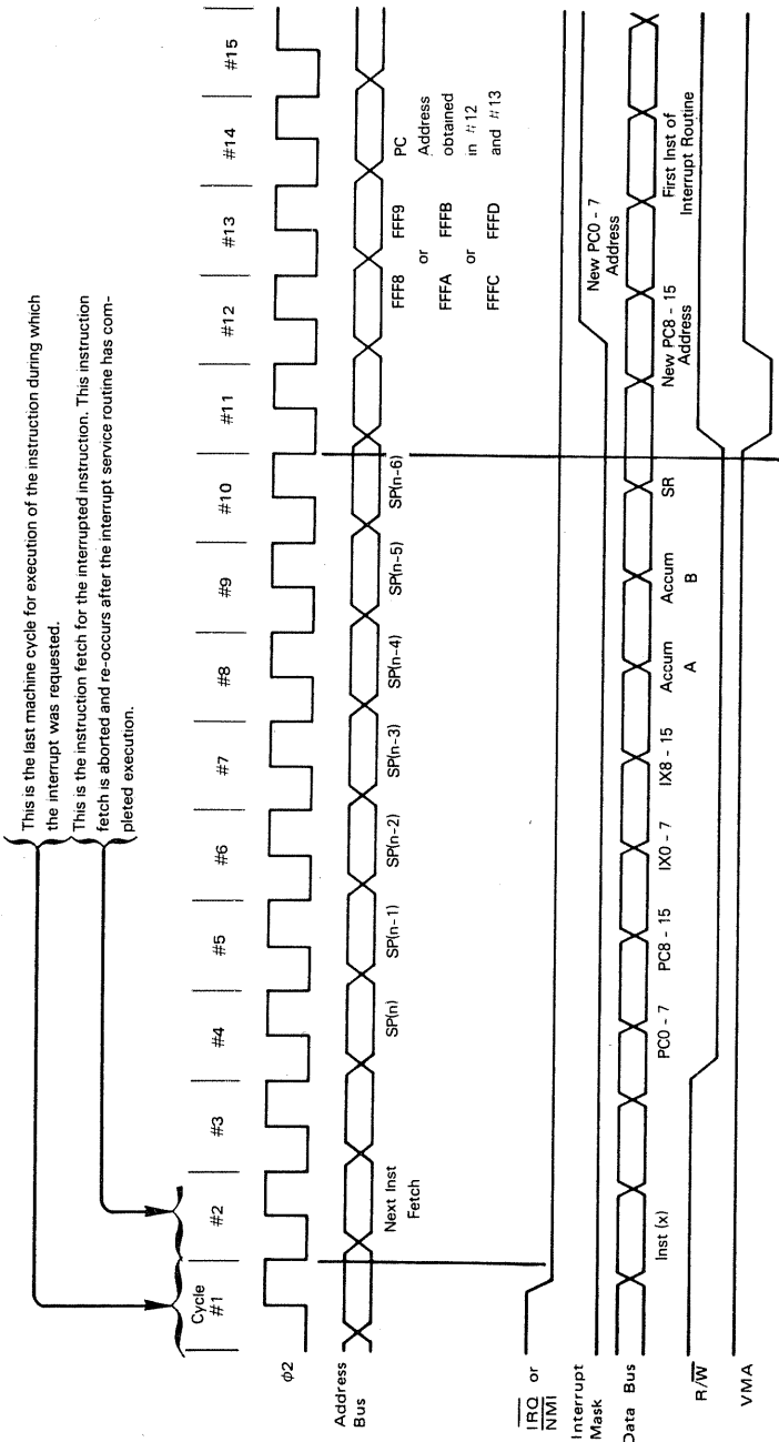
Figure 8-8. MC6800 Interrupt Acknowledge Sequence
