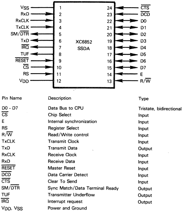
Figure 8-26 XC6852 SSDA Signals And Pin Assignments
