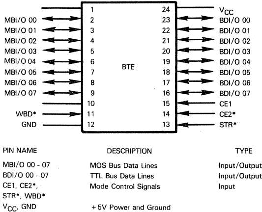
Figure 14-18 BTE Signals And Pin Assignments
