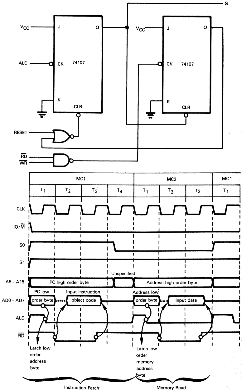
Figure 5-6 A Memory Read Machine Cycle Following An Instruction Fetch
