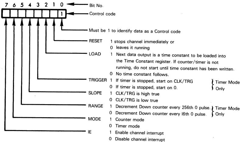
Figure 7-23 Z80 CTC Control Code Interpretation
