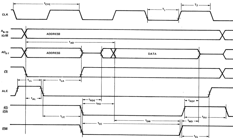
ROM READ AND I/O READ AND WRITE.
