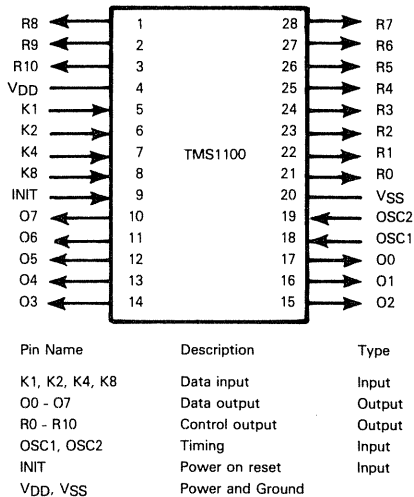
Figure 1-6. TMS1100 Microcomputer Signals And Pin Assignments
