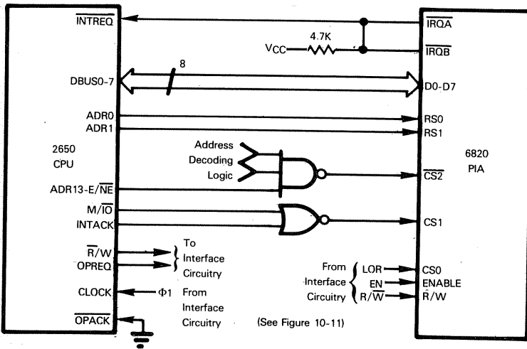
Figure 10-13 An MC6820 PIA Connected To A 2650
