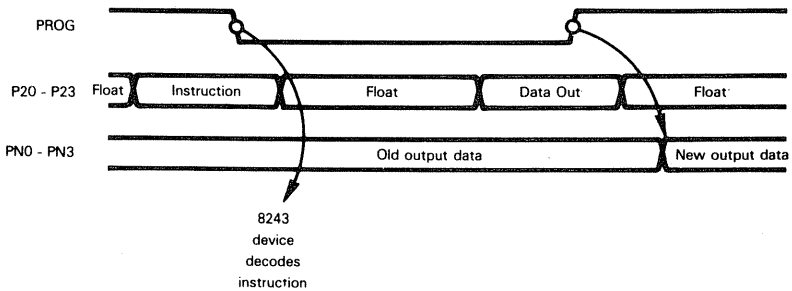
Figure 6-19 Timing For Data Output To An 8243 Port Via A MOV, ORLD Or ANLD Instruction
