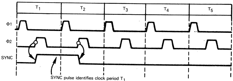
Figure 4-3. A Machine Cycle Consisting Of Five Clock Periods
