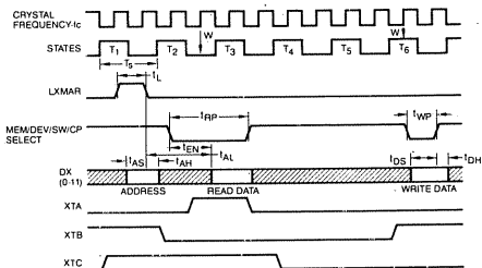
IM6100 TIMING AND STATE SIGNALS
