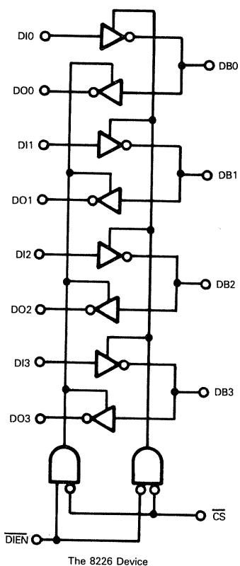
Figure 4-62. Bidirectional Bus Drivers
