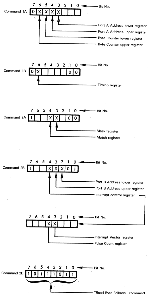
Figure 7-26. A Summary Of Z80 DMA Writable Register Locations
