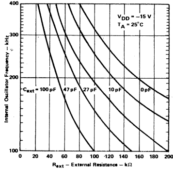
TYPICAL INTERNAL OSCILLATOR FREQUENCY vs EXTERNAL RESISTANCE
