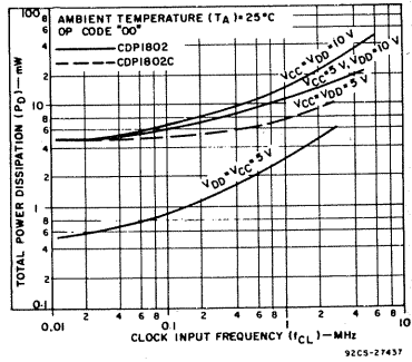
Typical total power dissipation vs. clock input frequency.
