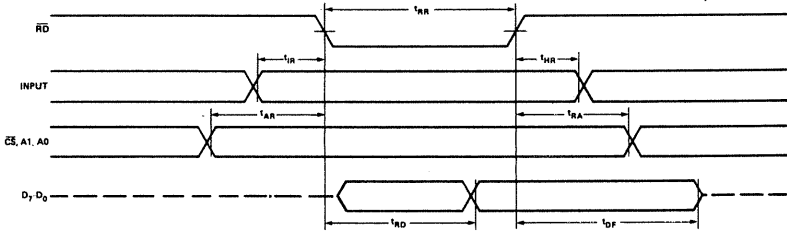
Mode 0 (Basic Input)
