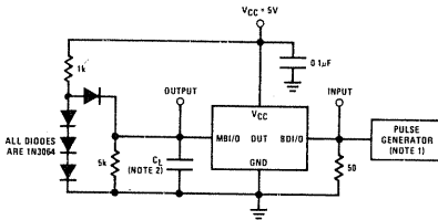
FIGURE 6. BDI/O to MBI/O ac Loads
