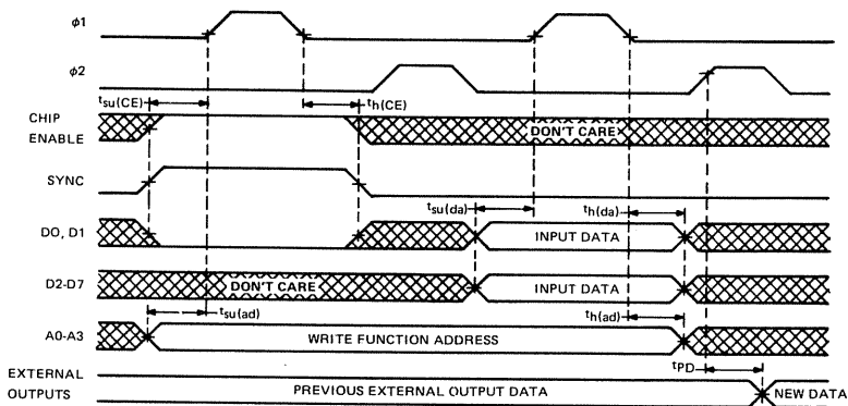
FIGURE 7—WRITE CYCLE TIMING
