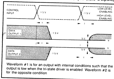
Output Enable and Disable Times (Tri-state Outputs)
