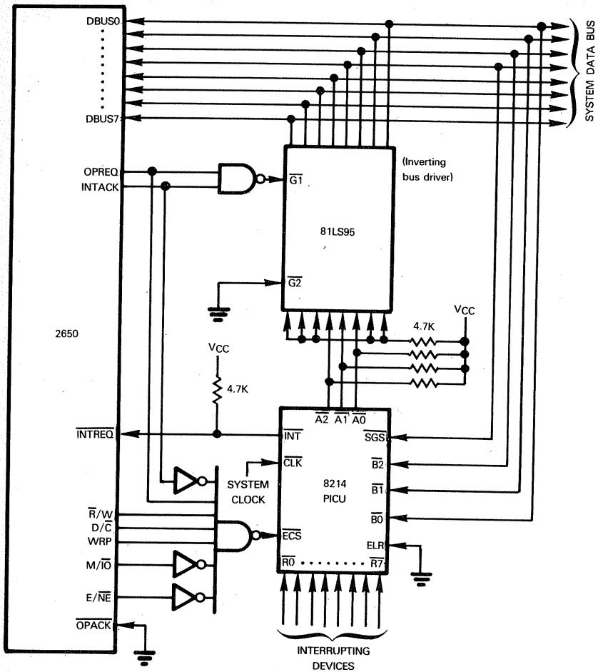
Figure 10-10. Vectored Interrupt Using The 8214 PICU With A 2650 CPU
