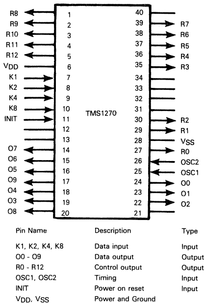
Figure 1-5. TMS1270 Microcomputer Signals And Pin Assignments
