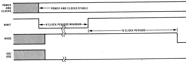
FIGURE 6. Initialization Timing
