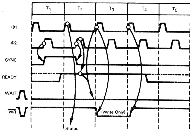
Figure 4-7. The 8080A CPU Operating With Fast Memory And No Wait State
