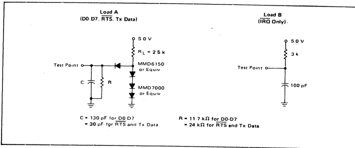
FIGURE 9 - BUS TIMING TEST LOADS
