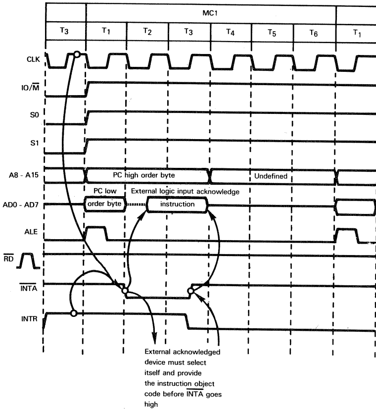
Figure 5-16. An Interrupt Being Acknowledged Using A Single Byte Instruction
