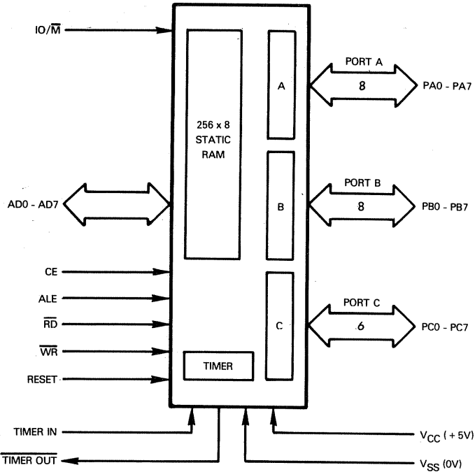
Figure 5-20. Logic Functions Of The 8155 Device
