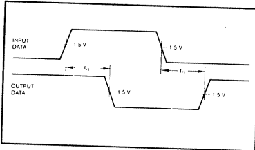
Setup and Hold Times
