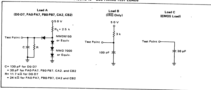
FIGURE 12 -- BUS TIMING TEST LOADS
