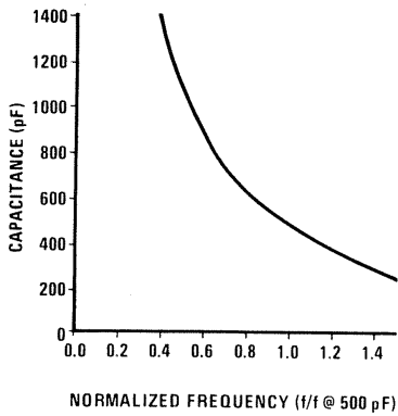
Oscillator Frequency versus Capacitance
