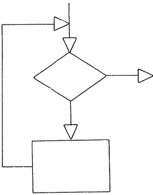
DO WHILE
