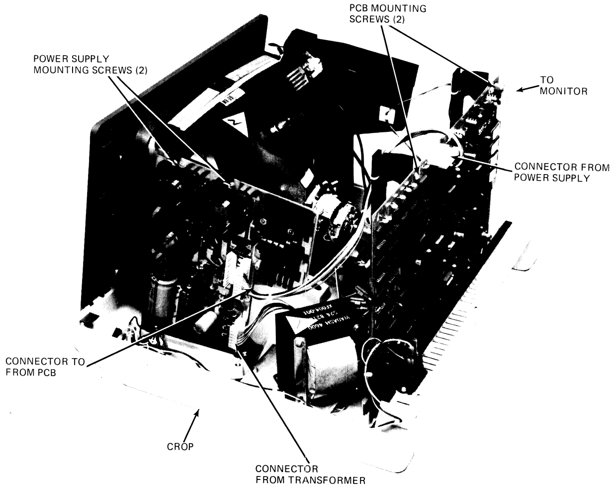
Figure 7-2. PCB Mounting
