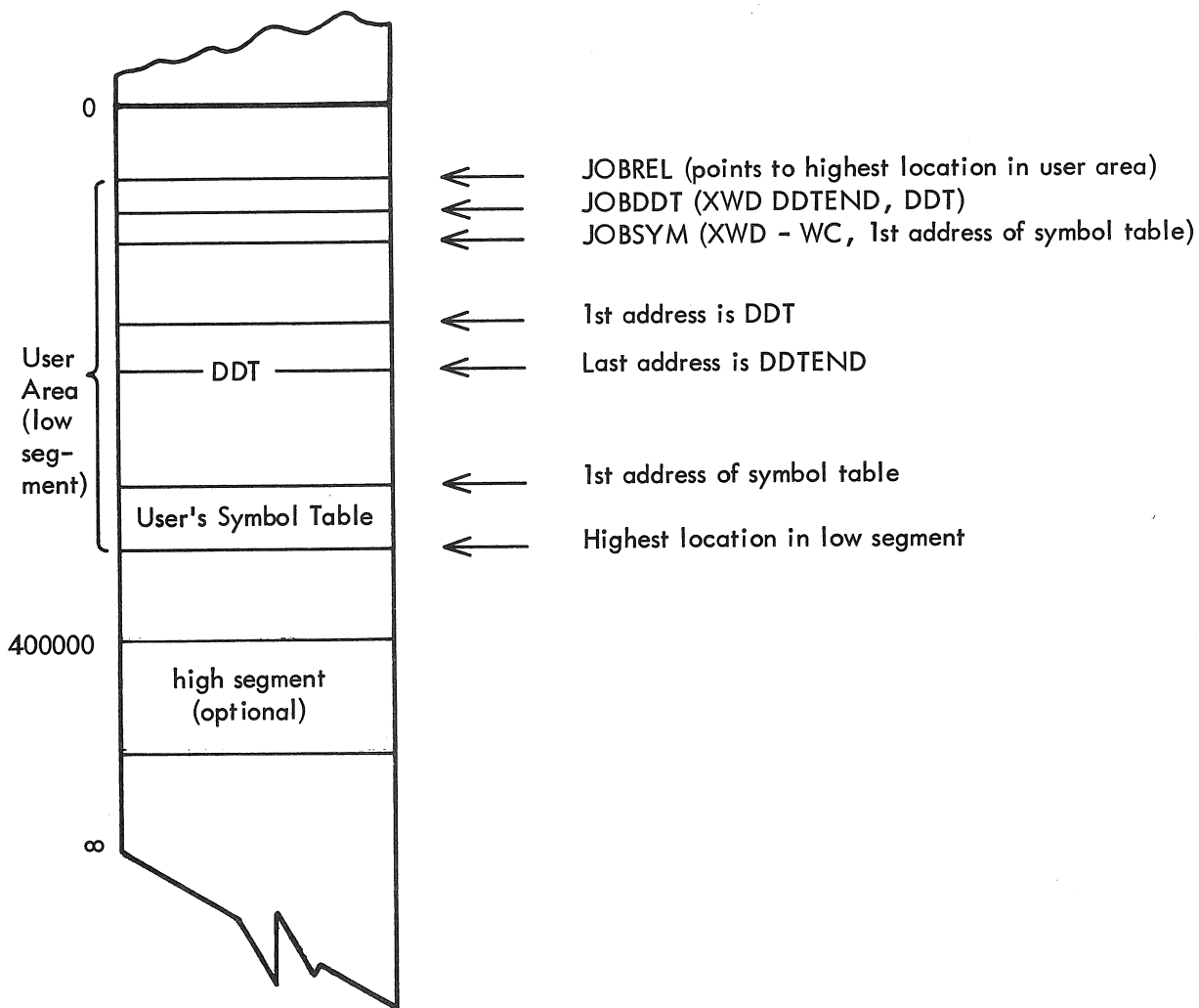
Figure B-1 Storage Map for User Mode DDT
