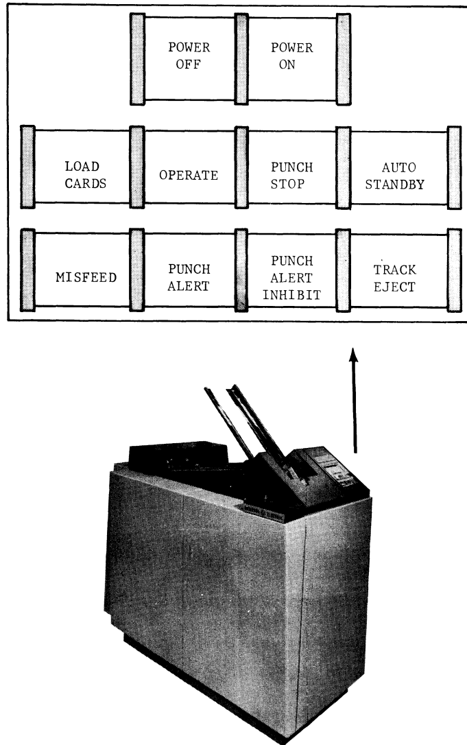
Figure 42. 300 cpm Card Punch Control and Indicator Panel
