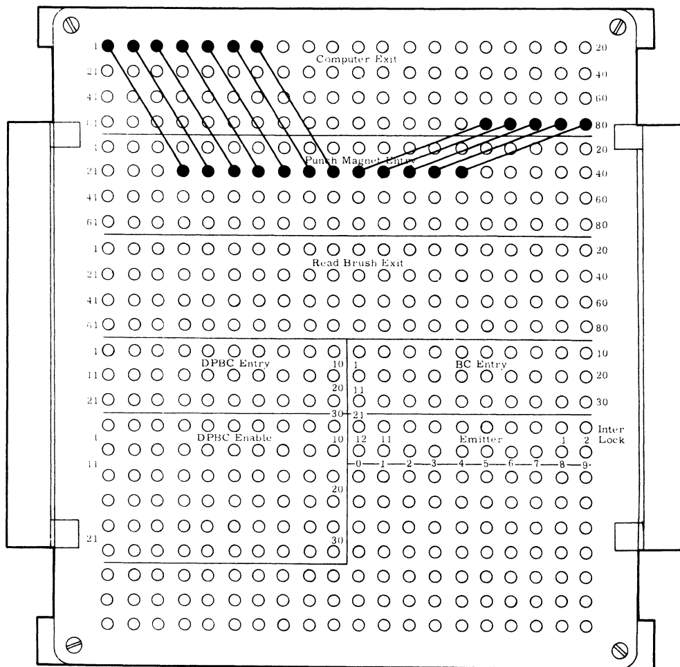
Figure 38. Plugboard Wiring for Relocation of Central Processor Information
