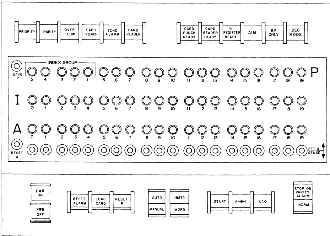
Figure 20. GE-225/GE-215 Operator's Console
