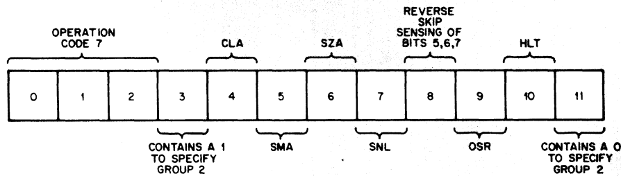
Figure 7 Group 2 Operate Instruction Bit Assignments
