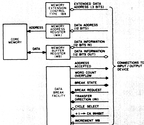
Figure 34 Data Break Transfer Interface Block Diagram
