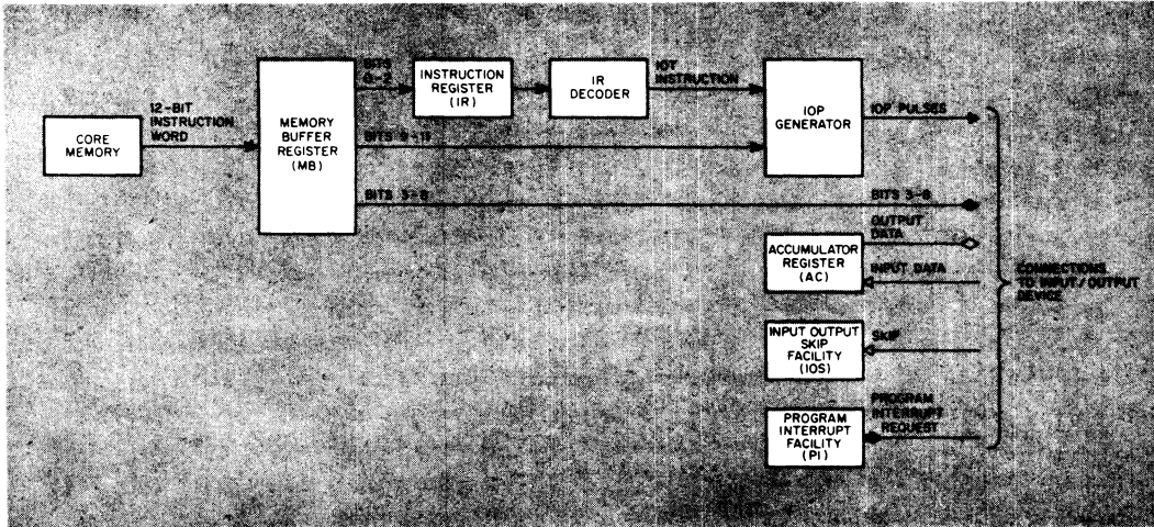
Figure 21 Programmed Data Transfer Interface Block Diagram
