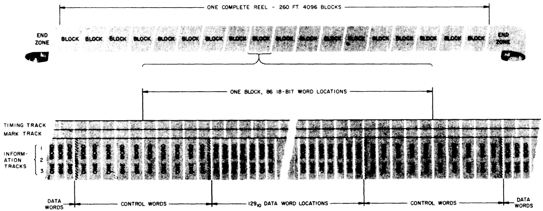
Figure 11 DECTape Control Word and Data Word Assignments
