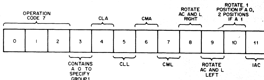
Figure 6 Group 1 Operate Instruction Bit Assignments
