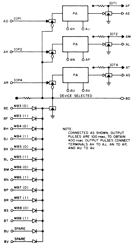
Figure 55 Device Selector W103 Logic Circuit
