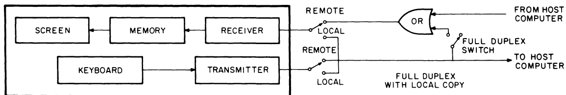
Figure 4-1 Interface Modes
