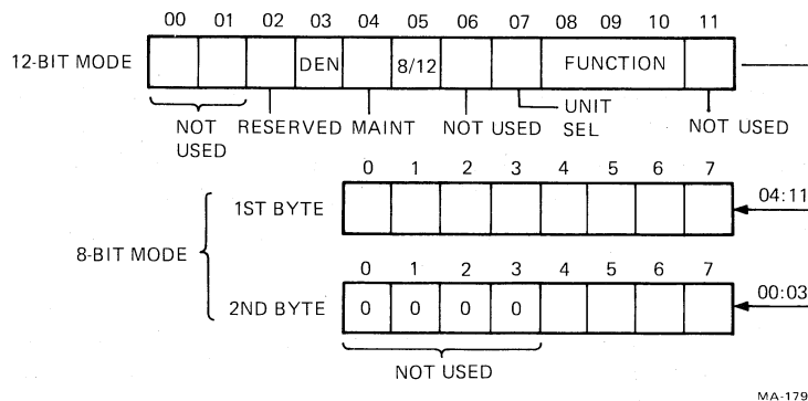
Figure 4-4 Command Register Format (RX28)
