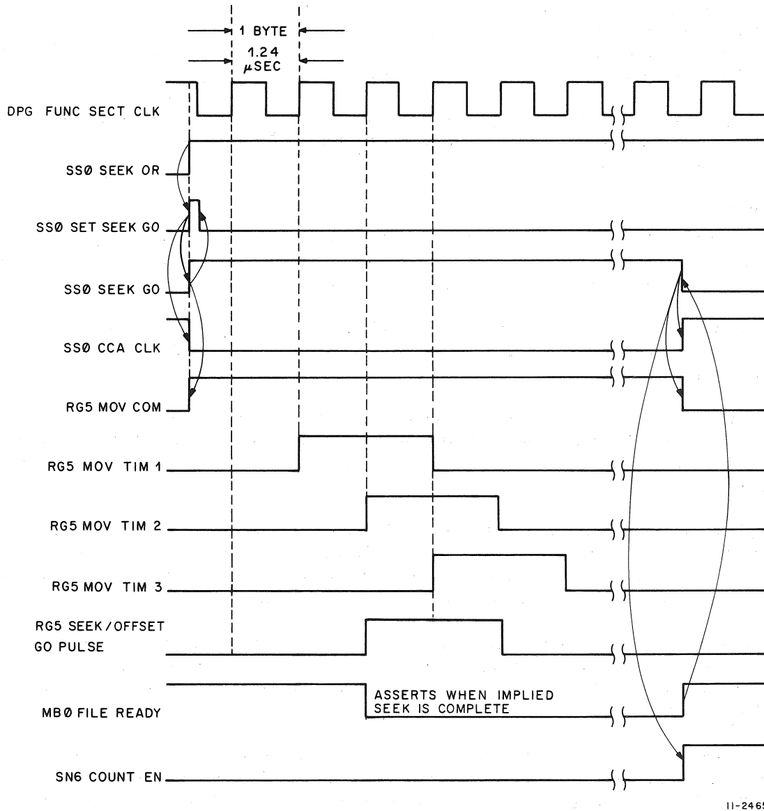
Figure 3-2 Implied Seek Timing Diagram
