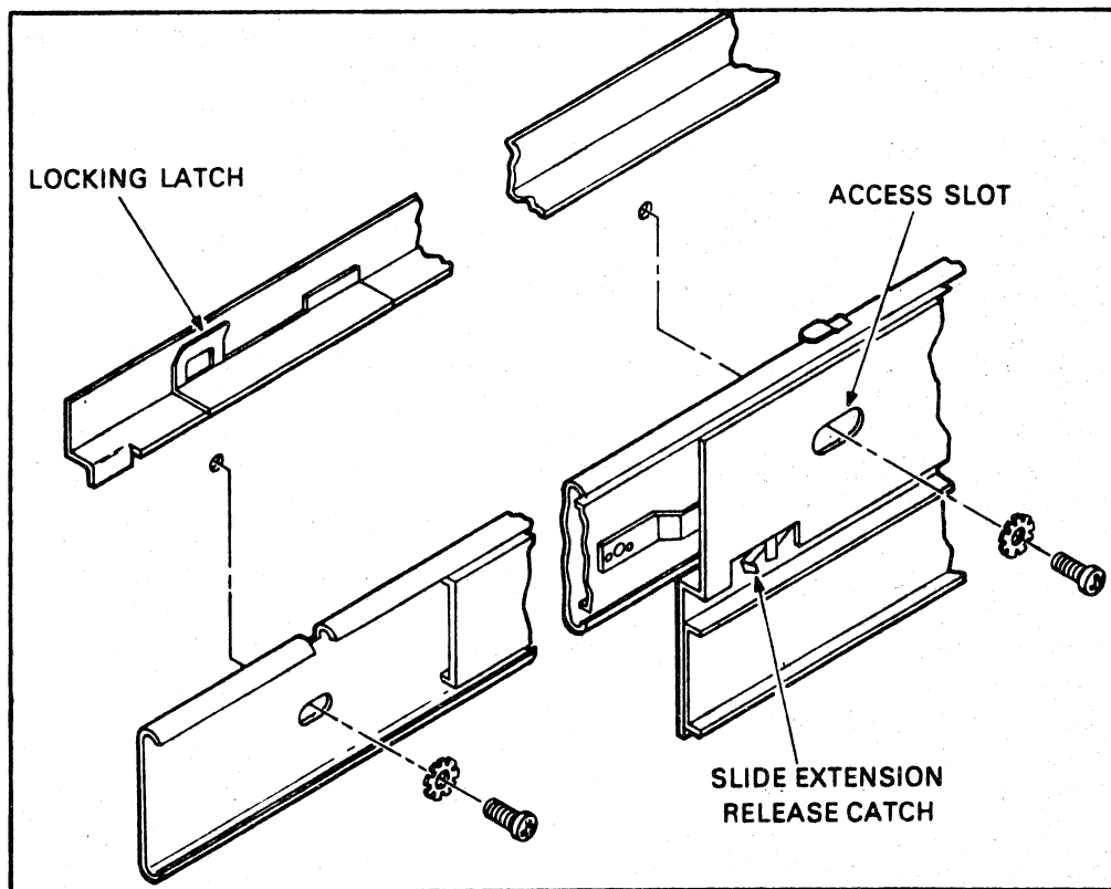
Figure 2-6 Slide Rails
