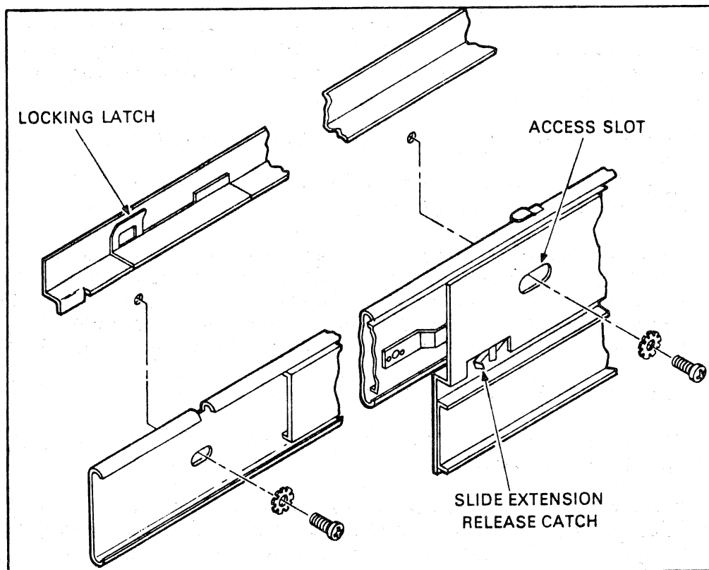
Figure B-20 RL01/RL02 Cabinet Installation
