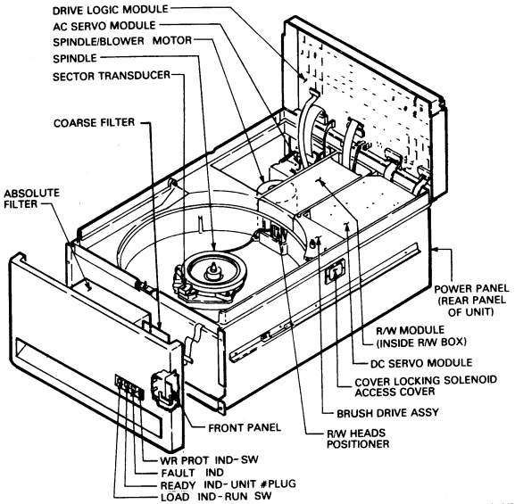
Figure 2-7 Physical Location of FRUs
