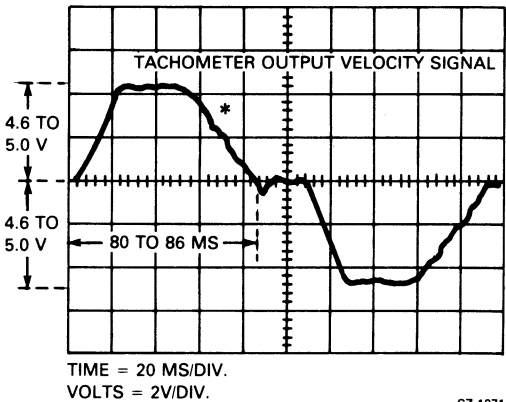
Figure 9-10 Tachometer Output Velocity Signal
