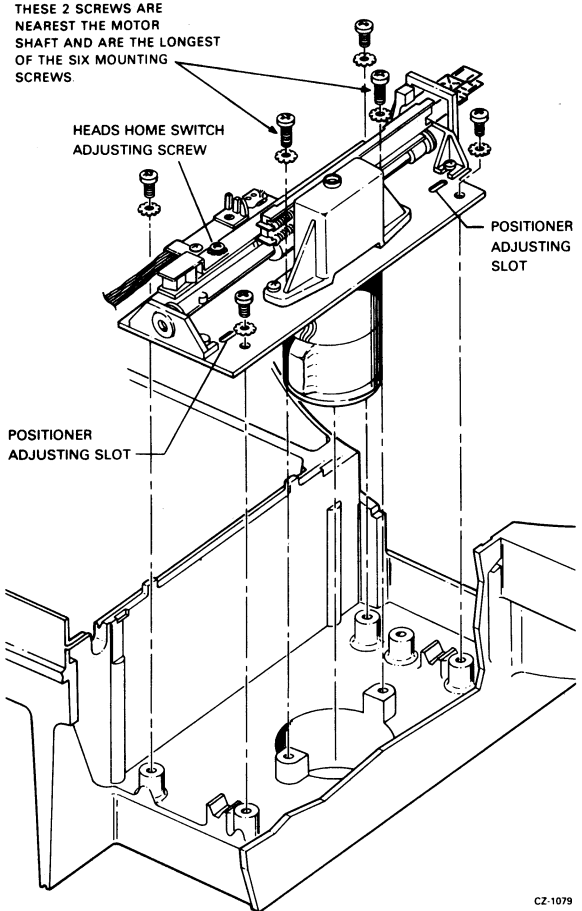
Figure 9-5 Positioner Assembly
