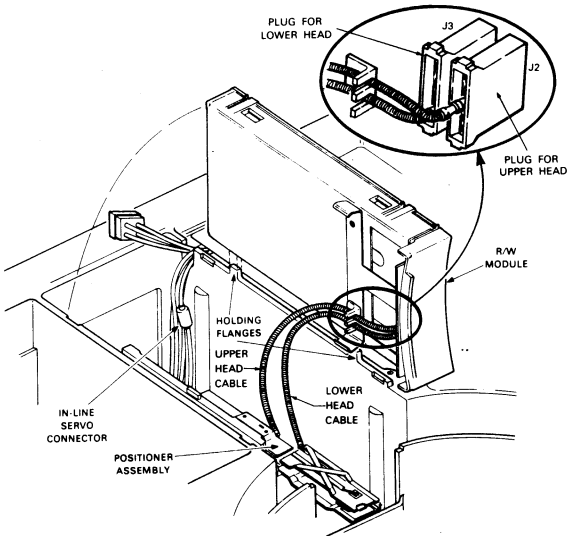
Figure 9-3 Positioner and Read/Write Module Box Assembly
