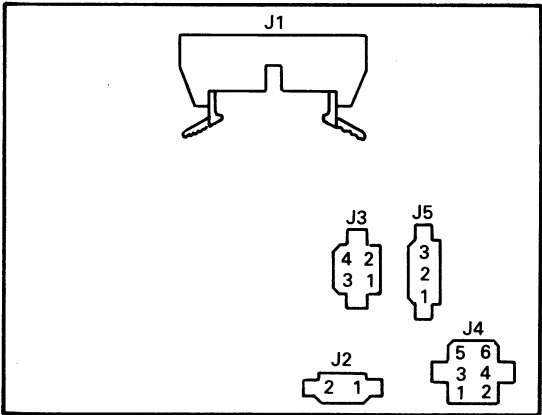
Figure 2-13 AC Servo Module Layout — Front View
