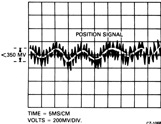
Figure 9-7 Position Signal
