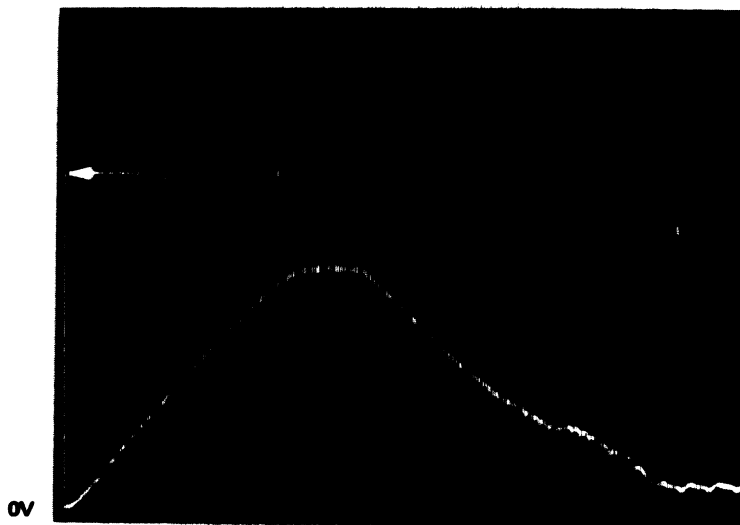
Figure 6-6 Acceleration Waveform
