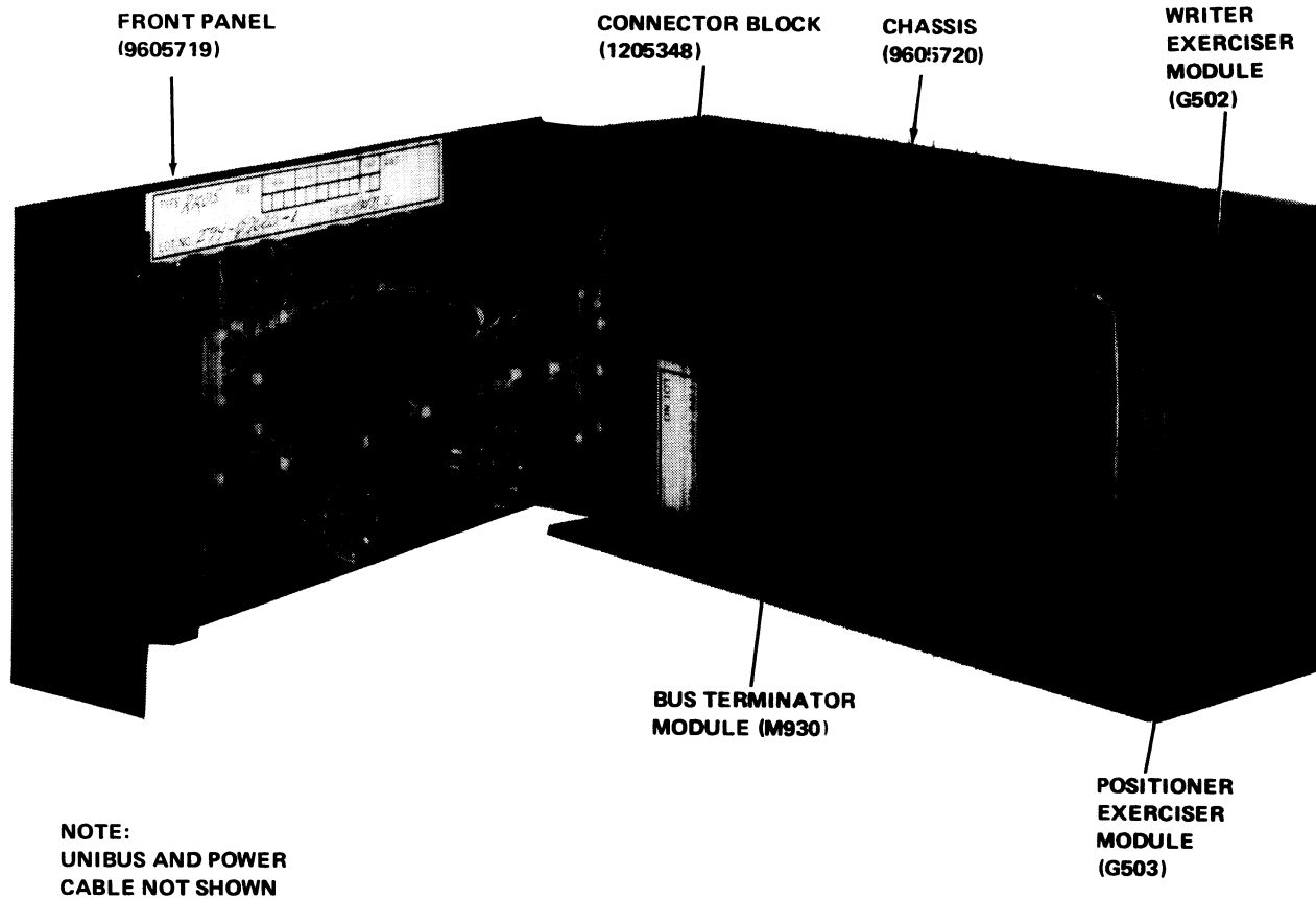
Figure 1-1 RK05 Exerciser Components
