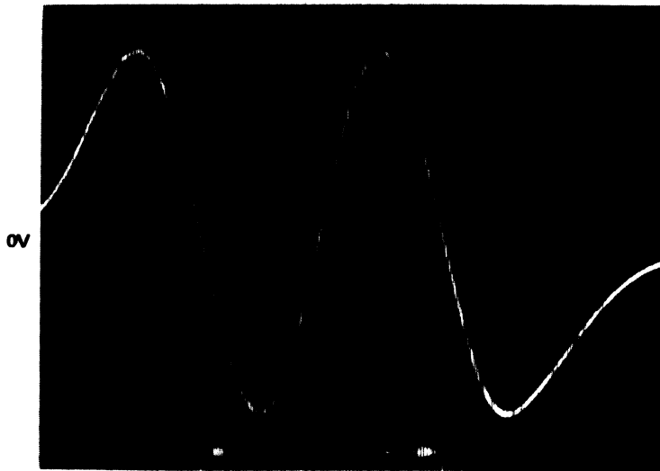
Figure 6-5 Velocity Amplitude Waveform
