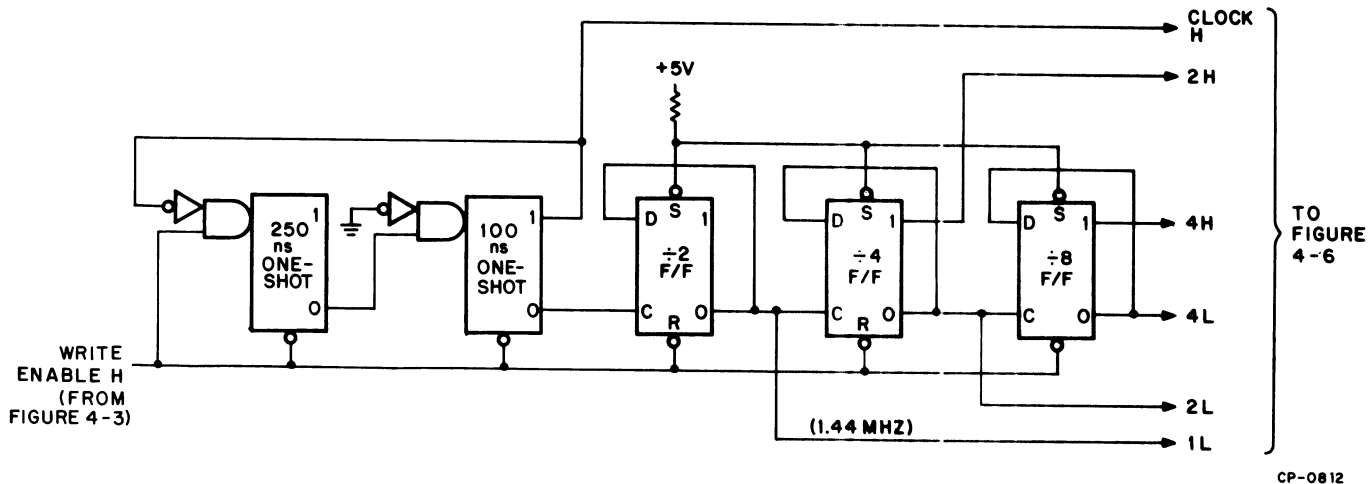
Figure 4-4 Write Clock
