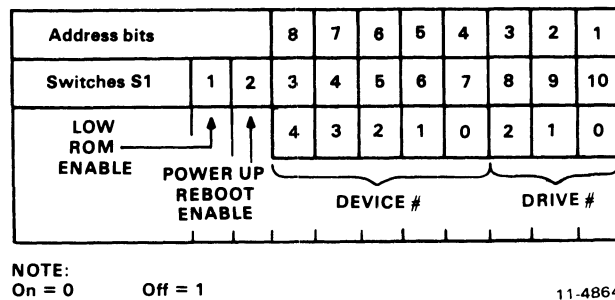
Figure 9-2 Microswitch Assignment
