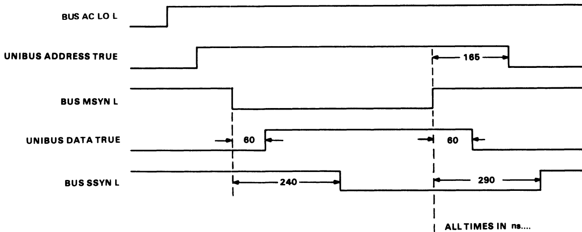
Figure 1-2 M9301 Timing
