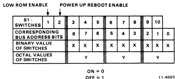
Figure 11-2 Offset Switches and Corresponding Bus Address Bits
