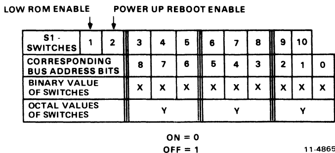
Figure 7-2 Offset Switches and Corresponding Bus Address Bits
