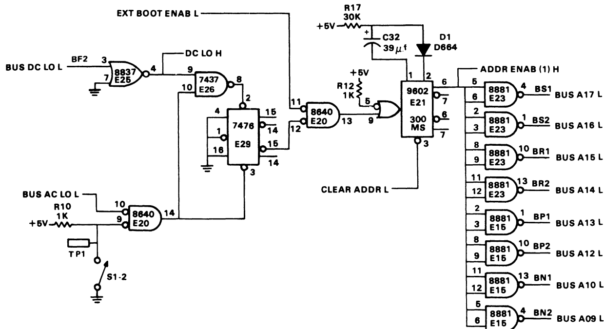
Figure 2-2 Power-Up Boot Logic
