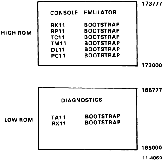
Figure 7-1 Program Memory Map for the M9301-YA
