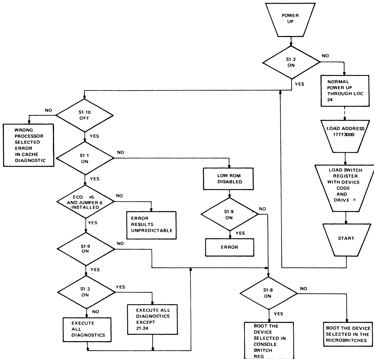
Figure 13-3 M9301-YH Used with PDP-11/70
