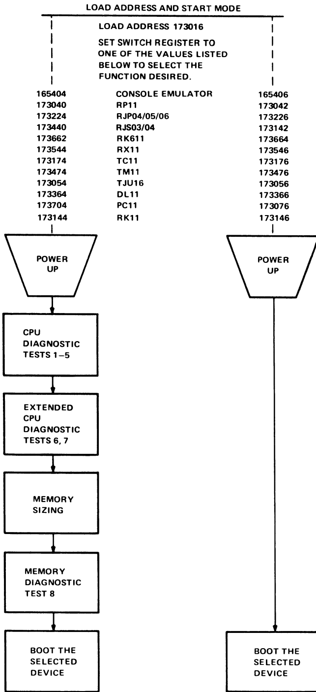
Figure 12-4 M9301-YF Load Address and Start Mode Flowchart
