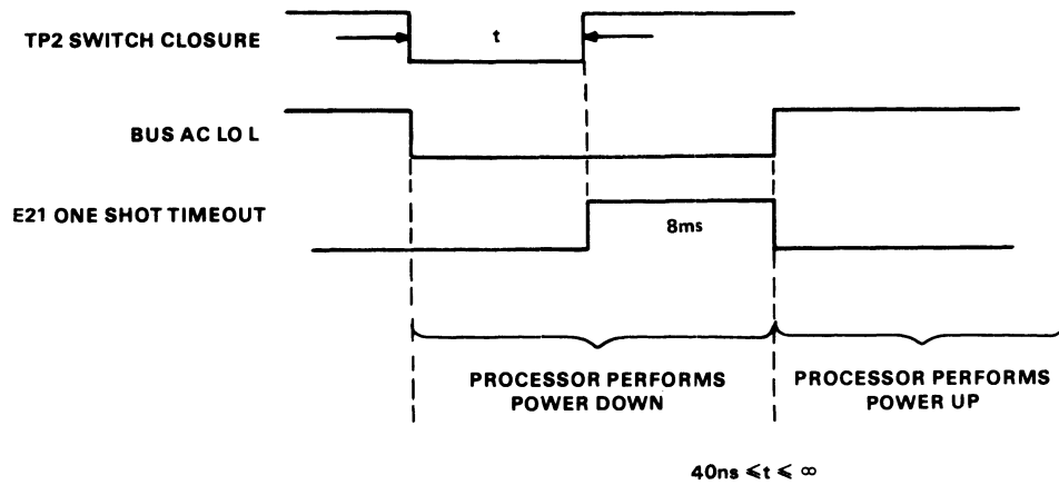
Figure 2-4 External Boot Timing
