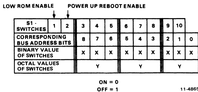
Figure 1-3 Offset Switches and Corresponding Bus Address Bits
