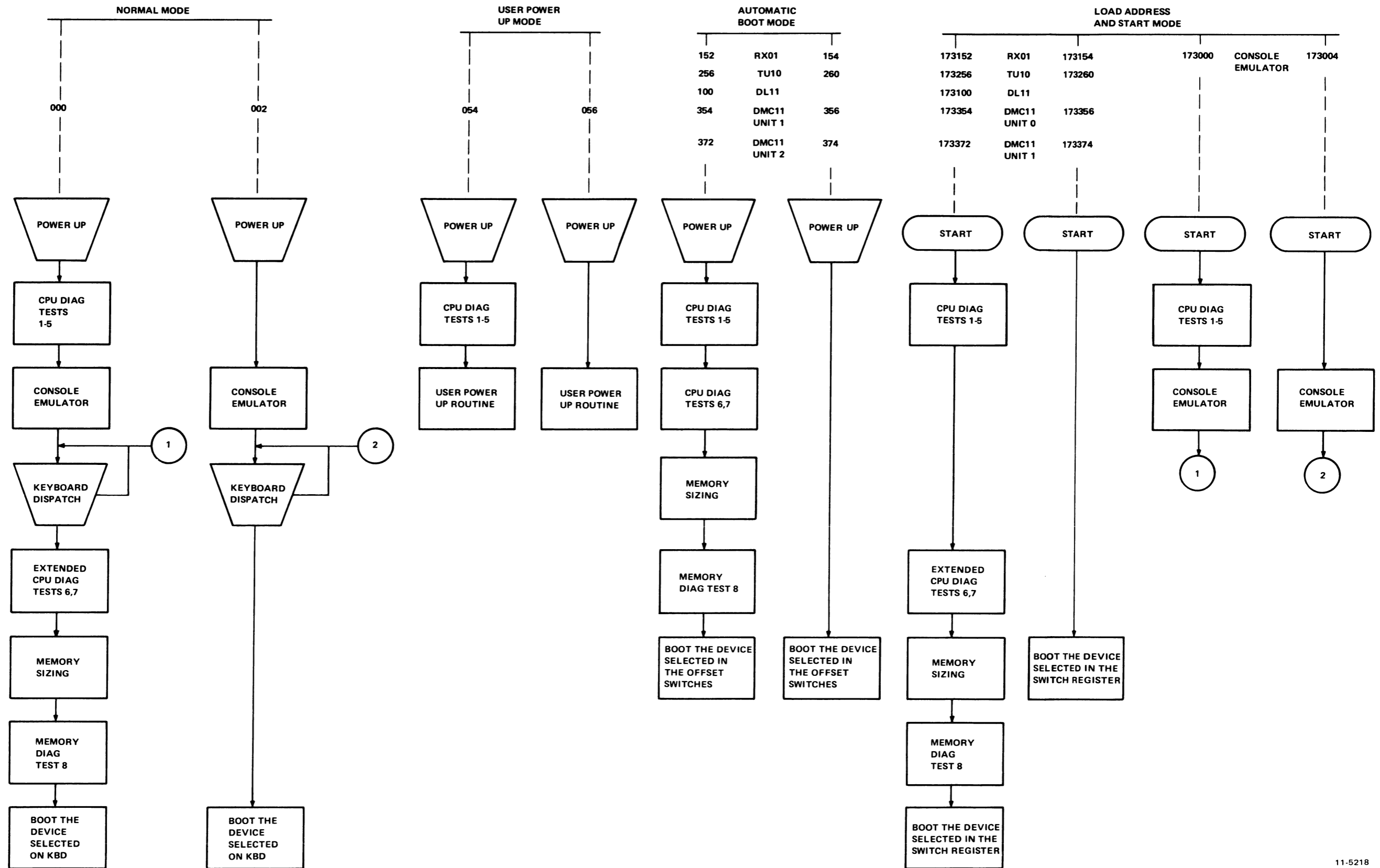
Figure 14-4 M9301-YJ Operator's Flowchart
