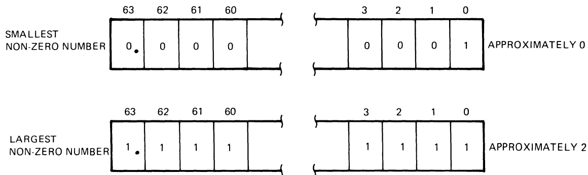
Figure 4-5 Unnormalized Floating-Point Fraction
