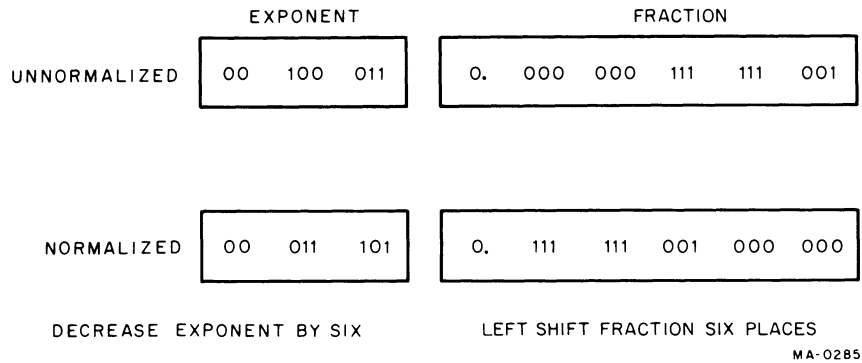
Figure 3-1 Normalization
