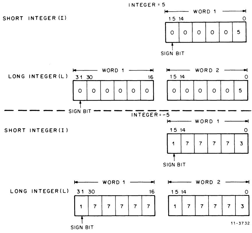
Figure 4-1 Integer Formats
