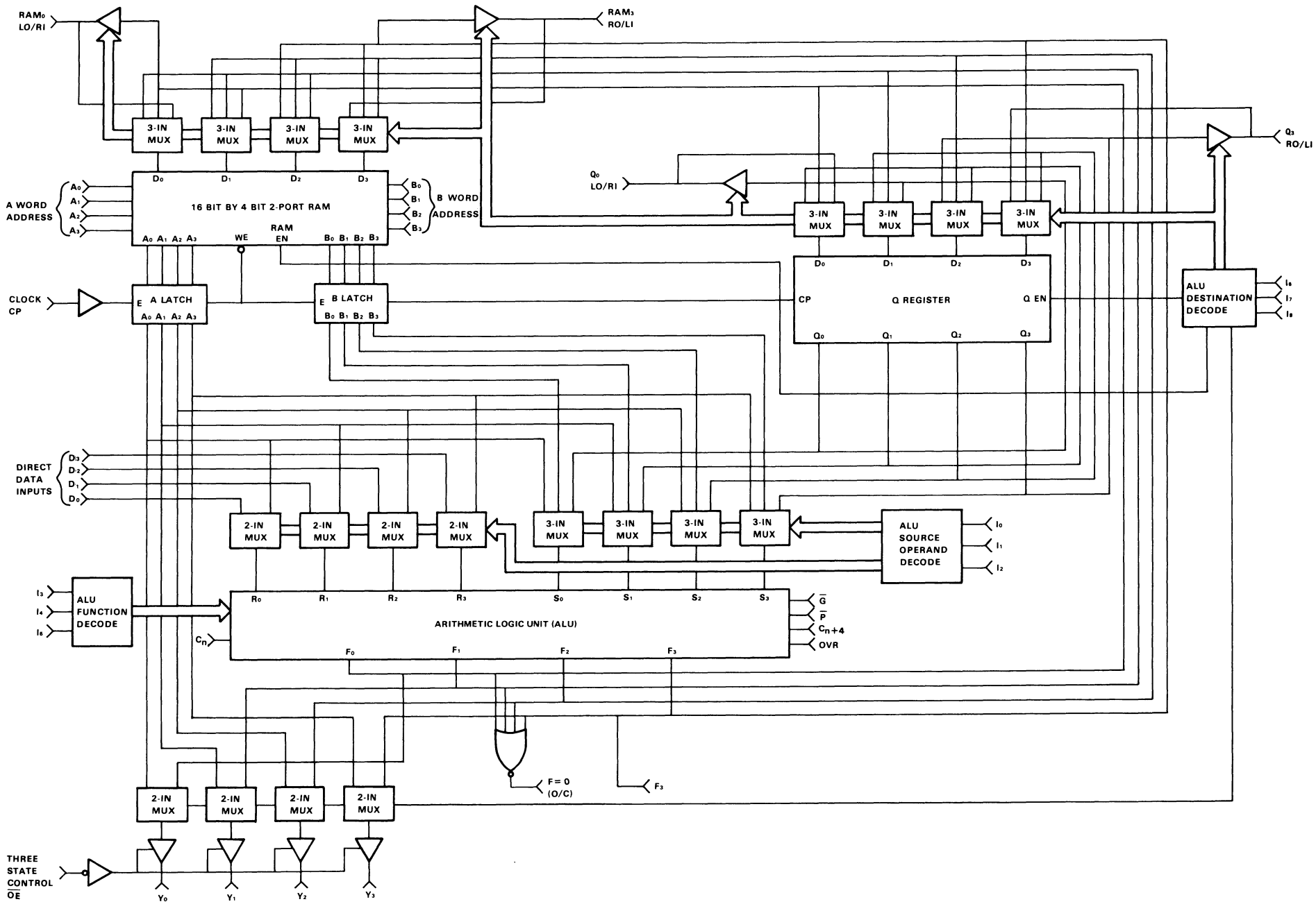
Figure 6-3 Microprocessor (AM2901) Block Diagram
