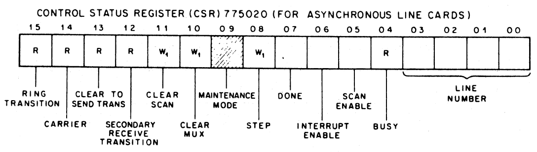
Figure 3-3 DV11 Primary Registers (Sheet 2 of 3)
