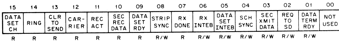
Figure 3-1 Receiver Status Register (RXCSR)
