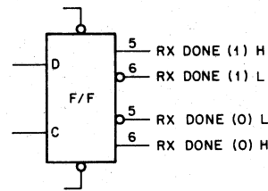
Figure 1-5 Flip-Flop Signal Names
