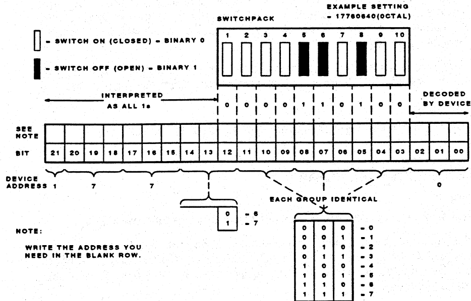
Figure 2-6 CSR Address Switch Setting Guide
