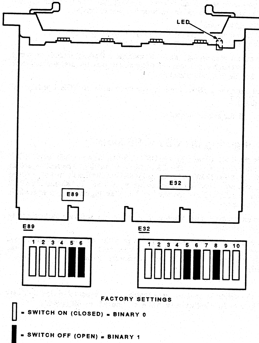
Figure 2-5 DSV11-SF Module Layout
